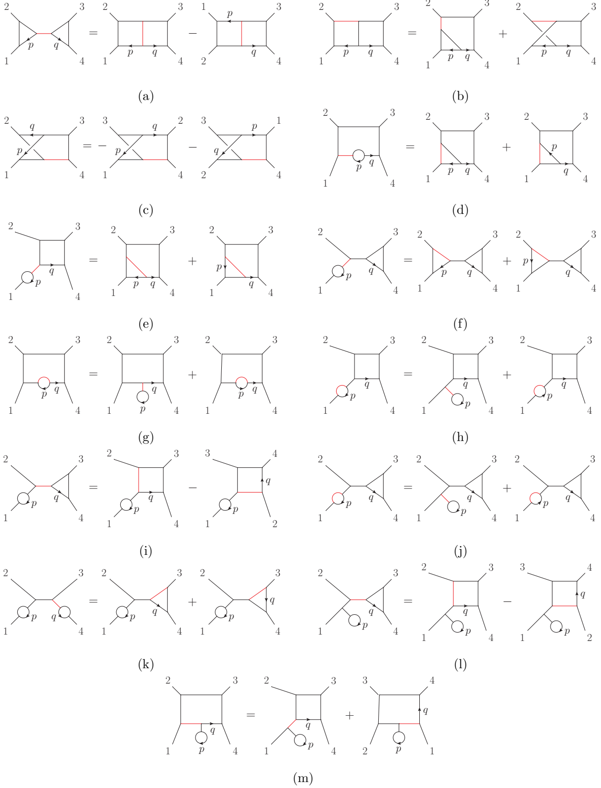
FIG. 8: The nontrivial duality relations (a)-(m) satisfied by the numerators of the identical-helicity two-loop amplitude. The shaded (red) leg marks the central leg of the applied Jacobi identity.
