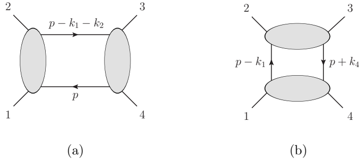
FIG. 5: The (a) s -channel and (b) t -channel unitarity cuts used to determine the amplitude. The exposed intermediate legs are on shell.
