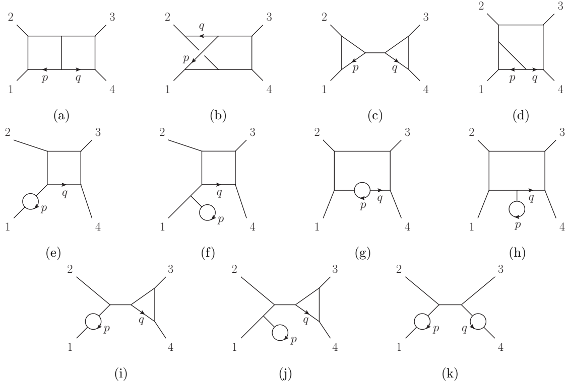
FIG. 6: The diagrams needed to describe an integrand for the identical helicity-amplitude where the duality between color and kinematics is manifest. When integrated all diagrams, except the (a) planar double-box, (b) nonplanar double-box, and (c) double-triangle integrals, vanish.
