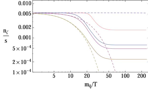
FIG. 6. Evolution of the goldstino number density for non-negligible m_\zeta . Here we have fixed m_{\bar{q}} = 1 TeV, F_\zeta = (100 \text{ TeV})^2 and T_R = 40 GeV. From top to bottom, the continuous lines are the yield computed assuming kinetic equilibrium in the massless case, and the yields using the full Boltzmann equation, for three different values of the masses, m_\zeta = 0 GeV, 100 GeV, 200 GeV. The dashed lines are equilibrium number densities for the same masses.
