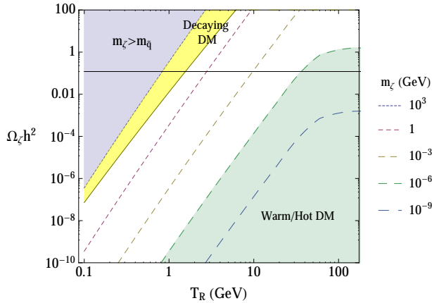
FIG. 4. Late-time energy density of goldstinos, with small F -term F_\zeta = (100 \text{ TeV})^2 and m_{\bar{q}} = 1 \text{ TeV} , for different values of the goldstino mass. For m_\zeta < 1 \text{ keV} the goldstino is warm or hot dark matter. For m_\zeta in the range 100 \text{ GeV} - 1 \text{ TeV} (yellow region) the goldstino lifetime, Eq. (27), is too short, \tau \lesssim 10^{26} \text{ sec} , and is excluded by DM indirect detection constraints. The horizontal black line marks the observed value of the DM abundance, \Omega_{DM} h^2 = 0.12 .
