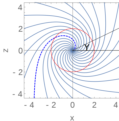
FIG. 14: Example congruence of geodesics in the equatorial plane of the Schwarzschild black hole, with a non-vanishing impact parameter b translating into \mathcal{P} = 2/27M^2 (not the value we use for the simulations, but instead chosen to accentuate the perturbation). The red circle is the location of the event horizon. Angle Y is the angle at which the dashed geodesic strikes the origin.
