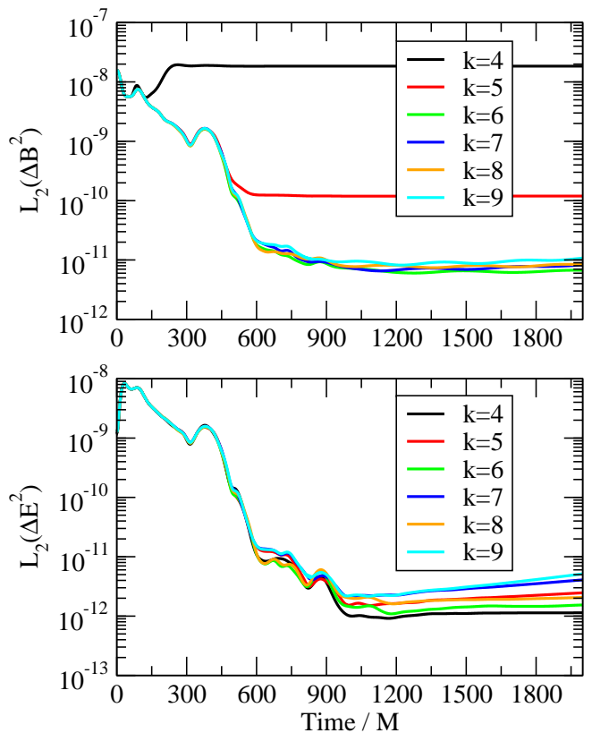
FIG. 16: Top: The L_2 norm of the difference measure \Delta B^2 for the \text{null}^+ simulations initially perturbed in the propagation direction. Bottom: The L_2 norm of the difference measure \Delta E^2 .
