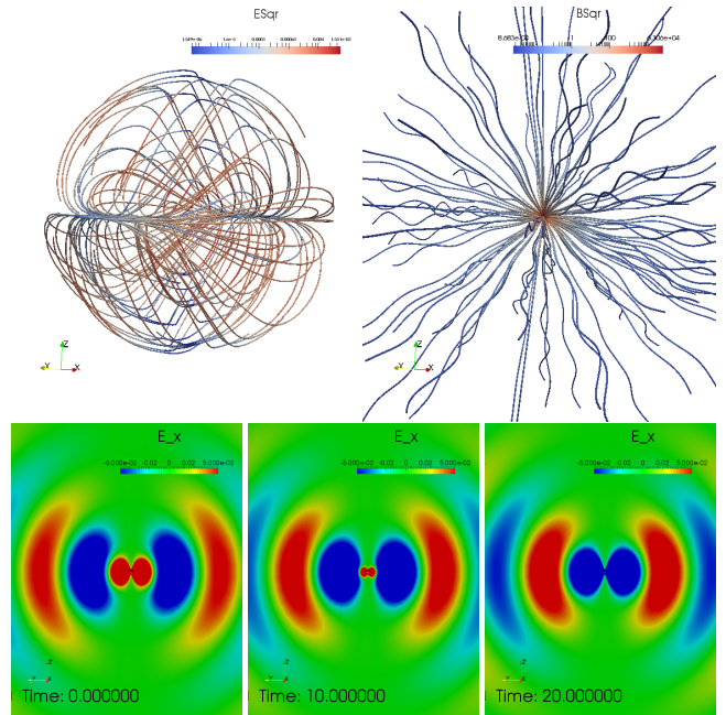
FIG. 2: Top left figure shows the electric field lines, and the top right figure shows the magnetic field lines for the same \text{null}^+ solution as shown in Fig. 1, the lines are coloured by E^2 and B^2 respectively. The bottom figures plot the time variation of the E_x component, showing the wave propagating inwards.
