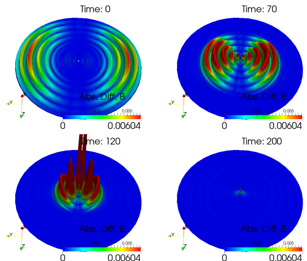
FIG. 20: The absolute difference |\Delta \mathbf{B}| on a vertical slice of the computational domain. The initial perturbation seen at t = 0 propagates inwards creating the patterns seen at t = 70 and t = 120 . By t = 200 , the perturbation has been almost entirely absorbed by the black hole. We have shown the absolute, rather than the relative difference, because |\mathbf{B}| increases quickly when we approach the black hole, so it is more difficult to see what is going on in the inner regions with a relative difference plot.
