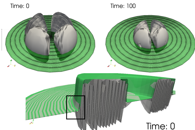
FIG. 6: Top row: Contours of \Re\phi_0 that shows the structure of the wave train. It has a Y^{2,2} angular profile, and consists of fast radial oscillations with frequency \Omega . It is confined into a radial tophat style envelope of width 200M . The shape of the wave train shows that our test is fully three dimensional, without any axisymmetry. The figures on the left and right depict the wave train at earlier and later times, showing that it is initially moving inwards toward the black hole. The green semi-transparent surface is the equatorial slice of the computational domain, included to indicate its extend. The grid structure on this slice is also plotted to provide a visual description of the density of collocation points at K = 7 . Bottom figure: The \Re\phi_0 is depicted by warping half of the equatorial slice with a vertical displacement proportional to the \Re\phi_0 values at collocation points, and then connecting them via “straight lines” into the gray surface (i.e. the gray surface is a trivial interpolation between the collocation points and is not the actual \Re\phi_0 as represented by the spectral functions). The green surface is the tophat-like radial envelope function. This figure also corresponds to K = 7 .
