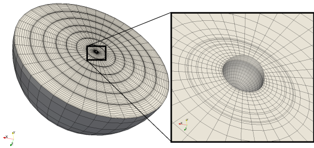
FIG. 3: Half of the computational domain and the spectral grid (spectral collocation points are at the intersection of the black lines), the semi-transparent sphere represents the event horizon of the Schwarzschild black hole.
