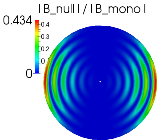
FIG. 1: The ratio |B_{\text{null}}|/|B_{\text{mono}}| for the \text{null}^+ solution studied, where \mathbf{B}_{\text{null}} and \mathbf{B}_{\text{mono}} are the null and monopole contributions in Eq. (33), while the norm is defined as |B_{\text{null}}| = \sqrt{\mathbf{B}_{\text{null}} \cdot \mathbf{B}_{\text{null}}} . Shown is a cross-section in the xz -plane, which extends radially from R_- = 1.95M to R_+ = 195M .
