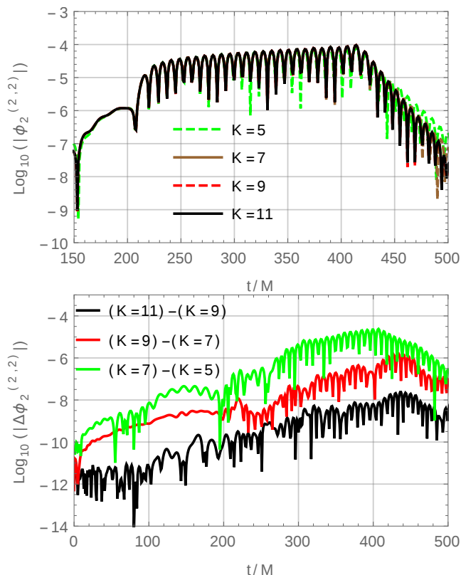
FIG. 9: Top figure shows the wave train and the QNM tail for the four resolutions of the \Omega = 0.4 simulation. The bottom figure shows the differences between resolutions. Because the differences are approximately equally displaced in the vertical direction, which is plotted in log scale, the simulation indeed achieves exponential convergence.
