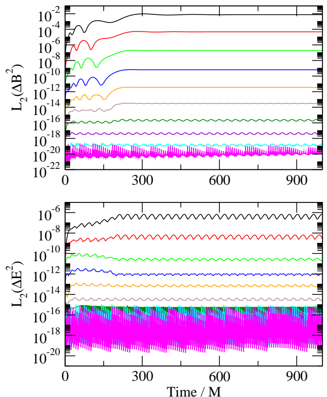
FIG. 5: Top: The L_2 norm of the error measure \Delta B^2 for the null + simulations. Bottom: The L_2 norm of the error measure \Delta E^2 . There are ten resolutions being plotted, with the number of radial collocation points given by k + 6 , and the maximum l for the angular Y^{lm} decomposition given by 2k + 7 . In both panels, the error decays with increasing k , so that k = 0 corresponds to the top-most (black) line, and the lower lines are, in turn, k = 1, 2, 3, \dots . The errors decline approximately linearly in log scale, indicating that our pseudo-spectral code achieves exponential convergence as expected over a wide range of resolutions, with the highest resolution being limited in accuracy by machine precision.
