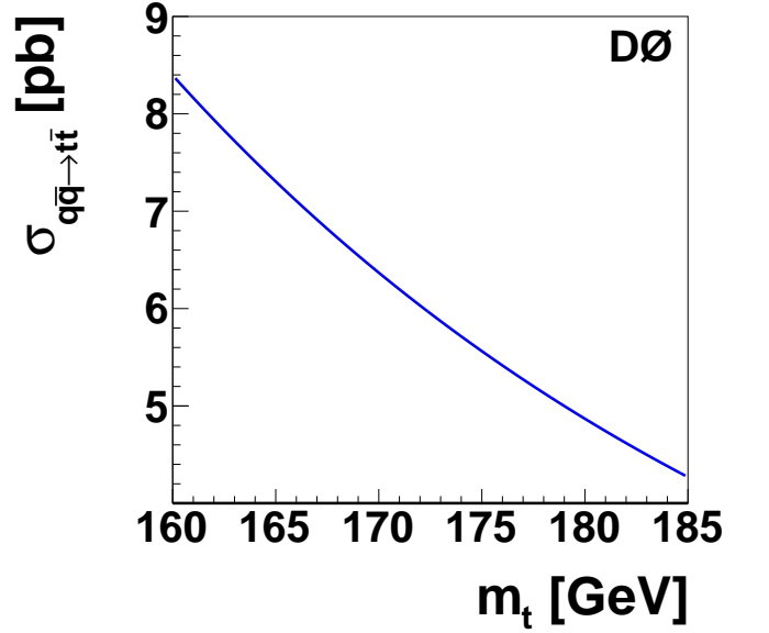
FIG. 1: The total partonic cross section for t\bar{t} production in p\bar{p} collisions through quark-antiquark annihilation at LO, as defined in Eq. (10).
