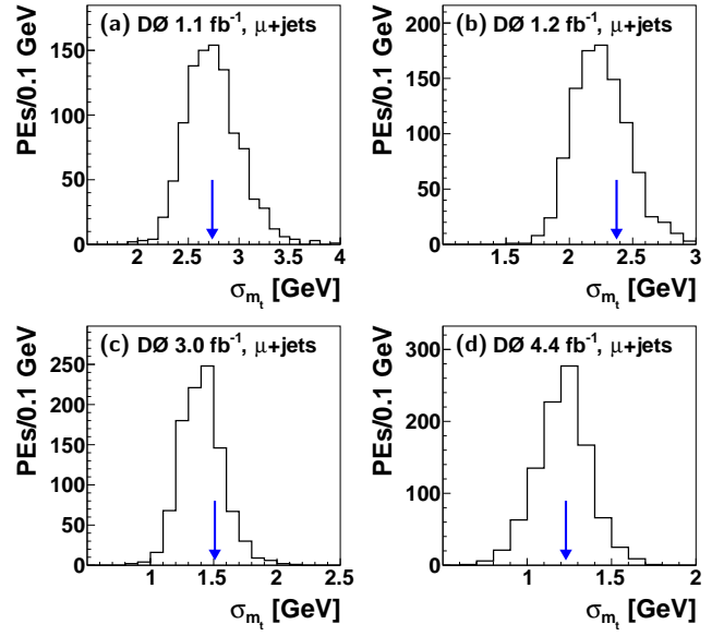
FIG. 21: Same as Fig. 20, in \mu + \text{jets} final states in (a) Run IIa, (b) Run IIb1, (c) Run IIb2, and (d) Run IIb3.
