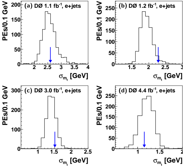
FIG. 20: Distribution of expected statistical uncertainties \sigma_{m_t} in e + \text{jets} final states in (a) Run IIa, (b) Run IIb1, (c) Run IIb2, and (d) Run IIb3, obtained in 1000 PEs at m_t^{\text{gen}} = 172.5 \text{ GeV} and k_{\text{JES}} = 1 , after calibrating for non-unit width of the distribution in \pi_{m_t} . The observed statistical uncertainties in data are indicated by arrows.
