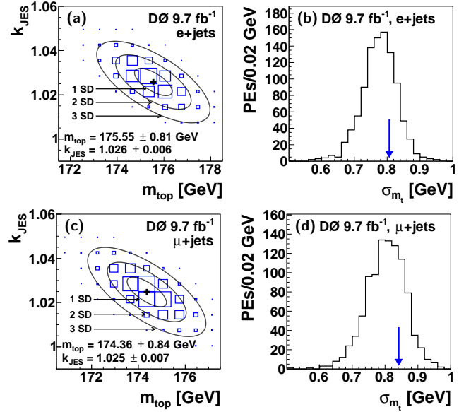
FIG. 25: (a) Two-dimensional likelihood \mathcal{L}(\mathbb{X}_N; m_t, k_{\text{JES}})/\mathcal{L}_{\text{max}} for data in the e+jets final state. Fitted contours of equal probability are overlaid as solid lines. The maximum is marked with a cross. (b) Distribution in expected uncertainty on m_t in e+jets final states, obtained using PEs where the t\bar{t} contribution is taken at m_t^{\text{gen}} = 172.5 GeV and k_{\text{JES}} = 1 , after calibration. The observed statistical uncertainty in data is indicated by the arrow. (c) Same as (a), but for the \mu+jets channel. (d) Same as (b), but for the \mu+jets channel.
