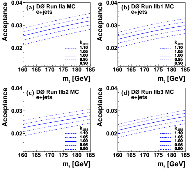
FIG. 2: Mean acceptance \langle A(m_t, k_{\text{JES}} \equiv 1) \rangle_{\vec{x}} with respect to the total partonic cross section for p\bar{p} \rightarrow t\bar{t} production, as a function of m_t for different k_{\text{JES}} values in the e +jets final state, for (a) Run IIa, (b) Run IIb1, (c) Run IIb2, and (d) Run IIb3. The acceptance tends to decrease for later epochs due to a decreased reconstruction efficiency, which is mainly caused by the higher instantaneous luminosity in the second half of Run II and detector aging.
