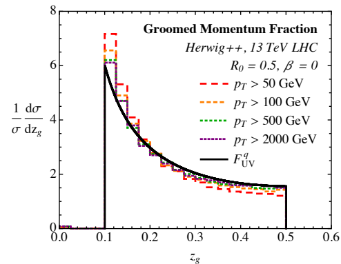
FIG. 2. Distributions of z_g for \beta = 0 and z_{\text{cut}} = 0.1 at the 13 TeV LHC, as simulated by HERWIG++ 2.6.3. The p_T of the jets ranges from 50 GeV to 2 TeV, and the asymptotic distribution for quark jets, F_{\text{UV}}^q in (21), is solid black.
