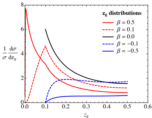
FIG. 1. Distributions of z_g for various \beta values, obtained from (9) at fixed \alpha_s = 0.1 and z_{\text{cut}} = 0.1 .
