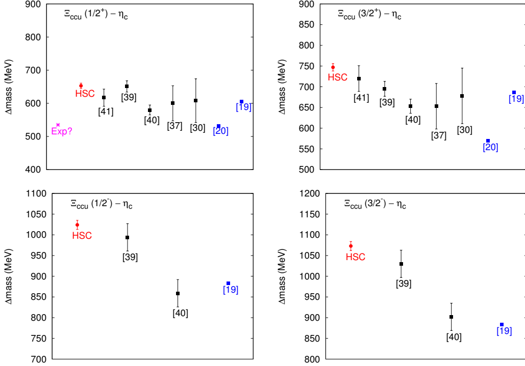
FIG. 9: Ground state masses of spin-1/2 and spin-3/2 doubly-charmed \Xi_{cc} baryons as a splitting from \eta_c meson mass. Our results are shown by the red filled circle (HSC). Our u quark mass is not physical and at pion mass 392 MeV, results for ETMC [38], PACS-CS [41], Bali et. al [40], and Briceno et. al [37] are extrapolated to the physical pion mass, while ILGTI [39] results are at pion mass 390 MeV.
