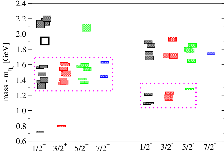
FIG. 12: Spin identified spectra of \Omega_{cc} baryons for both parities and with spin up to 7/2. Energy splittings of the \Omega_{cc} states from the mass of \eta_c meson, which has same number of charm quark, are shown here. All other details are same as in Figure 11.
