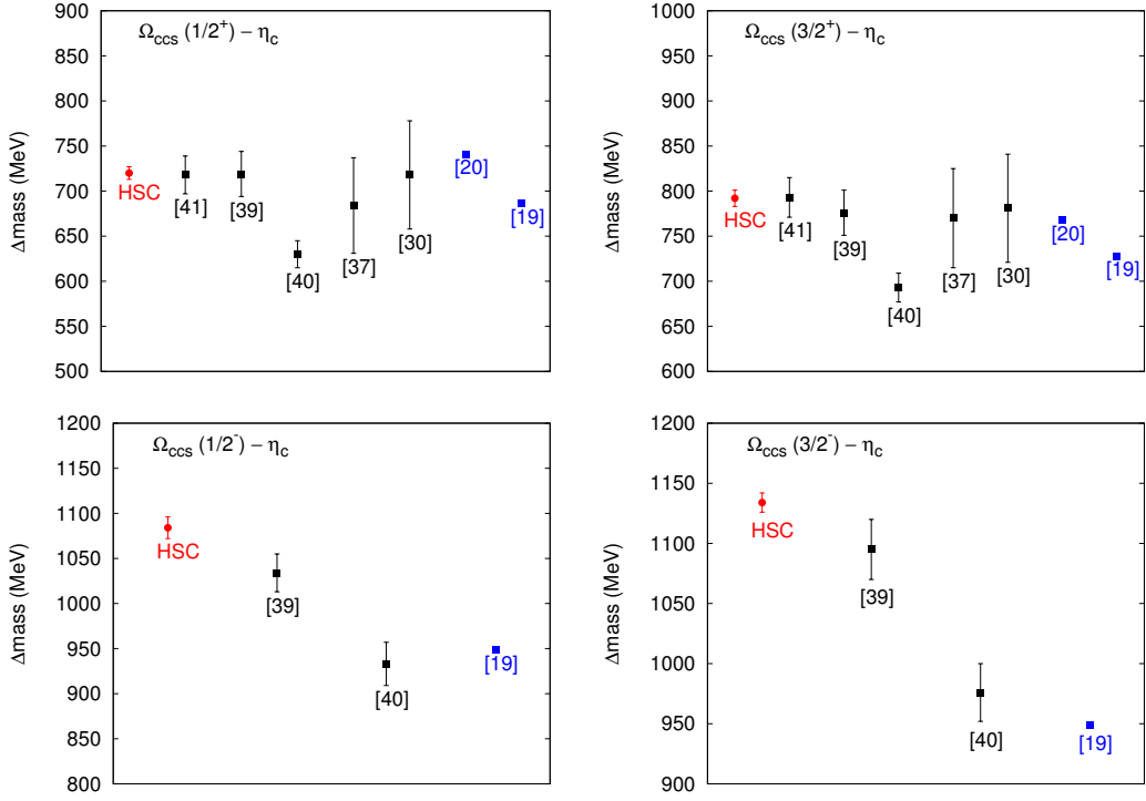
FIG. 10: Ground state masses of spin-1/2 and spin-3/2 doubly-charmed \Omega_{cc} baryons as a splitting from \eta_c meson mass. Our results are shown by the red filled circle (HSC). Other lattice as well as model results are also shown.
