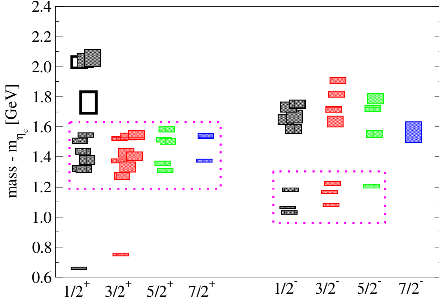
FIG. 11: Spin identified \Xi_{cc} baryon spectra for both parities and with spin up to 7/2. Energy splittings of the \Xi_{cc} baryons from the mass of m_{\eta_c} meson, which has same number of charm quarks, are shown here. The states inside the pink boxes are those with relatively larger overlap to non-relativistic operators and the states with unfilled thick borders corresponds to the states with strong hybrid content. The number of states inside these boxes matches with the expectations based on non-relativistic quark spins, as shown in Table II. This agreement of the number of low lying states between the lattice spectra obtained in this work and the expectations based on non-relativistic quark spins implies a clear signature of SU(6) \times O(3) symmetry in the spectra.
