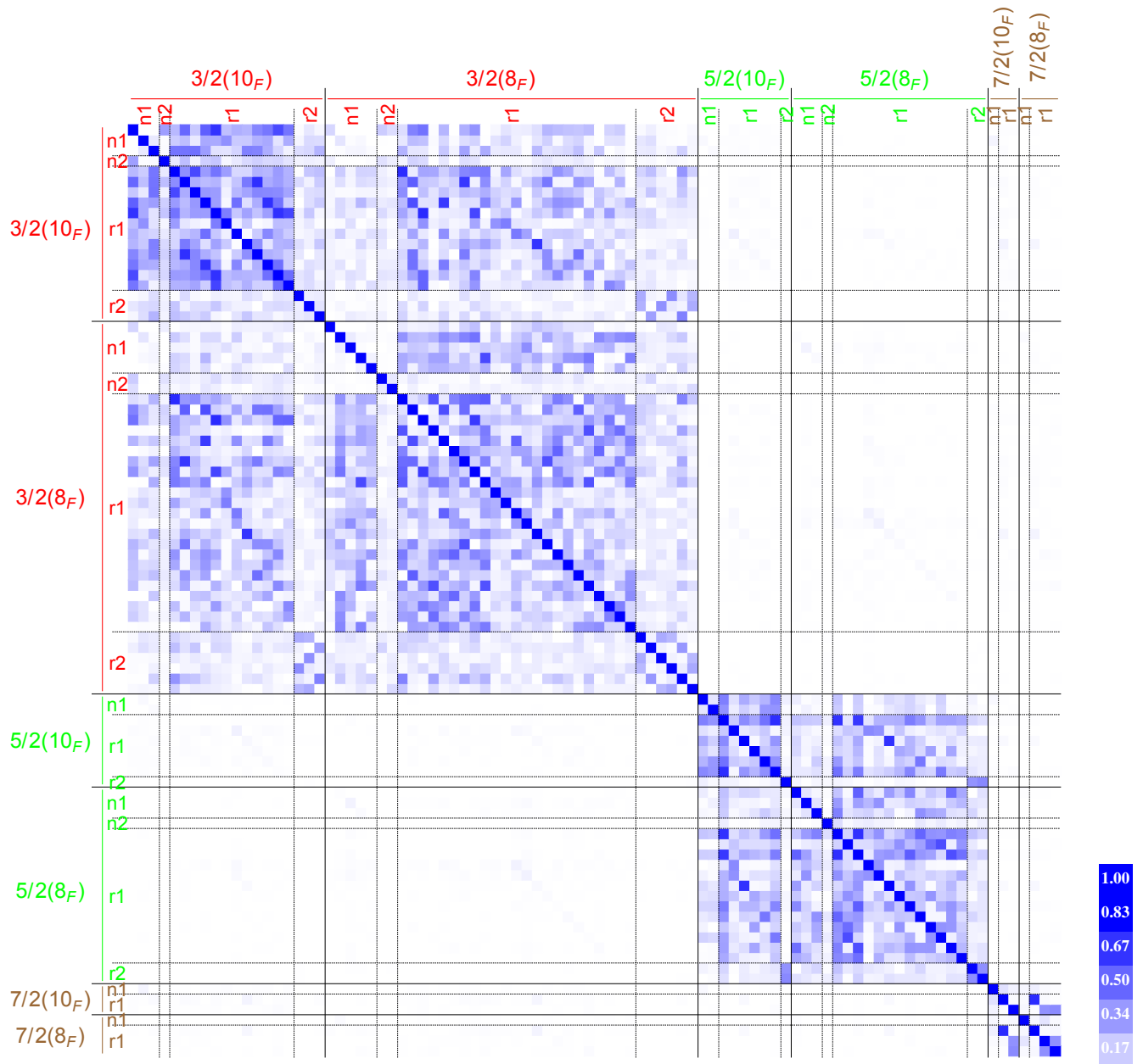
FIG. 3: The normalized correlation matrix, C_{ij}/\sqrt{C_{ii}C_{jj}} , at t/a_t = 5 are shown for \Xi_{cc} baryons in the H_g irrep., according to the darkness scale at the side. The operators are ordered such that those subduced from spin 3/2 appear first followed by spin 5/2 and then spin 7/2. The correlation matrix is observed to be mostly block diagonal in terms of spins which signifies the rotational symmetry on our lattice. There is significant mixing between octet ( 8_F ) and decuplet ( 10_F ) operators which is not present in the corresponding plot for light quark \Sigma(uus) having same operator structures (see figure 2 of Ref.[50]). This signifies that the SU(3) flavor symmetry is badly broken for doubly-charmed \Xi_{cc} baryons. Non-relativistic (n), relativistic (r), non-hybrid (1) and hybrid (2) operators are also identified for each of those spins. The strength of flavor mixing is maximum between relativistic operators (r), while for non-relativistic operators this mixing is relatively mild.
