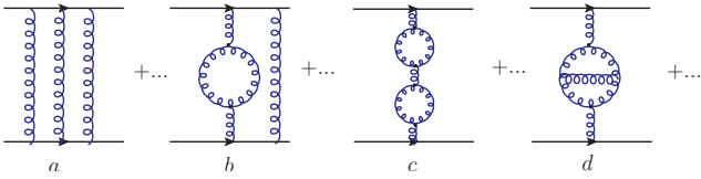
FIG. 1: Diagrammatic illustration for the \beta -pattern of the \alpha_s^3 -correction contributing to the photon polarization operator \Pi [5], following the relation \beta_i \sim \beta_0^{i+1} : (a) diagrams without any intrinsic renormalization contributions to r_3[0] ; (b) diagrams contributing to the \beta_0 -term r_3[1] ; (c) diagrams contributing to the \beta_0^2 -term r_3[2] ; (d) diagrams contributing to the \beta_1 -term r_3[0, 1] . The ellipses denote other diagrams with the gluon/vertex renormalization.
