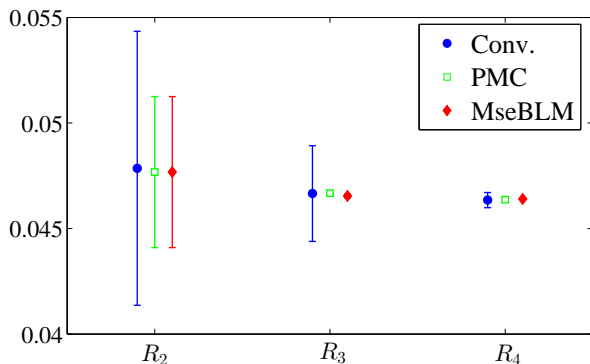
FIG. 2: Results for R_n ( n = 2, 3, 4 ) together with their errors ( \pm |\tilde{\mathcal{C}}_n a^{n+1}|_{\text{MAX}} ) at Q = 31.6 GeV. The big dots, the squares and the diamonds are for conventional scale setting (Conv.), PMC and MseBLM, respectively.
