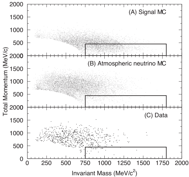
FIG. 2. Total momentum vs. the invariant mass after applying the selection criteria (a) and (b) on the FC sample: (A) signal MC, (B) atmospheric neutrino MC, and (C) Data. The boxed region in each panel shows the criterion (c) and (d) for the n - \bar{n} oscillation signal.
