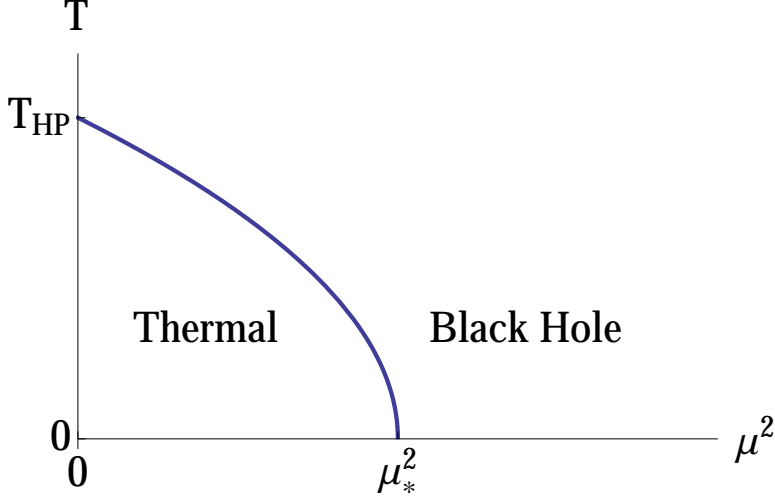
Figure 1: Phase diagram for holographic massive gravity showing the Hawking-Page temperature, T_{HP}(\mu^2) , v.s. the mass parameter, \mu^2 . The region below the purple line is a confined phase in which the thermal solution dominates the ensemble, while the region above the line is a deconfined phase in which the black hole solution dominates. The line of first-order phase transitions terminates in a second-order phase transition at zero temperature and \mu^2 = \mu_*^2 = 2/L^2 .
