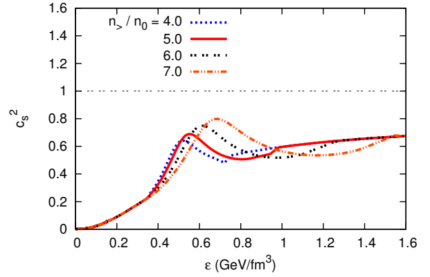
FIG. 12. The speed of sound c_s^2 = \partial P / \partial \epsilon as a function of \epsilon . The NJL parameter set is the same as Fig. 11, for different values of the high density boundary: n_> / n_0 = 4.0, 5.0, 6.0, and 7.0 . For each of these choices, the causality condition is satisfied.
