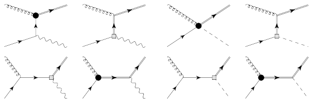
FIG. 1. Tree-level diagrams for pp \rightarrow tV and pp \rightarrow th . The black dots represent contributions from color dipole operators O_{uG}^{(i3,3i)} , while the shaded squares represent other operators.
