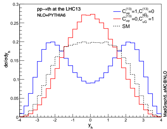
FIG. 4. Normalized rapidity distribution of the Higgs boson in pp \rightarrow th induced by operators O_{u\varphi}^{(13)} and O_{uG}^{(13)} .
