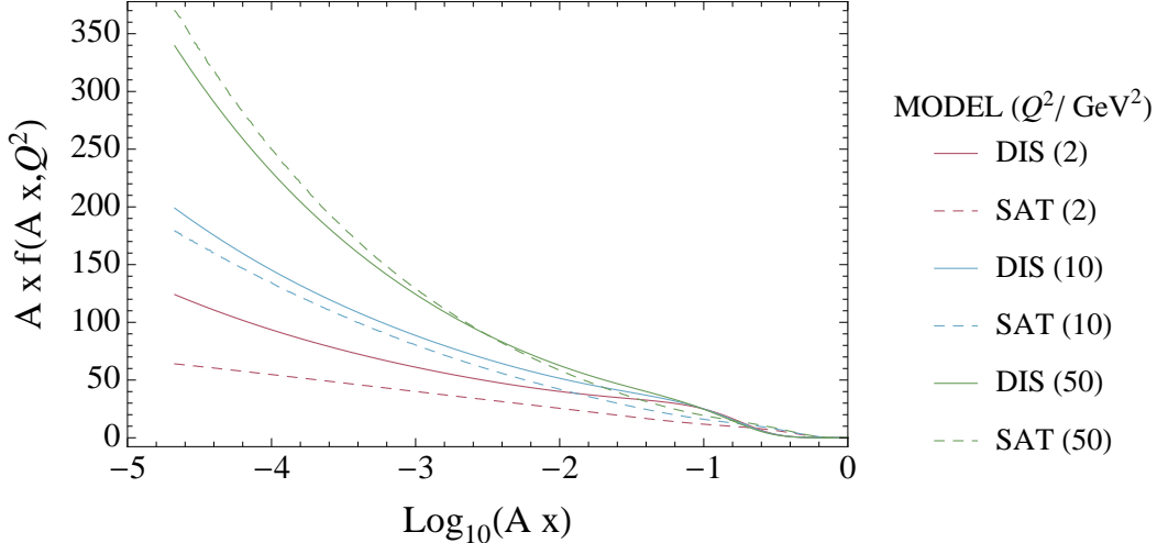
FIG. 7: The parton distribution function f_{q/A}(x, Q^2) for \bar{u} quarks in a uranium nucleus according to the HKNlo parton distributions [34] used in this paper compared to the same distribution in the saturation model, Eq. (31). We plot Ax f_{q/A}(Ax, Q^2) versus \log_{10}(Ax) for Q^2 = 2 \text{ GeV}^2 , 10 \text{ GeV}^2 , and 50 \text{ GeV}^2 .
