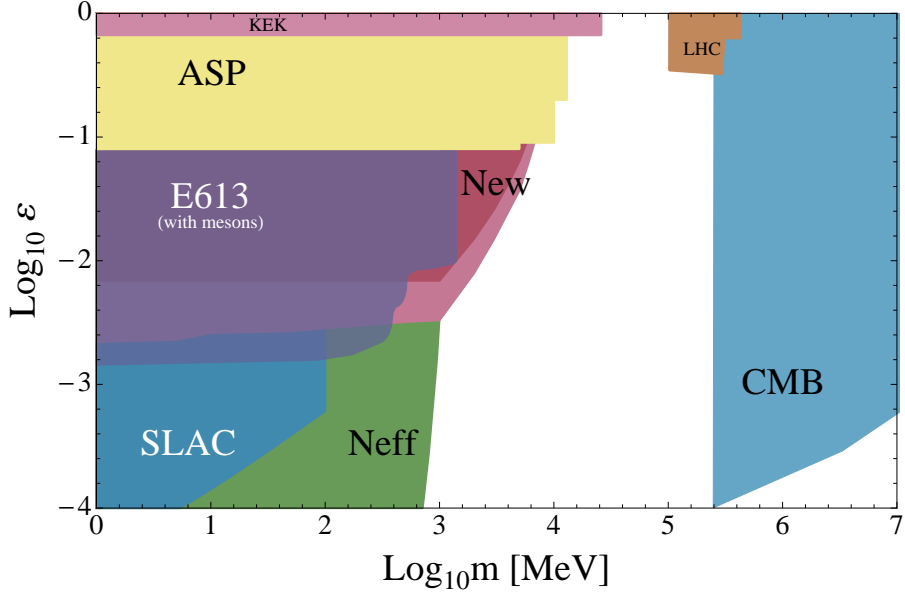
FIG. 9: Exclusion limits for minicharged particles in the MeV to GeV mass regime, including the results of this analysis. Other constraints are shown, arising from colliders [59], a SLAC beam dump [60], the LHC [61], CMB [62, 63] and recent work on the number of light species, N_{\text{eff}} [64].
