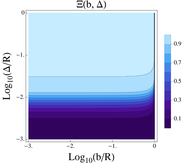
FIG. 6: The function \Xi(\mathbf{b}, \Delta) as a function of |\mathbf{b}|/R and |\Delta|/R where R is the radius of the lead nucleus. We calculate \Xi(\mathbf{b}, \Delta) using Eqs. (25), (26), and (27) with parameters given in Eqs. (28) and (29) and using HKNlo parton distributions for the distribution of gluons in a lead nucleus, with x = 10^{-4} and Q^2 = 1 \text{ GeV}^2 .
