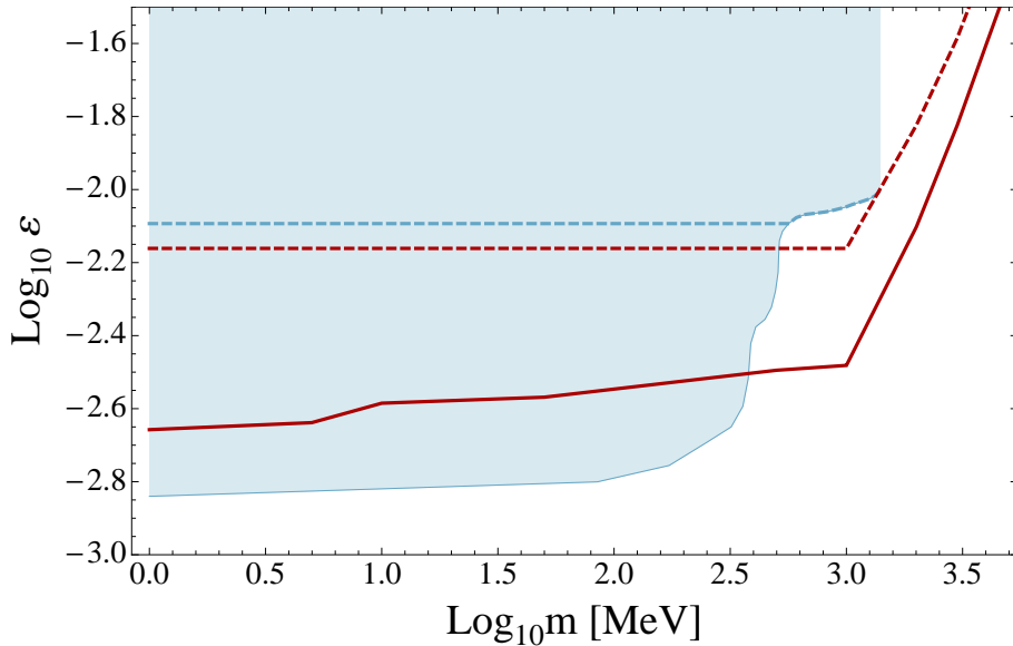
FIG. 9: Exclusion limits for minicharged particles in the MeV to GeV mass regime, including the results of this analysis. Other constraints are shown, arising from colliders [59], a SLAC beam dump [60], the LHC [61], CMB [62, 63] and recent work on the number of light species, N_{\text{eff}} [64].
