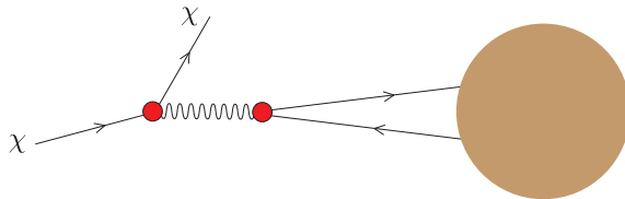
FIG. 4: Dipole picture for a \chi particle scattering from a nucleus.
