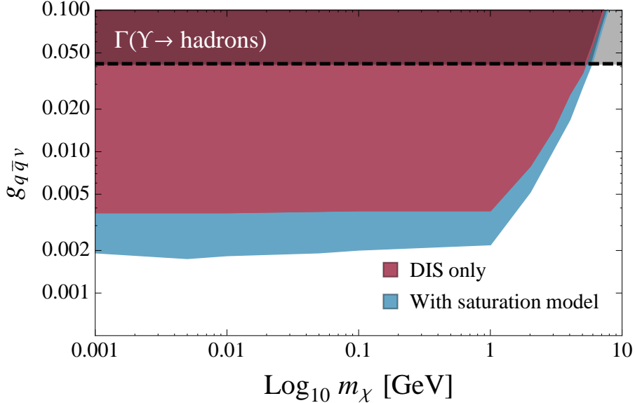
FIG. 8: Exclusion limits for the leptophobic model described in the text, with g_{\chi\bar{\chi}v} = 1 and a mediator mass of 1 MeV. Also plotted is the region excluded by the study of \Upsilon decays from [26].
