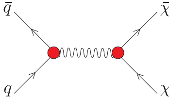
FIG. 1: Feynman diagram for direct production of \chi particles from pA collisions.
