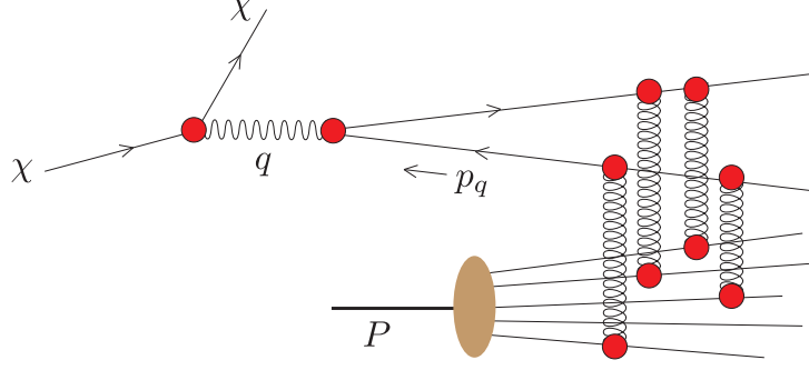
FIG. 5: The dipole created by the dark vector boson interacts with the nucleus via gluon exchange.
