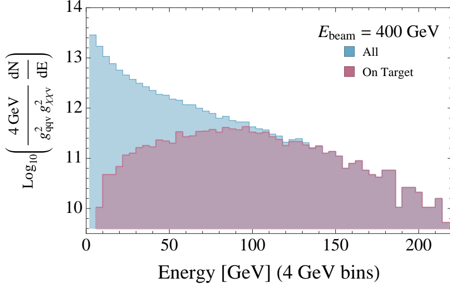
FIG. 2: Typical distribution of \chi particles as a function of energy, \frac{dN}{dE} , divided by g_{qqv}^2 g_{\chi\chi v}^2 . The vertical scale is logarithmic. We show the distribution of all produced particles \chi and \bar{\chi} and the distribution of particles produced at angles that will result in their impacting the target. Many of the lowest energy dark particles are produced at wide angles and miss the detector.
