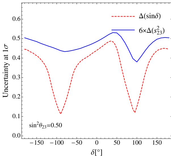
FIG. 8: Comparison between the precision achievable for \sin^2 \theta_{23} and the precision achievable for \sin \delta for the T2HK setup. The solid line shows the error on \sin^2 \theta_{23} multiplied by a factor of 6, while the dashed lines show the error on \sin \delta as obtained directly from a simulation. The agreement between the two curves is noticeable in most of the \delta parameter space, as predicted by Eq. (9), which was derived from simple analytical considerations in Ref. [13] for facilities sitting at the first VOM. It should be noted that in this figure the full size of the confidence interval is plotted in both cases, unlike for the rest of the figures in this paper where we show half of the size of the full confidence interval.
