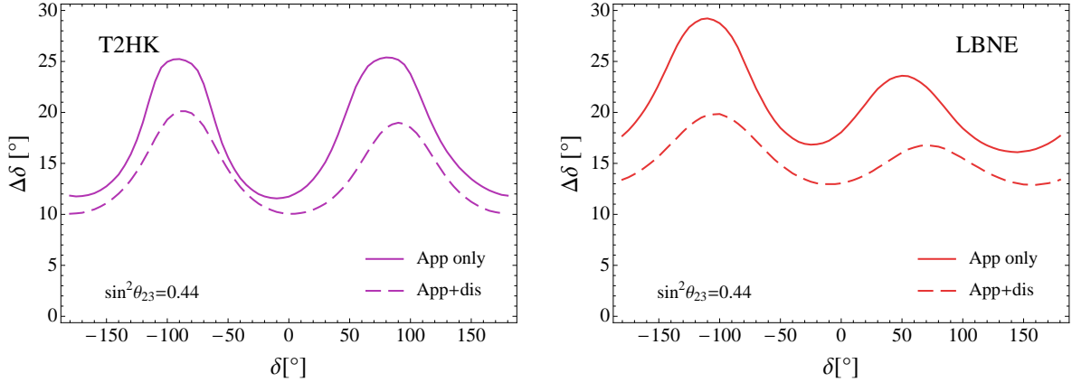
FIG. 9: Precision on \delta (at 1\sigma , for 1 d.o.f.) as a function of the value of \delta itself, for T2HK in the left panel and for LBNE in the right panel. Solid lines show the results using the appearance channels only, while dashed lines show the results from the combination of appearance and disappearance data.
