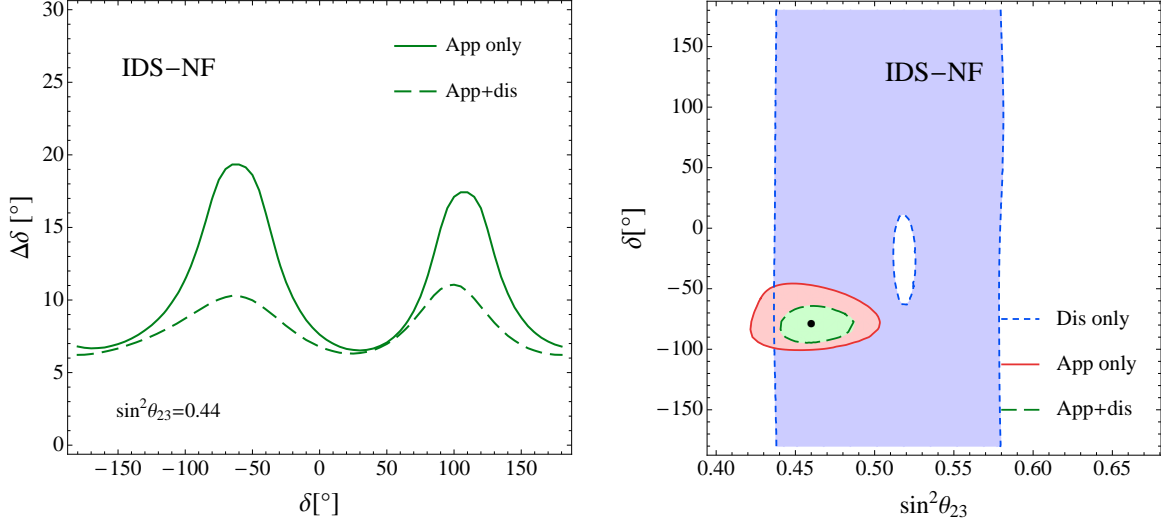
FIG. 10: Left panel: expected precision on \delta (at 1\sigma , for 1 d.o.f.) as a function of the value of \delta itself, for the IDS-NF setup. Solid and dashed lines indicate the results obtained from the appearance results alone and from the combination between appearance and disappearance data, respectively. Right panel: confidence regions in the \sin^2\theta_{23} - \delta plane (at 1\sigma , for 2 d.o.f.) , for a particular set of true values and for different combinations of oscillation channels, as indicated in the legend. Results in both panels correspond to the IDS-NF setup as defined in Sec. III. It should be pointed out that the “hole” in the confidence region obtained for the disappearance channels vanishes just above the 1\sigma CL.
