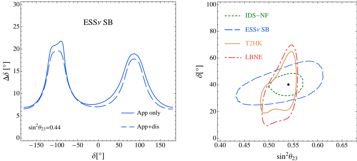
FIG. 11: Left panel: expected precision on \delta (at 1\sigma , for 1 d.o.f.) as a function of the value of \delta itself for the ESS \nu SB setup. Solid and dashed lines indicate the results obtained from the appearance results alone and from the combination between appearance and disappearance data, respectively. Right panel: confidence regions in the \sin^2\theta_{23} - \delta plane (at 1\sigma , for 2 d.o.f.), for a particular set of true values (indicated by the black dot) and for the four setups considered in this work. See Tabs. I and II for a precise definition of the different setups and for the expected number of events in each oscillation channel, respectively. In this panel, all regions include data from both appearance and disappearance channels.
