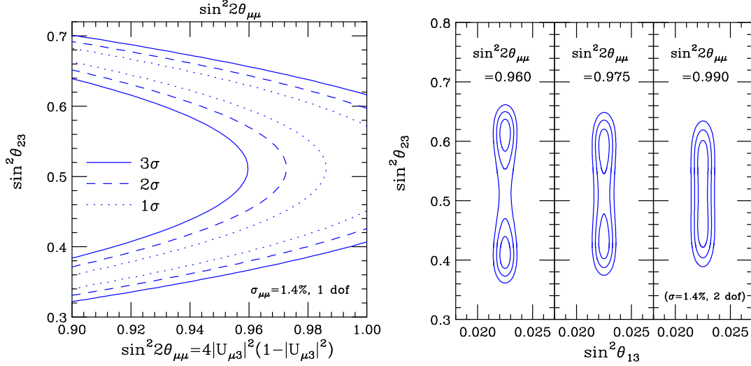
FIG. 3: Left panel: Contours for the \chi^2 distribution in the \sin^2 2\theta_{\mu\mu} - \sin^2 \theta_{23} plane, where \chi^2 \equiv (4 \cos^2 \theta_{13} \sin^2 \theta_{23} (1 - \cos^2 \theta_{13} \sin^2 \theta_{23}) - \sin^2 2\theta_{\mu\mu})^2 / (\sigma_{\mu\mu} \sin^2 2\theta_{\mu\mu})^2 , \sin^2 \theta_{13} = 0.023 and \sigma_{\mu\mu} = 1.4\% . Right panel: Contours for the same \chi^2 in the \sin^2 \theta_{13} and \sin^2 \theta_{23} plane, for different values of \sin^2 2\theta_{\mu\mu} as indicated in each sub-panel. With the assumed uncertainty, there are two distinct allowed bands for \sin^2 \theta_{23} for values of \sin^2 2\theta_{\mu\mu} < 0.96 , whereas the two bands start to merge for \sin^2 2\theta_{\mu\mu} > 0.96 . Note the small upward shift with respect to the line \sin^2 \theta_{23} = 0.5 caused by the non-zero value of \sin^2 \theta_{13} . In both panels, the different lines correspond to different confidence levels as indicated in the legend. Note that the left panel corresponds to 1 d.o.f. while the right panel is obtained for 2 d.o.f.
