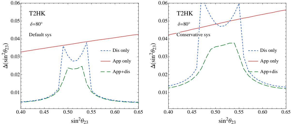
FIG. 5: Expected precision for \sin^2 \theta_{23} at 1\sigma (1 d.o.f.) as a function of the true value of \sin^2 \theta_{23} for the T2HK setup. The left and the right panels correspond to our reference ( \sim 5 - 10\% ) and conservative ( \sim 10 - 15\% ) sets of systematic errors, respectively. See App. A for more precise specification of the reference errors. The true value of \delta is taken as 80^\circ .
