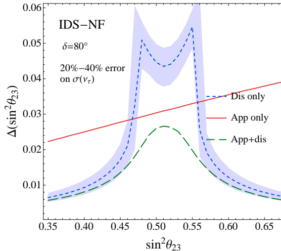
FIG. 7: Same as left panel in Fig. 5, but for the IDS-NF setup. All lines correspond to the assumed uncertainty for this parameter in our default scenario (30%), while the blue band shows the impact on the result for the disappearance channels if the systematic error on the \nu_\tau cross section is varied between a 20% and a 40%.
