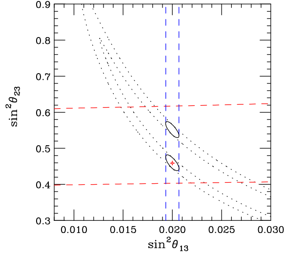
FIG. 4: Allowed confidence regions in the \sin^2 \theta_{13} - \sin^2 \theta_{23} plane at the 2 \sigma CL (2 d.o.f.), using different oscillation channels, for an experiment with a baseline of 295 km and a (monochromatic) neutrino energy of 0.8 GeV ( i.e. , \Delta_{31} \sim 3\pi/8 ). The allowed region for the appearance \nu_\mu \rightarrow \nu_e and \bar{\nu}_\mu \rightarrow \bar{\nu}_e measurements is given by the dotted black bands. The vertical blue and (almost) horizontal red bands indicate the regions allowed by the \nu_e and \nu_\mu disappearance measurements constraints on \sin^2 2\theta_{13} and \sin^2 2\theta_{\mu\mu} . Finally, the solid black ellipses are the overlap regions for these three types of measurements.
