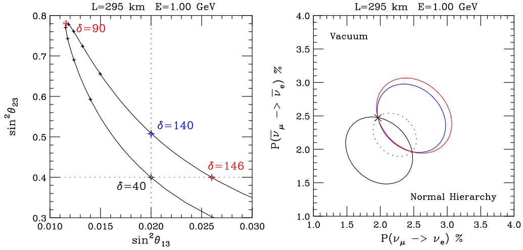
FIG. 1: Left panel: Set of points in the \sin^2 \theta_{13} - \sin^2 \theta_{23} plane which simultaneously give P(\nu_{\mu} \rightarrow \nu_e) \approx 0.02 and P(\bar{\nu}_{\mu} \rightarrow \bar{\nu}_e) \approx 0.025 in vacuum, for E_{\nu} = 1 GeV and L = 295 km. Each point in the curve corresponds to a different value of \delta . Larger stars on the curve mark the points corresponding to the \theta_{23} and \theta_{13} intrinsic degeneracy solutions. Small stars indicate values of \delta in steps of 10^\circ , from 40^\circ to 140^\circ . Notice the accumulation of points \delta = 80^\circ, 90^\circ , and 100^\circ near the tip of the “tusk”. Right panel: The bi-probability plot in P(\nu_{\mu} \rightarrow \nu_e) vs. P(\bar{\nu}_{\mu} \rightarrow \bar{\nu}_e) space. The points with large stars on the curve in the left panel correspond to the ellipses with the same color in the right panel. The dotted curve is the smallest ellipse that can be drawn through these points.
