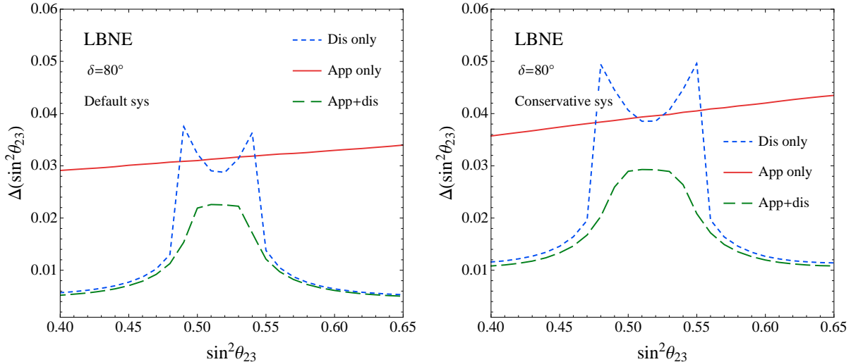
FIG. 6: Same as in Fig. 5, but for the LBNE setup.
