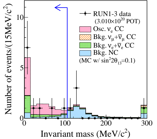
FIG. 24. Distribution of invariant mass M_{\text{inv}} when each event is forced to be reconstructed as two photon rings. The data are shown as points with error bars (statistical only) and the MC predictions are in shaded histograms. The last bin shows overflow entries. The arrow shows the selection criterion M_{\text{inv}} < 105 \text{ MeV}/c^2 .
