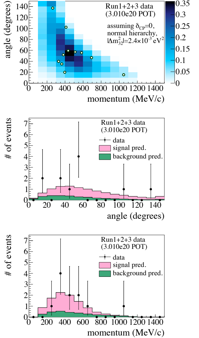
FIG. 35. The (p_e, \theta_e) distribution of the \nu_e events (dots) (top) overlaid with the prediction. The prediction includes the rate tuning determined from the fit to near detector information and a signal assuming the best-fit value of \sin^2 2\theta_{13}=0.088 . The angular distribution (middle) of the \nu_e events in data overlaid with prediction, and the momentum distribution (bottom) with the same convention as above.
