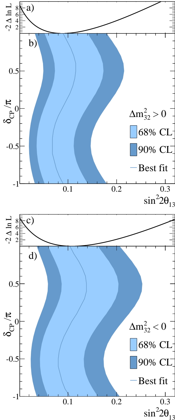
FIG. 36. The 68% and 90% confidence intervals for \sin^2 2\theta_{13} scanned over values of \delta_{CP} assuming normal hierarchy (top, b) and inverted hierarchy (bottom, d) with all other oscillation parameters fixed at the values in Table XIII. The best-fit value of \sin^2 2\theta_{13} for each value of \delta_{CP} is also shown for the (p_e, \theta_e) analysis. The -2\Delta \ln \mathcal{L} curve for normal hierarchy (top, a) and inverted hierarchy (bottom, c) at \delta_{CP}=0 are also shown vs. \sin^2 2\theta_{13} .
