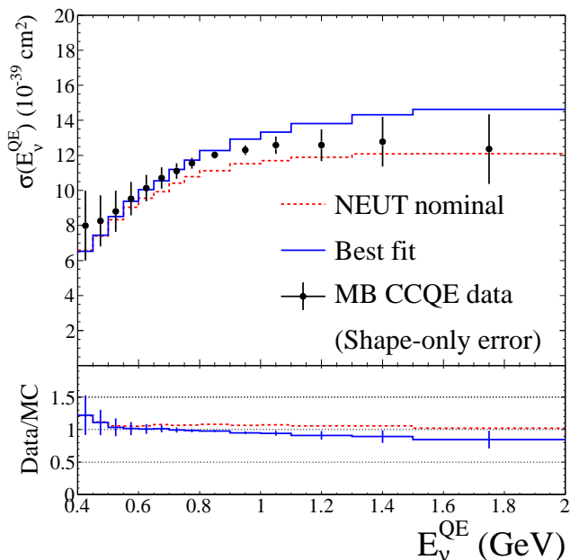
FIG. 41. The CCQE cross section as a function of neutrino energy (top) as measured by MiniBooNE (points), with the NEUT nominal and NEUT at the best-fit of the MiniBooNE CCQE ( T_\mu, \cos\theta_\mu ) spectrum. Ratio of data to NEUT (bottom) for nominal (dashed) and best-fit (solid).
