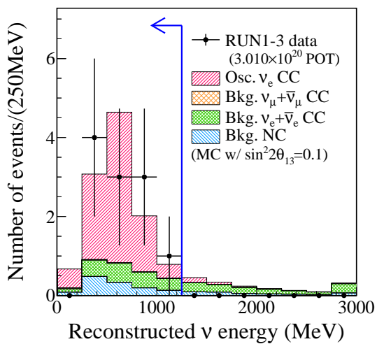
FIG. 25. Distribution of the reconstructed neutrino energy spectrum of the events which pass all \nu_e appearance signal selection criteria with the exception of the energy cut. The data are shown as points with error bars (statistical only) and the MC predictions are in shaded histograms. The arrow shows the selection criterion E_\nu^{\text{rec}} < 1250 MeV.
