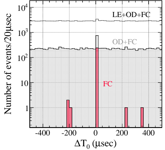
FIG. 22. \Delta T_0 distribution of all FC, OD and LE events observed in the \pm 500 \mu\text{s} T2K windows. The OD histogram is stacked on the FC histogram, and the LE histogram is stacked on the OD and FC histograms.
