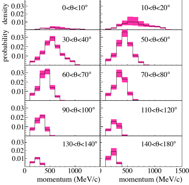
FIG. 32. The PDF as a function of momentum for different angular bins (10 of 15 (p_e, \theta_e) bins are shown) and \sin^2 2\theta_{13}=0.1 . The shaded areas represent one sigma deviations that are evaluated by fluctuating all of the systematic parameters that are evaluated to a multivariate normal distribution using their prior values and covariance matrix.
