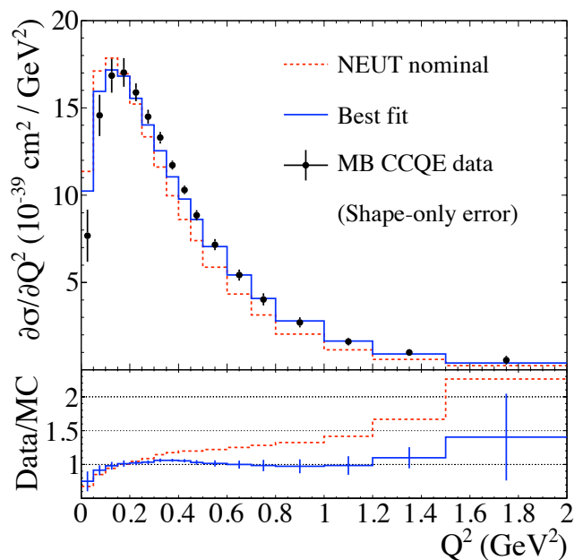
FIG. 40. The CCQE cross section as a function of Q^2 (top) as measured by MiniBooNE (points), with the NEUT nominal and NEUT at the best-fit of the MiniBooNE CCQE (T_\mu, \cos \theta_\mu) spectrum. Ratio of data to NEUT (bottom) for nominal (dashed) and best-fit (solid).
