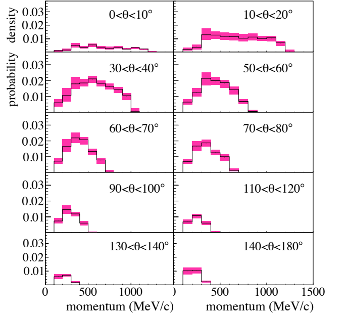
FIG. 33. The PDF as a function of momentum for for the same bins as in Fig. 32 and \sin^2 2\theta_{13}=0 . The shaded areas represent one sigma deviations that are evaluated by fluctuating all of the systematic parameters according to a multivariate normal distribution using their prior values and covariance matrix.
