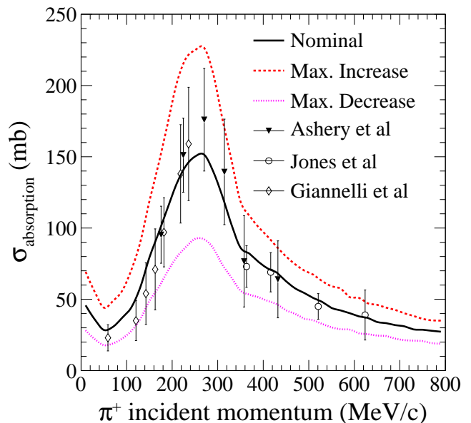
FIG. 39. Pion absorption cross section as a function of pion momentum overlaid with \pi^+ \text{-}^{12}\text{C} scattering data, Ashery et al. [79], Jones et al. [80], and Giannelli et al. [81].
