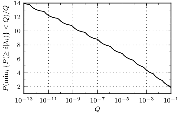
FIG. 4. The effective trials factor that is applied to the statistic Q = \min_i \{P(\geq i|\lambda(\mathcal{L}_i^*))\} in order to obtain the FAP for Q . The effective trials factor grows with increasing significance of the observed statistic.
