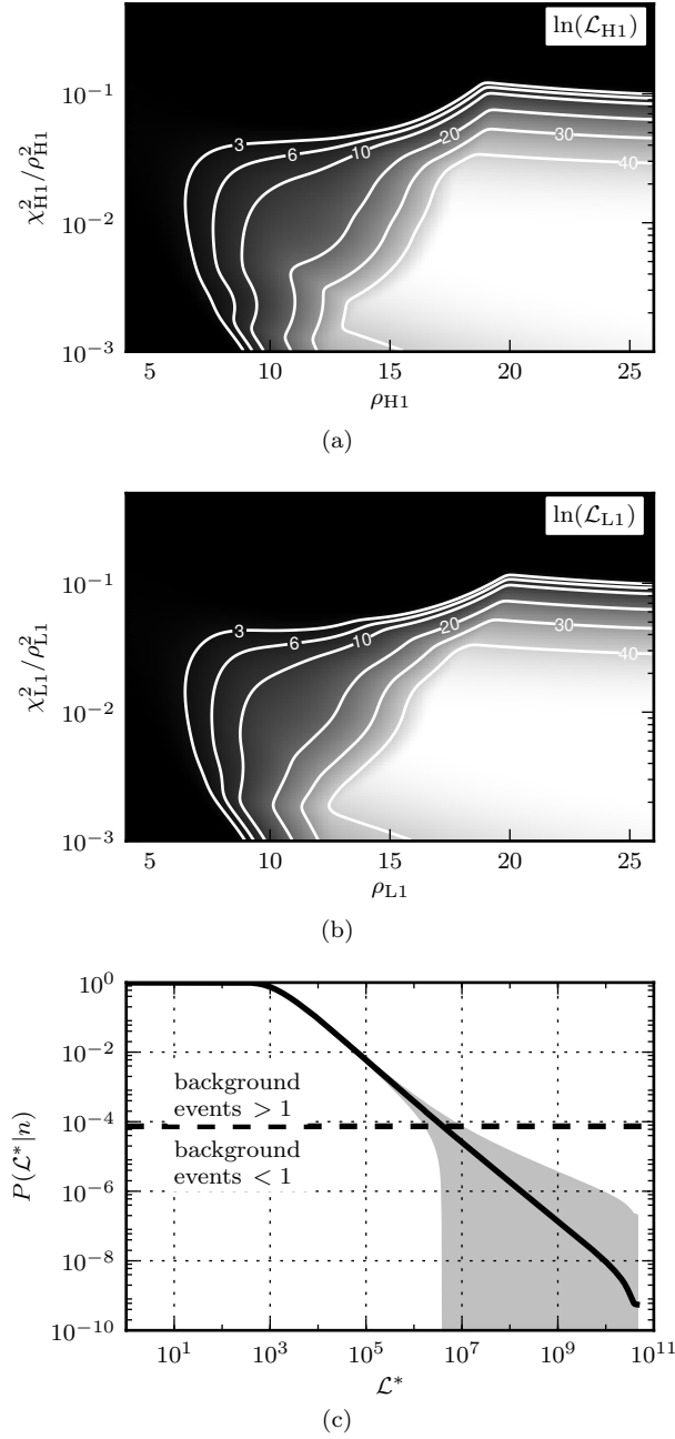
FIG. 1. Figure 1(a) and 1(b) show the likelihood ratios \mathcal{L}_{H1} , \mathcal{L}_{L1} as a function of \rho and \chi^2 for H1 and L1 respectively for templates with masses consistent with neutron star binaries ( 1.2-2 M_{\odot} .) \mathcal{L}_{H1} , \mathcal{L}_{L1} appear as the right-hand-side of (2). White indicates high likelihood ratio values. Figure 1(c) shows the probability of having obtained a given value of likelihood ratio \mathcal{L}^* or greater from noise as defined in (8) after M trials (where M is the number of independent coincidences formed. In this example M = 6 \times 10^4 .)
