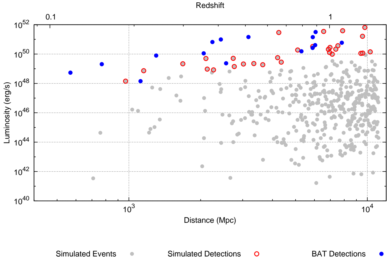
FIG. 1: SGRB luminosity and distance distribution for approximately a year of simulated events (grey) and simulated detections, with flux \geq 10^{-8} \text{ erg cm}^{-2} \text{ s}^{-1} (red). Isotropic equivalent luminosity in the BAT band is plotted against luminosity distance and redshift. Over-plotted are the SGRBs with known distances from Table III (excluding GRB 090426 at z = 2.6 ). The simulated and observed SGRB properties appear consistent, and larger samples of data show populations with matching average properties.
