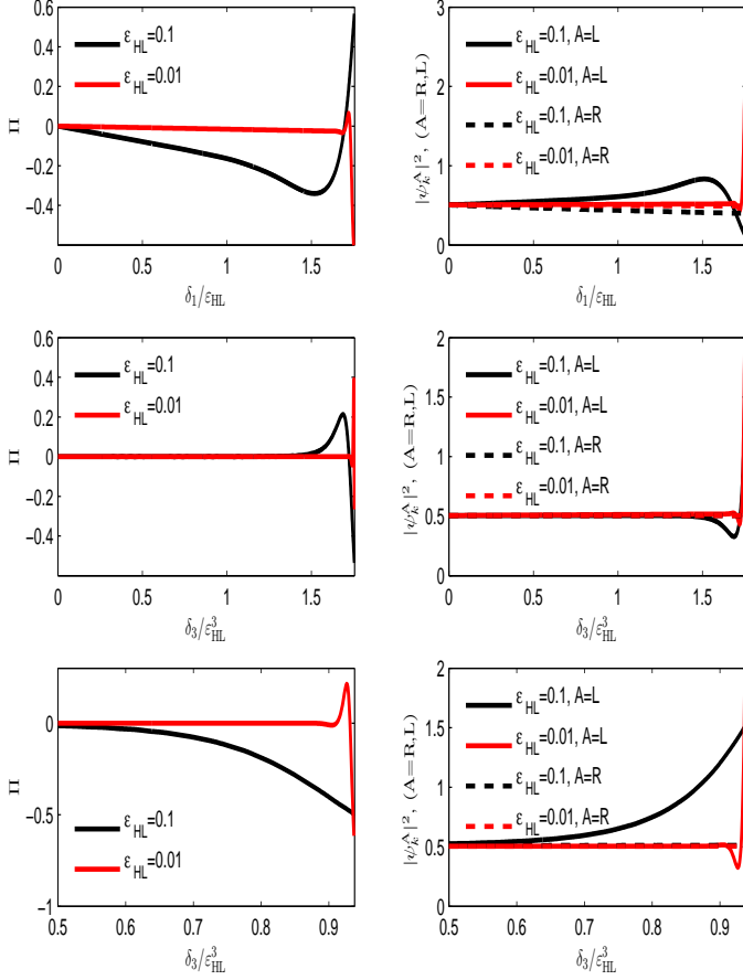
FIG. 2: (a) Top panel: \delta_1 \neq 0 , \delta_2 = \delta_3 = 0 . (b) Middle panel: \delta_3 \neq 0 , \delta_1 = \delta_2 = 0 . (c) Low panel: \delta_1 = 0 , \delta_2 = -\varepsilon_{\text{HL}}^2 . In all the plots, we have set \delta_4 = \varepsilon_{\text{HL}}^4 .
