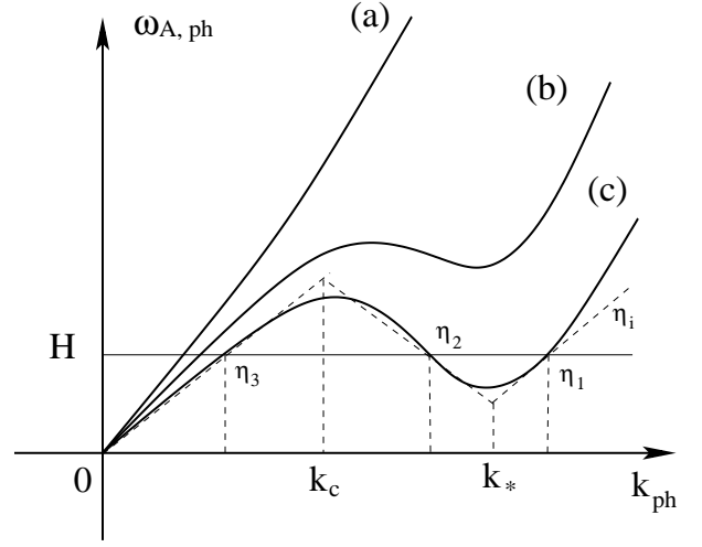
FIG. 1: The evolution of \omega_{A,ph} vs k_{ph} for (i) \delta_2 = \delta_3 = 0 or (ii) \delta_1 = \delta_2 = 0 , where k_{ph} \equiv k/a . Region I: \eta \in (\eta_i, \eta_1) ; Region II: \eta \in (\eta_1, \eta_2) ; Region III: \eta \in (\eta_2, \eta_3) ; and Region IV: \eta \in (\eta_3, 0) .
