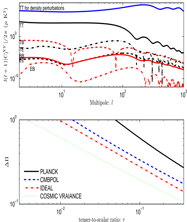
FIG. 3: Top panel: The CMB power spectra generated by polarized PGWs with r = 0.1 and \Pi = 1 , and the TT power spectrum generated by density perturbations for comparison. Low panel: The uncertainties \Delta\Pi as a function of r for potential observations.
