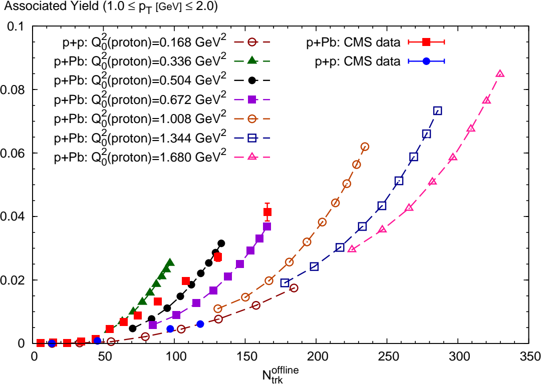
FIG. 2. The nearside yield per trigger as a function of N_{\text{trk}}^{\text{offline}} (specific to the acceptance of the CMS experiment) for 1 \leq p_T \leq 2 , for p_T = p_T^{\text{trig}} = p_T^{\text{asc}} . The open circles (brown) are the computed Glasma graph yield for increasingly rare proton initial saturation scales in multiples N_{\text{part}}^{\text{proton}} of Q_0^2 = 0.168 \text{ GeV}^2 . The filled circles (blue) are proton-proton data at \sqrt{s} = 7 \text{ TeV} from the CMS collaboration. Each of the p+Pb curves corresponds, for fixed Q_0^2(\text{proton}) , to the increasing yield with a larger number of participants in the nucleus (in increments of two, from N_{\text{part}}^{\text{Pb}} = 6 to N_{\text{part}}^{\text{Pb}} = 22 ), where N_{\text{part}}^{\text{Pb}} denotes the initial saturation scale in the Pb nucleus through the relation Q_0^2(\text{lead}) = N_{\text{part}}^{\text{Pb}} \cdot 0.168 \text{ GeV}^2 . The three curves with open symbols are new computations for higher multiplicities. In this case the number of participants in the nucleus increases in increments of two up to N_{\text{part}}^{\text{Pb}} = 26 . The red squares are CMS data for proton-lead collisions at \sqrt{s} = 5.02 \text{ GeV/nucleon} . Similar curves are obtained for the N_{\text{trk}}^{\text{offline}} appropriate in the acceptance of the other experiments.
