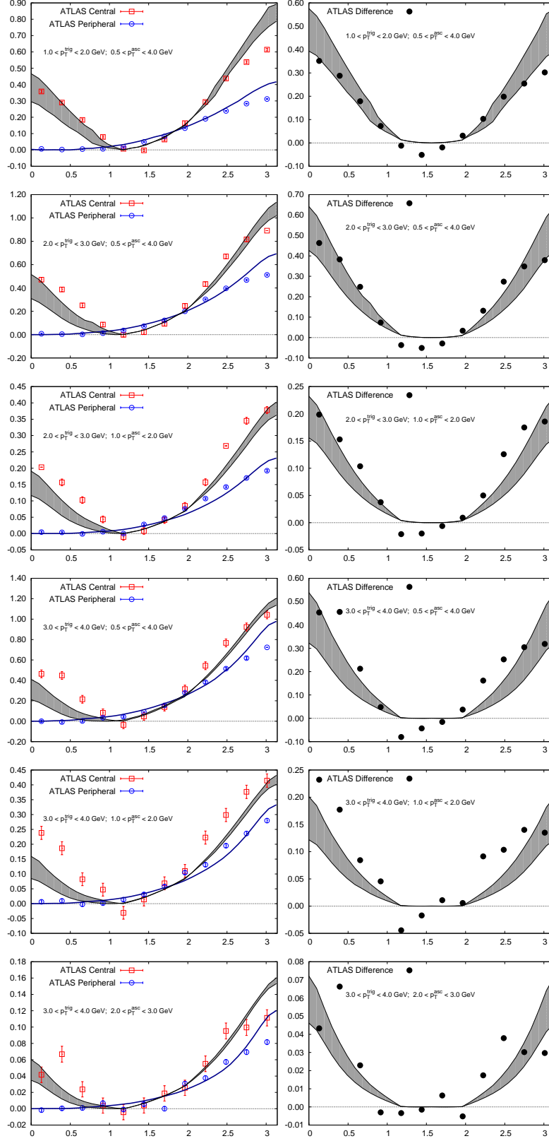
FIG. 8. Per-trigger-yield 1/N_{\text{trig}} d^2 N/d\Delta\phi versus |\Delta\phi| for asymmetric p_T^{\text{trig}}, p_T^{\text{asc}} . Red squares are the ATLAS data for central p+Pb events, blue circles are for peripheral p+Pb events. The blue curves show the results of the BFKL contribution for (N_{\text{part}}^{\text{proton}}, N_{\text{part}}^{\text{Pb}})=(1,3) . The gray band, representative of central collisions, corresponds to (4,14)–lower curve and (3,22)–upper curve.
