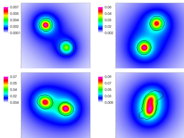
FIG. 2: The scalar field (color code) and the NS surfaces (solid black line) at t = \{1.8, 3.1, 4.0, 5.3\} ms for \beta/(4\pi G) = -4.5 , and the binary of Fig. 1.
