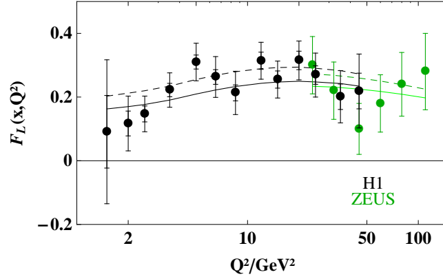
Figure 5: The proton structure function F_L as a function of Q^2 . The average x values for each Q^2 of the H1 data (black) are given in Figure 13 of [19]. ZEUS data are taken from [20]. The solid line represents our calculation with the LO photon impact factor and the dashed line using the kinematically improved one.
