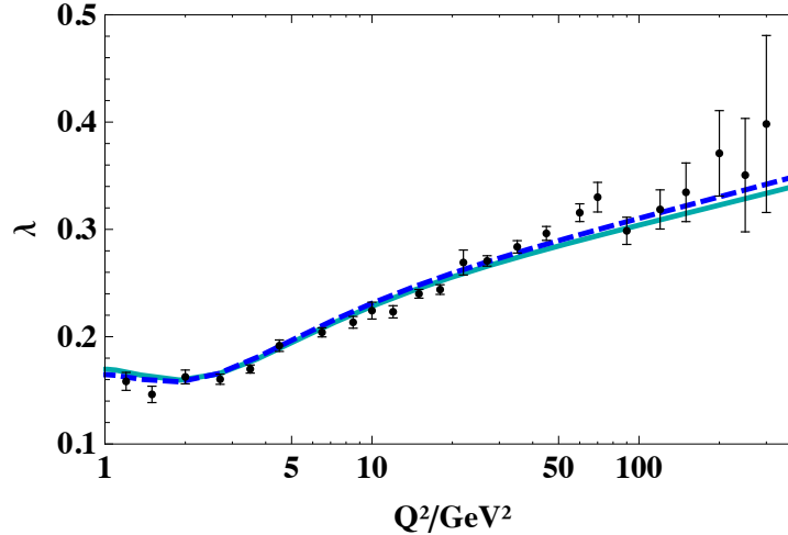
Figure 1: Fit to \lambda for F_2 with the LO photon impact factor (solid line) and the kinematically improved one (dashed line). The data set has been extracted from [17].
