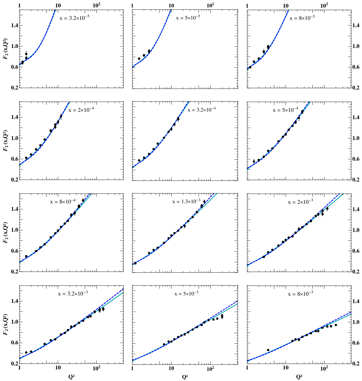
Figure 2: Study of the dependence of F_2(x, Q^2) on Q^2 using the LO photon impact factor (solid lines) and the kinematically improved one (dashed lines). Q^2 runs from 1.2 to 200 \text{GeV}^2 .
