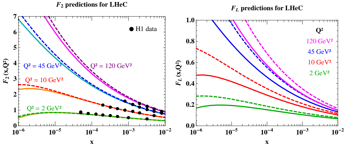
Figure 6: Predictions for F_2 (left) and F_L (right) for LHeC. On the left plot, the curve with Q^2 = 10\text{GeV}^2 can be compared with Figure 4.13 of [22]. Simulated measurements for F_L in the kinematic range plotted here (right) can be found in Figure 3.7 of the same reference.
