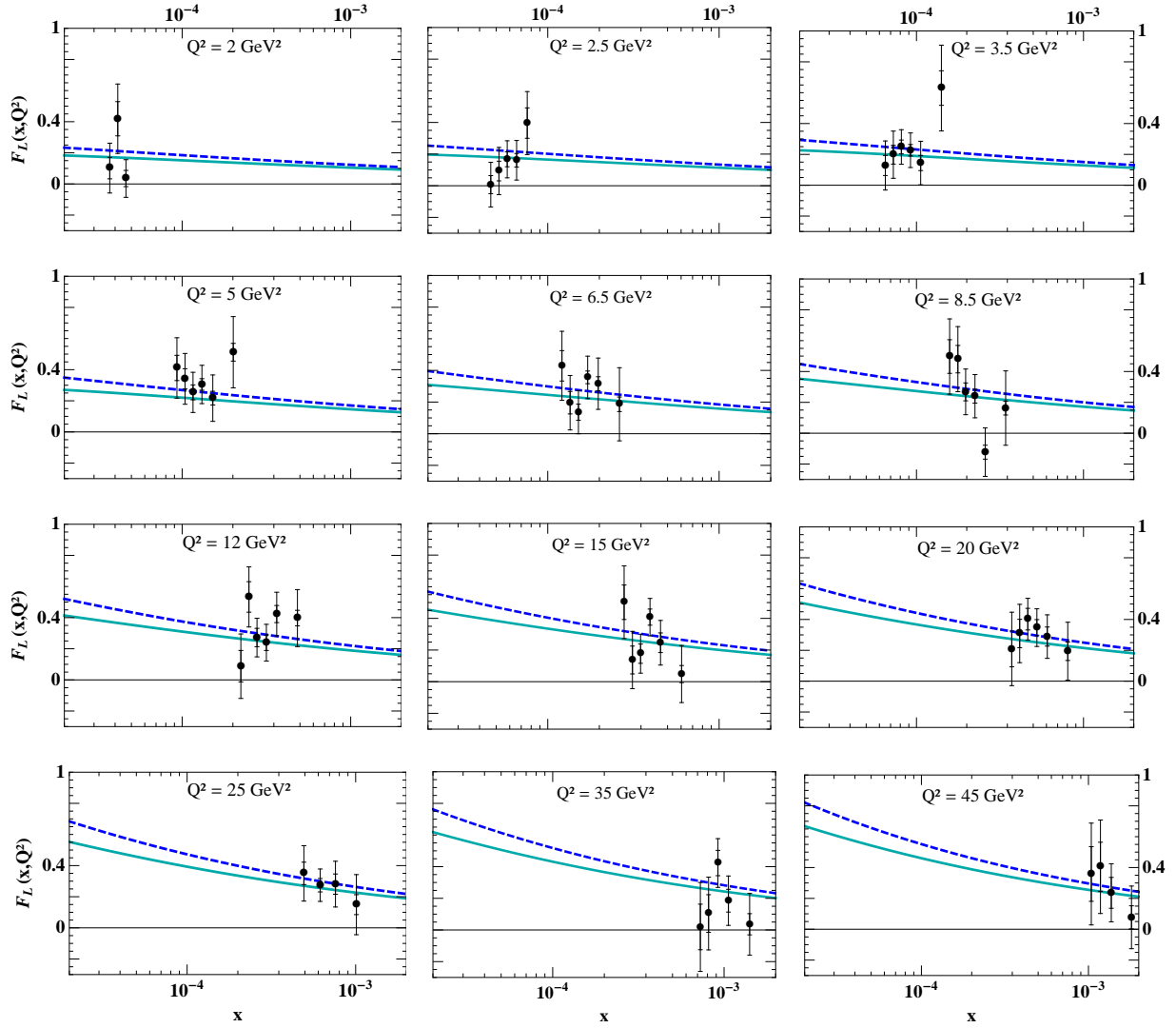
Figure 4: Fit to F_L with the LO photon impact factor (solid lines) and the improved one (dashed lines). The experimental data are taken from [19].
