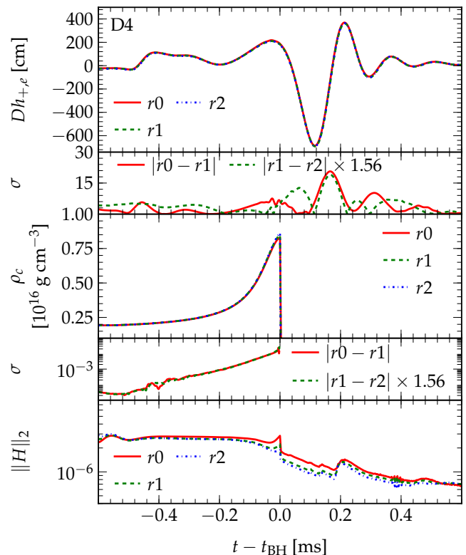
FIG. 14. Rotating neutron star collapse: convergence analysis of the “+” polarization of the GW strain Dh_{+,e} as emitted in the equatorial plane and extracted via CCE (top two panels), central density \rho_c evolution (next two panels), and L_2 -norm of the Hamiltonian constraint \|H\|_2 (bottom panel). The differences in Dh_{+,e} and \rho_c between medium and high resolution are scaled for second-order convergence. At t - t_{\text{BH}} = 0 , the density drops to zero due to hydrodynamic excision within the horizon. The L_2 -norm of the Hamiltonian constraint (bottom panel) does not converge initially due to numerical artifacts from the initial data solver, however, later converges at second-order during black hole formation t - t_{\text{BH}} \simeq 0 and black hole ring-down t - t_{\text{BH}} > 0 . The convergence study is performed using cell-centered AMR with ePPM.
