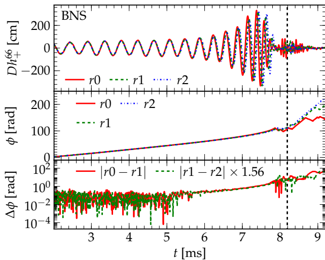
FIG. 21. Binary neutron stars: Phase convergence of the (\ell, m) = (6, 6) mode of the GW strain Dh . The top panel shows the “+” polarization component Dh_+^{66} , and the panel below shows the phase \phi , for low r0 , medium r1 , and high r2 resolutions. The bottom panel shows the phase differences between low and medium, and medium and high resolutions, scaled for second-order convergence. Convergence is maintained throughout inspiral and merger. In the ring-down phase, the coarsest resolution r0 is insufficient to accurately resolve this mode, and the results cease to converge properly. The vertical line indicates appearance of an apparent horizon in the high resolution simulation.
