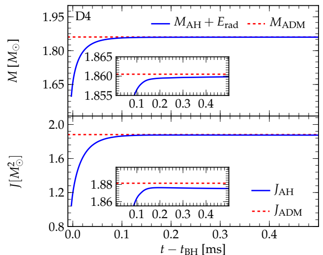
FIG. 16. Rotating neutron star collapse: we show the total ADM mass M_{\text{ADM}} (top panel; red dashed line) and the mass of the apparent horizon M_{\text{AH}} plus energy radiated in GWs E_{\text{rad}} as a function of time (blue straight line). The total ADM angular momentum J_{\text{ADM}} of the spacetime (red dashed line), and the angular momentum J_{\text{AH}} as measured on the apparent horizon (blue straight line) is shown in the bottom panel. The inset plots show a close-up of the time evolution of M_{\text{AH}} + E_{\text{rad}} and J_{\text{AH}} . As all matter becomes trapped in the event horizon, both, M_{\text{AH}} + E_{\text{rad}} and J_{\text{AH}} , quickly asymptote to the conserved ADM values of the spacetime. Due to systematic (atmosphere) and numerical errors, the asymptoted values do not agree with the initial ADM values. Note that the mass radiated in GWs is negligible compared to the total mass of the black hole and thus barely contributes to M_{\text{AH}} + E_{\text{rad}} . No angular momentum is radiated in GWs. The results are shown for resolution r2 using cell-centered AMR with ePPM.
