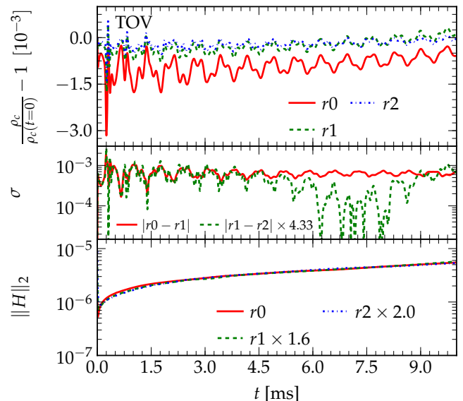
FIG. 6. Unperturbed TOV star: normalized central density \rho_c(t)/\rho_c(t=0) - 1 on the three resolutions r_0 , r_1 , and r_2 (top panel), difference in normalized central density between low and medium resolutions, and medium and high resolution (center panel), and the L_2 -norm of the Hamiltonian constraint \|H\|_2 on all three resolutions (bottom panel). As the resolution is increased, the amplitude of the central density oscillations, the offset, and the slope decrease as expected. The differences in resolutions of the central density are scaled for second-order convergence. The L_2 -norms of the Hamiltonian constraint \|H\|_2 are scaled for first-order convergence. The resolution study is performed using cell-centered AMR and ePPM.
