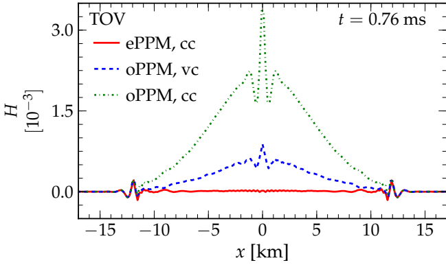
FIG. 25. TOV star (from Sec. III A): the effect of original PPM (oPPM) versus enhanced PPM (ePPM) on the Hamiltonian constraint as a function of x at time t = 0.76 ms. on cell-centered (cc) and vertex-centered (vc) AMR grids. The star’s radius is R_e = 14.16 km. The original PPM results in large constraint violations on the cell-centered grid. The enhanced PPM clearly outperforms oPPM. For ePPM, the error is dominated by the first-order error at the neutron star surface, where the scheme reduces to first order.
