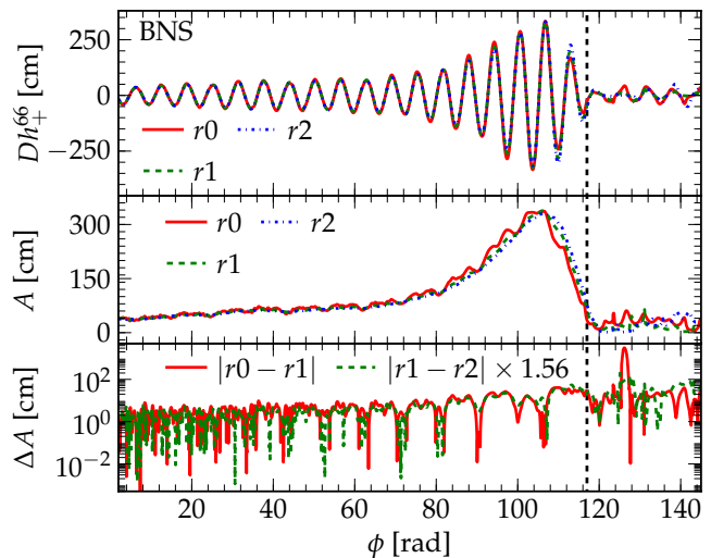
FIG. 22. Binary neutron stars: Amplitude convergence of the (\ell, m) = (6, 6) mode of the GW strain Dh = Dh(\phi) as a function of phase \phi . The top panel shows the “+” polarization component Dh_+^{66}(\phi) , and the panel below shows the amplitude A(\phi) , for low ( r0 ), medium ( r1 ), and high ( r2 ) resolutions. The bottom panel shows the amplitude differences between low and medium, and medium and high resolutions, scaled for second-order convergence. Convergence is maintained throughout inspiral and merger. In the ring-down phase, however, the coarsest resolution r0 is insufficient to accurately resolve this mode, and the results cease to properly converge. The vertical line indicates appearance of an apparent horizon in the high resolution simulation.
