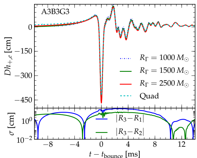
FIG. 13. The GW strain extracted Dh_{+,e} from the rotating stellar collapse model A3B3G3 (upper panel). We show the strain extracted via CCE from different worldtube locations R_\Gamma = 1000 M_\odot , R_\Gamma = 1500 M_\odot , and R_\Gamma = 2500 M_\odot , as well as the strain computed via the quadrupole formula. Larger CCE worldtube radii permit lower FFI cut-off frequencies without introducing unphysical drifts in the GW strain. All waveforms extracted via CCE are in good agreement to within a few percent with the waveform computed via the quadrupole formula. The lower panel shows the differences in strain amplitude of the inner extraction radii to the outermost extraction radius. The differences converge as the extraction radius is increased. The comparison is done using baseline resolution r1 .
