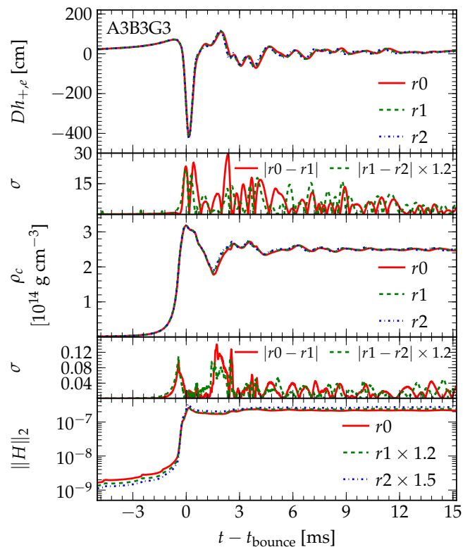
FIG. 11. Stellar collapse: The GW strain Dh_{+,e} extracted via the quadrupole formula (upper panel), the central density \rho_c (third panel from the top), and the L_2 -norm of Hamiltonian constraint \|H\|_2 , all on the three resolutions r_0 , r_1 , and r_2 . The panels directly below the top panel and the third panel from the top show the difference in strain and central density between low and medium resolutions, and medium and high resolutions. The differences are scaled for second-order convergence. The L_2 -norm of Hamiltonian constraint is scaled for first-order convergence. Before core bounce, the constraint exhibits second order convergence. After shock formation, the convergence rate is reduced to first order. The convergence study is performed using cell-centered AMR and ePPM.
