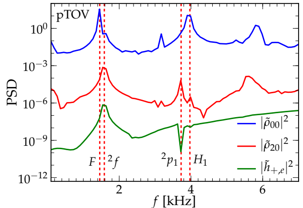
FIG. 10. Perturbed TOV star: Power spectrum of \rho_{00} , \rho_{20} and h_{+,e} (individually scaled for better visibility), and the first few fundamental neutron star oscillation modes (vertical lines) computed in [36].
