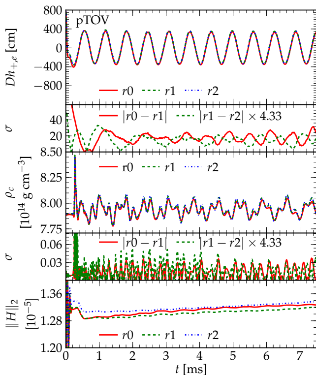
FIG. 8. Perturbed TOV star: the top panel shows the “+” polarization of the GW strain Dh_{+,e} as emitted in the equatorial plane and rescaled by distance D for the three resolutions r_0 , r_1 , and r_2 . The waveforms are computed with CCE. In the panel below, we show the differences in GW strain between r_0 and r_1 , and r_1 and r_2 , where the latter is rescaled for second-order convergence. In the third panel from the top, we show the absolute central density evolution \rho_c(t) for the three resolutions. Below, we show the differences in central density scaled for second-order convergence. In the bottom panel, we show the L_2 -norms of the Hamiltonian constraint \|H\|_2 . Since the initial data for the perturbed case are not constraint satisfying, the constraints do not exhibit clean convergence. The convergence study is performed using cell-centered AMR and ePPM.
