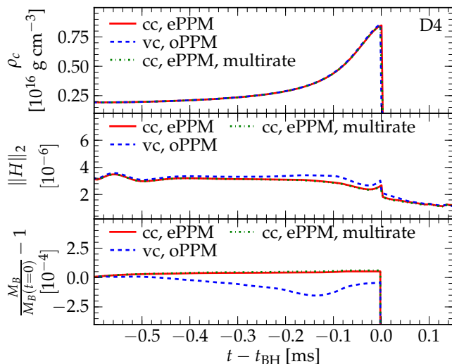
FIG. 15. Rotating neutron star collapse: we compare vertex-centered (vc) AMR and oPPM reconstruction with cell-centered (cc) AMR and ePPM reconstruction. The latter setup is also shown using multirate RK time integration. The top panel compares the central density evolution profile \rho_c(t) . The center panel compares the evolution of the L_2 -norm of the Hamiltonian constraint \|H\|_2 . The bottom panel compares the conservation of baryonic mass M_B . The setup “vc, oPPM” produces slightly larger violations in the Hamiltonian constraints, especially in the late collapse phase shortly before the black hole forms. Due to refluxing, the cell-centered case exhibits much better conservation of baryonic mass. Multirate RK time integration does not lead to different results. The comparison is done using baseline resolution r1 .
