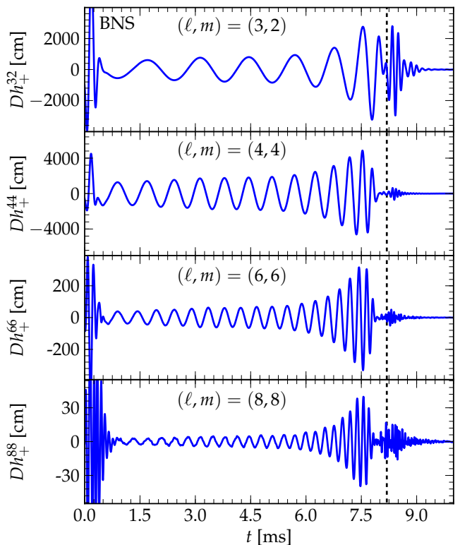
FIG. 20. Binary neutron stars: GW modes (\ell, m) = (3, 2), (4, 4), (6, 6), (8, 8) of “+” polarization of the strain Dh unambiguously extracted via CCE. The waveforms are shown for high resolution simulation r2 . The vertical line indicates the time of appearance of an apparent horizon. Following appearance of an apparent horizon, a black hole ring-down signal is visible.
