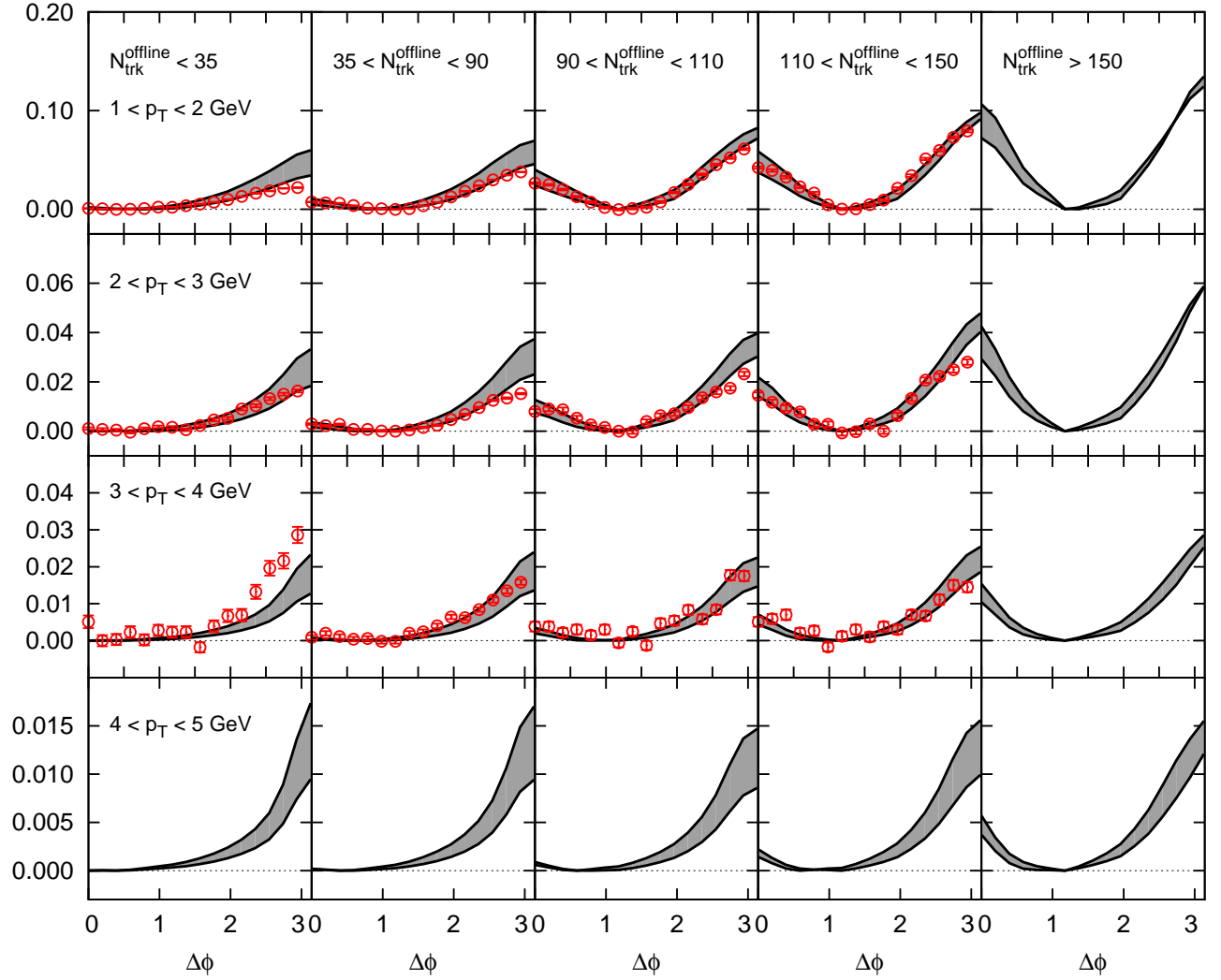
FIG. 4. Correlated yield 1/N_{\text{trig}} d^2 N / d\Delta\phi after ZYAM as a function of \Delta\phi integrated over 2 \leq |\Delta\eta| \leq 4 for several multiplicity bins, each for a particular range in p_T^{\text{trig}} = p_T^{\text{asc}} . The data points are from the CMS collaboration [14]. The theoretical curves are the result of adding the glasma and BFKL contributions with the band representing the variation in results when changing the K-factors from K_{\text{glasma}} = 1.5, K_{\text{bfl}} = 1.65 to K_{\text{glasma}} = 1.95, K_{\text{bfl}} = 0.9 . The results for the different multiplicity windows correspond (from left to right) to: Q_0^2(\text{proton})=0.168 \text{ GeV}^2, N_{\text{part}}^{\text{Pb}} = 3 ; Q_0^2(\text{proton})=0.336 \text{ GeV}^2, N_{\text{part}}^{\text{Pb}} = 6 ; Q_0^2(\text{proton})=0.336 \text{ GeV}^2, N_{\text{part}}^{\text{Pb}} = 12 ; Q_0^2(\text{proton})=0.504 \text{ GeV}^2, N_{\text{part}}^{\text{Pb}} = 14 ; Q_0^2(\text{proton})=0.504 \text{ GeV}^2, N_{\text{part}}^{\text{Pb}} = 22 . Predictions are shown for very large multiplicity windows and higher values of p_T^{\text{trig}} = p_T^{\text{asc}} .
