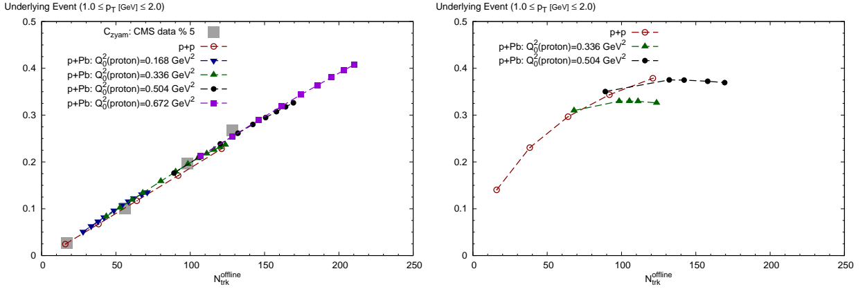
FIG. 6. Left: The underlying glasma event per trigger (equivalent to C_{zyam} in [14]) as a function of N_{\text{trk}}^{\text{offline}} for 1 \leq p_T^{\text{trig}}, p_T^{\text{asc}} \leq 2 . The large grey squares are the experimental values of C_{ZYAM} divided by a factor 5. All other symbols denote theory computations with a fixed initial scale Q_0 in the proton and varying values of N_{\text{part}}^{\text{pPb}} . Right: The underlying BFKL event per trigger for Q_0^2 = 0.336 \text{ GeV}^2 and Q_0^2 = 0.504 \text{ GeV}^2 and varying values of N_{\text{part}} . See text for discussion.
