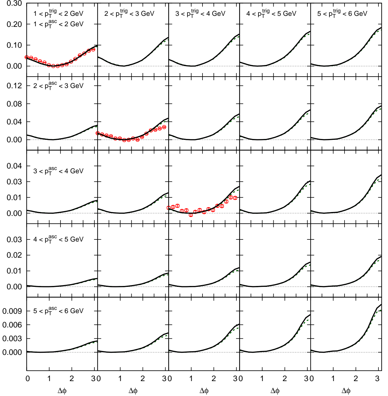
FIG. 5. Correlated yield 1/N_{\text{trig}} d^2 N / d\Delta\phi after ZYAM as a function of \Delta\phi integrated over 2 \leq |\Delta\eta| \leq 4 for the most central multiplicity bin N_{\text{trk}}^{\text{offline}} \geq 110 . The data points are from the CMS collaboration [14] and have currently only been provided for the diagonal components p_T^{\text{trig}} \sim p_T^{\text{asc}} of the correlation matrix. The curves are obtained by adding the glasma contributions ( K = 1.5 ) and the BFKL contribution ( K = 1.65 ). The solid black curve is the result for Q_0^2(\text{proton}) = 0.504 \text{ GeV}^2 on N_{\text{part}}^{\text{Pb}} = 14 and the dashed green is for Q_0^2(\text{proton}) = 0.336 \text{ GeV}^2 on N_{\text{part}}^{\text{Pb}} = 16 .
