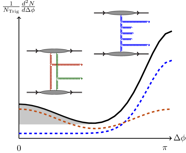
FIG. 1. Anatomy of di-hadron correlations. The glasma graph is on the left and its schematic contribution to the double inclusive cross-section is shown as the dashed orange curve. On the right is the back-to-back graph and the shape of its yield (dashed blue curve). The grey blobs denote emissions all the way from beam rapidities to those of the triggered gluons. The solid black curve represents the sum of contributions from glasma and back-to-back graphs. The shaded region represents the Associated Yield (AY) calculated using the zero-yield-at-minimum (ZYAM) procedure. Figure from ref. [9].
