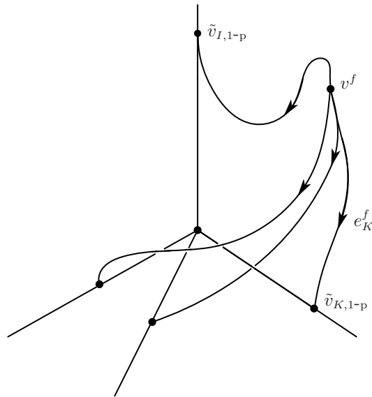
FIGURE (8): The graph underlying a causal completion of the 1- past of c .
