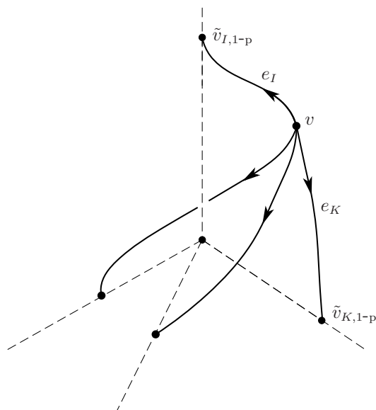
FIGURE (6): The future graph \gamma_{1-p}^{f_0} of \gamma_{1-p}(c) in c .
