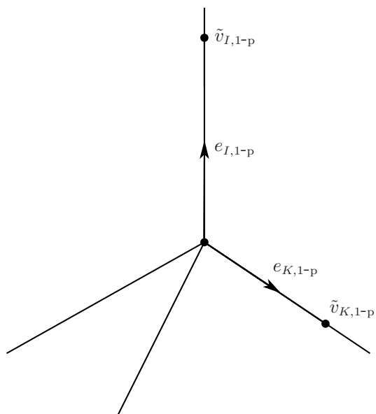
FIGURE (5): The 1-past \gamma_{1-p}(c) .
