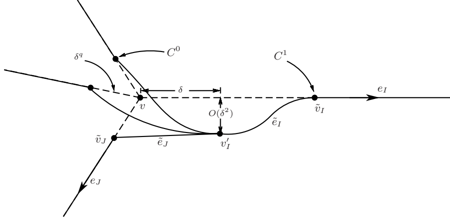
FIGURE (1): A sample deformation produced by a single Hamiltonian constraint action at a non-degenerate vertex v along the edge e_I . The dashed edges emanating from the original vertex v are now only charged in two of the three U(1) factors, but v'_I is expected to be, generically, non-degenerate. With respect to the coordinate system fixed at v , v'_I is located a distance \delta from v along e_I and displaced off of e_I a distance O(\delta^2) . \tilde{e}_I and e_I share a tangent at \tilde{v}_I , but \tilde{e}_J and e_J do not share a tangent. All of the \tilde{e}_{J \neq I} have tangents at v'_I which are ‘bunched’ and lie within a cone of apex angle O(\delta^{q-1}) .
