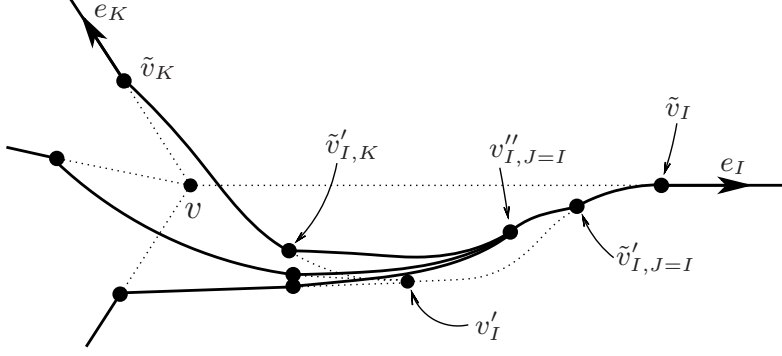
FIGURE (3): Sample deformation produced by two successive singular diffeomorphisms along the edge e_I . Here the dotted lines indicate the position of the graph before the deformations; these are not part of the resulting graph. The structure of the deformations is similar to that produced by the action of two successive Hamiltonian-type deformations, except that now the original vertices v and v'_I are charged in no copies of U(1) ; the dotted edges are not actually there. Note that the kink structure is the same as for the Hamiltonian deformations: The edge e_I is C^1 at \tilde{v}_I and \tilde{v}'_{I,J=I} , but all other edges are C^0 at the various \tilde{v}_K and \tilde{v}'_{I,K} .
