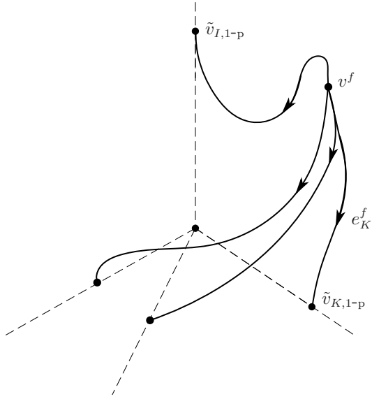
FIGURE (7): A future graph \gamma_{1-p,c}^f of \gamma_{1-p}(c) with respect to c .
