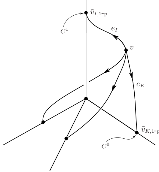
FIGURE (4): The original graph \gamma(c) .
