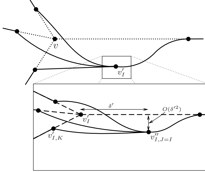
FIGURE (2): Detail of the deformation generated by two successive Hamiltonian actions, in this case along the same edge J = I . Here \delta' \ll \delta .
