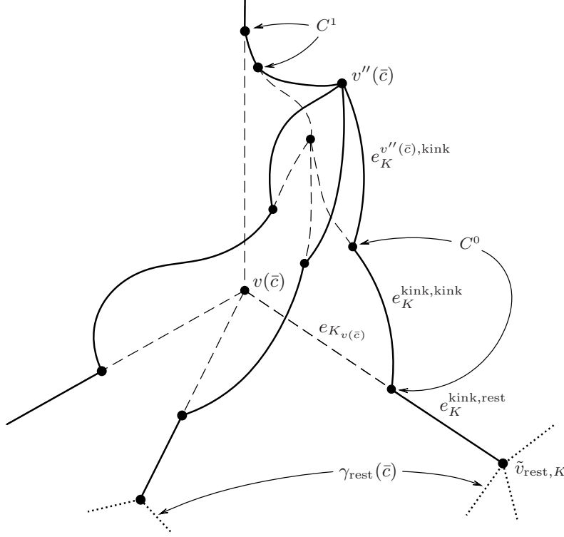
FIGURE (9): The result of a double singular diffeomorphism action on \bar{c} labeled corresponding to definitions used in this section.
