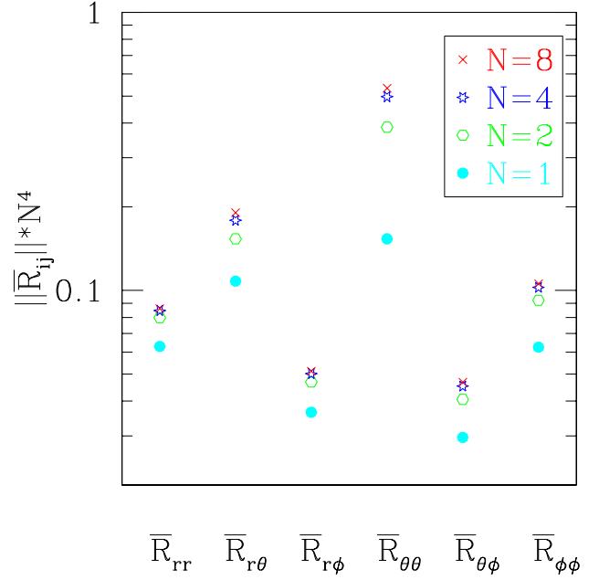
FIG. 10: Values of the norms of the components of the Ricci tensor, \|R_{ij}\| , for the flat metric (A1) with functions (A6), evaluated using grid sizes (16N, 8N, 16N) for N = 1, 2, 4 and 8. All values are rescaled with N^4 , so that the convergence of these results indicates fourth-order convergence of our implementation.
