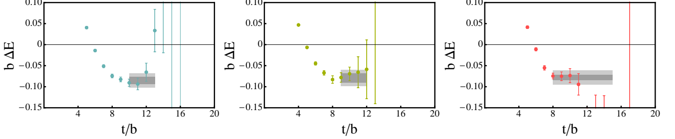
FIG. 14: EMPs associated with a |\mathbf{P}| = 0 J^\pi = 0^+ {}^4\text{He} correlation function computed with the 24^3 \times 48 (left), 32^3 \times 48 (center) and 48^3 \times 64 (right) ensembles. The inner (darker) shaded region corresponds to the statistical uncertainty of the extracted energy, while the outer (lighter) shaded region corresponds to the statistical and fitting systematic uncertainties combined in quadrature.
