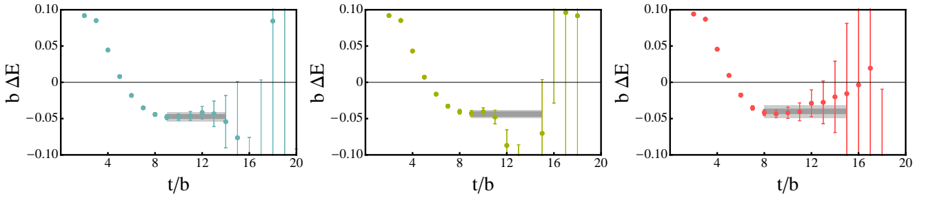
FIG. 12: The EMPs associated with one J^\pi = \frac{3}{2}^+ \frac{3}{\Sigma}\text{He} correlation function computed with the 24^3 \times 48 (left), 32^3 \times 48 (center) and 48^3 \times 64 (right) ensembles, with momentum |\mathbf{P}| = 0 . The inner (darker) shaded region corresponds to the statistical uncertainty of the extracted energy, while the outer (lighter) shaded region corresponds to the statistical and fitting systematic uncertainties combined in quadrature.
