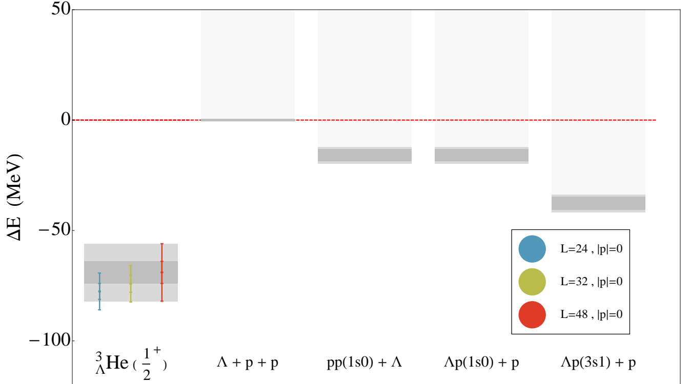
FIG. 10: The EMPs associated with one J^\pi = \frac{1}{2}^+ \frac{3}{\Lambda}\text{He} ( \frac{3}{\Lambda}\text{H} and nn\Lambda ) correlation function computed with the 24^3 \times 48 (left), 32^3 \times 48 (center) and 48^3 \times 64 (right) ensembles, with momentum |\mathbf{P}| = 0 . The inner (darker) shaded region corresponds to the statistical uncertainty of the extracted energy, while the outer (lighter) shaded region corresponds to the statistical and fitting systematic uncertainties combined in quadrature.
