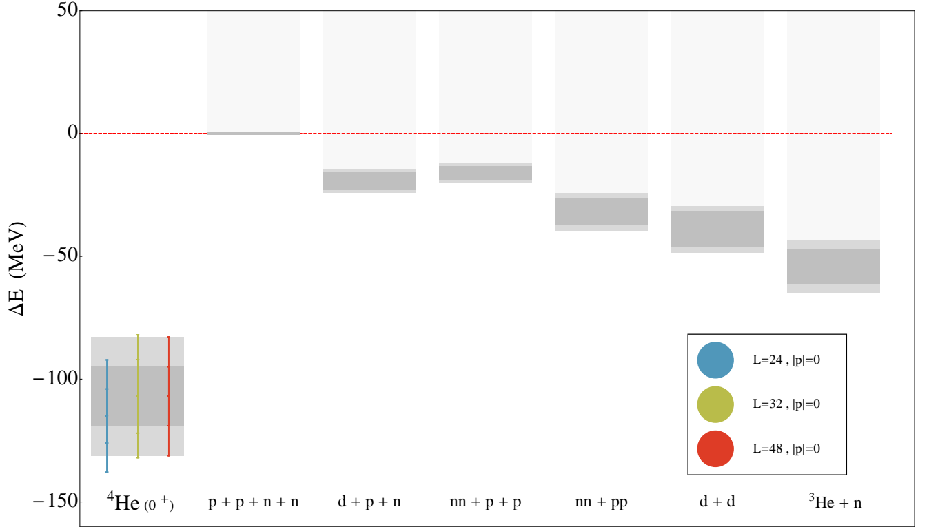
FIG. 15: The bound-state energy levels in the J^\pi = 0^+ {}^4\text{He} sector. The points and their associated uncertainties correspond to the energies of the states extracted from the correlation functions with the quantum numbers of the ground state of {}^4\text{He} . The locations of the energy-levels associated with non-interacting \text{N-}{}^3\text{He} , d-d, di-neutron-di-neutron, di-neutron-N-N, d-N-N and N-N-N-N continuum states, determined from the two-body binding energies given in Table VII and the three-body energies given in eq. (9), are shown.
