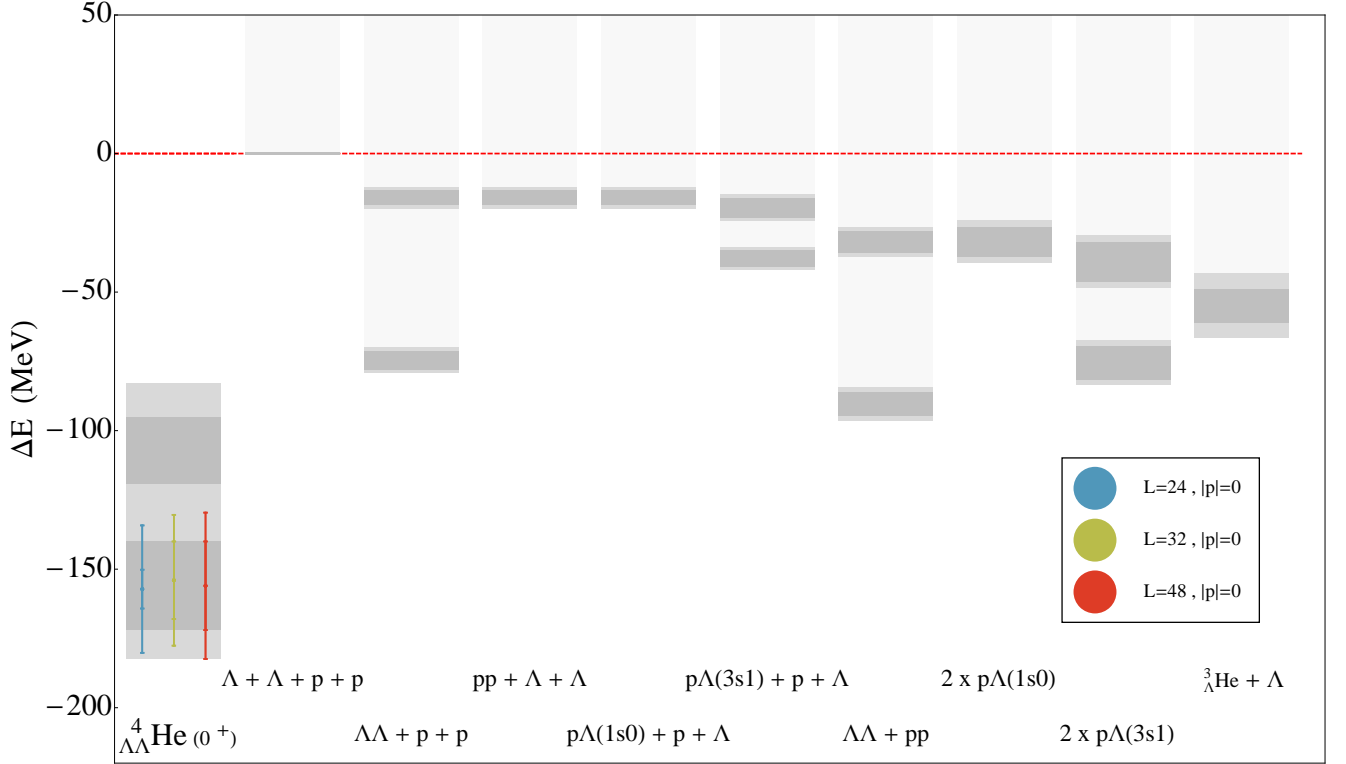
FIG. 17: The bound-state energy levels in the J^\pi = 0^+ {}^4_{\Lambda\Lambda}\text{He} ( {}^4_{\Lambda\Lambda}\text{H} and nn\Lambda\Lambda ) sector. The points and their associated uncertainties correspond to the energies of the states extracted from the correlation functions with the quantum numbers of the ground state of {}^4_{\Lambda\Lambda}\text{He} . The excited state of the {}^4_{\Lambda\Lambda}\text{He} , in the \mathbf{28} , has the same energy as the ground state of {}^4\text{He} . The locations of the energy-levels associated with non-interacting \Lambda - {}^3_{\Lambda}\text{He} , N\Lambda - N\Lambda , H-dibaryon-di-neutron, N\Lambda - N - \Lambda , di-neutron- \Lambda - \Lambda , H-dibaryon- N - N , and \Lambda - \Lambda - N - N continuum states, determined from the two-body binding energies given in Table VII and the three-body energies given in eq. (9) and eq. (12), are shown.
