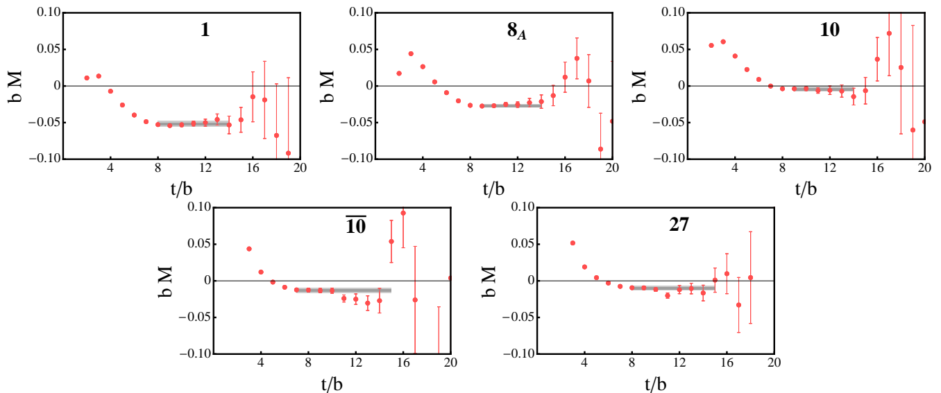
FIG. 4: EMPs associated with |\mathbf{P}| = 0 two-baryon correlation functions computed with the 48^3 \times 64 ensemble. The inner (darker) shaded region corresponds to the statistical uncertainty of the extracted energy, while the outer (lighter) shaded region corresponds to the statistical and fitting systematic uncertainties combined in quadrature. The time-extent of each band corresponds to the choice of the fitting interval for each correlation function. From left to right, the top row corresponds to the \mathbf{1} , \mathbf{8}_A , \mathbf{10} SU(3) irreps (corresponding to the H-dibaryon, I = 0 N\Xi in the {}^3S_1 - {}^3D_1 coupled channels and n\Sigma^- in the {}^3S_1 - {}^3D_1 coupled channels, respectively), and the bottom row corresponds to the \overline{\mathbf{10}} and \mathbf{27} (corresponding to the deuteron and di-neutron, respectively).
