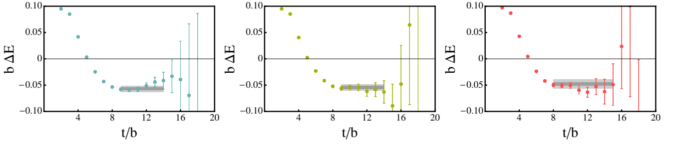
FIG. 10: The EMPs associated with one J^\pi = \frac{1}{2}^+ \frac{3}{\Lambda}\text{He} ( \frac{3}{\Lambda}\text{H} and nn\Lambda ) correlation function computed with the 24^3 \times 48 (left), 32^3 \times 48 (center) and 48^3 \times 64 (right) ensembles, with momentum |\mathbf{P}| = 0 . The inner (darker) shaded region corresponds to the statistical uncertainty of the extracted energy, while the outer (lighter) shaded region corresponds to the statistical and fitting systematic uncertainties combined in quadrature.
