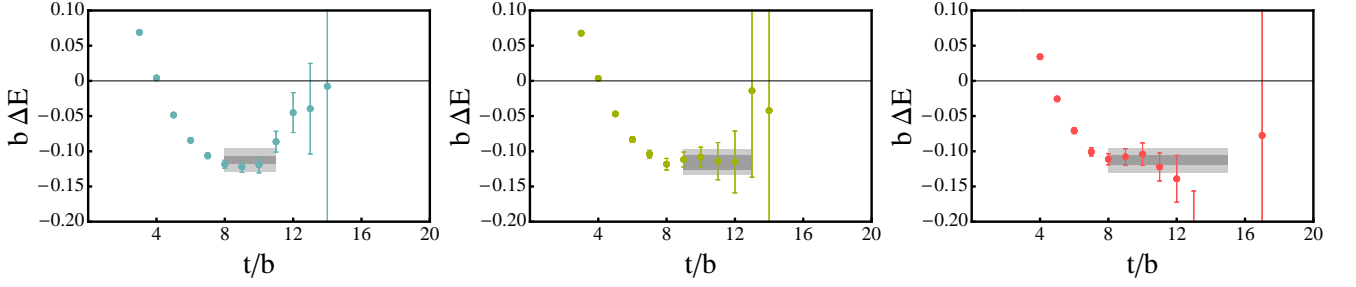
FIG. 16: The EMPs associated with one of the eight J^\pi = 0^+ {}^4_{\Lambda\Lambda}\text{He} correlation functions computed with the 24^3 \times 48 (left), 32^3 \times 48 (center) and 48^3 \times 64 (right) ensembles, with momentum |\mathbf{P}| = 0 . The inner (darker) shaded region corresponds to the statistical uncertainty of the extracted energy, while the outer (lighter) shaded region corresponds to the statistical and fitting systematic uncertainties combined in quadrature.
