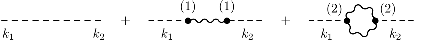
FIG. 1. Leading diagrams for \langle \zeta^2 \rangle , with the vertices labelled as in (26).
