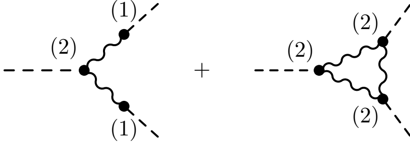
FIG. 2. Leading diagrams for \langle \zeta^3 \rangle , with the vertices labelled as in (26).
