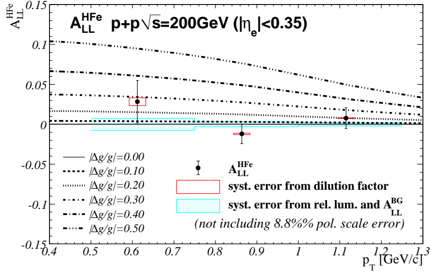
(a) Expected A_{LL}^{\text{HFe}} for several |\Delta g/g| .
