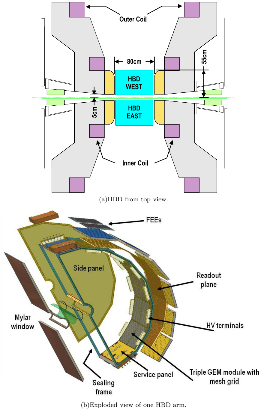
FIG. 2: (color online) (a) Top view of the HBD showing the location of the HBD in the central magnet. (b) Exploded view of one HBD arm, which is half of the total HBD. \text{CF}_4 gas is filled in the volume as the Čerenkov light radiator.
