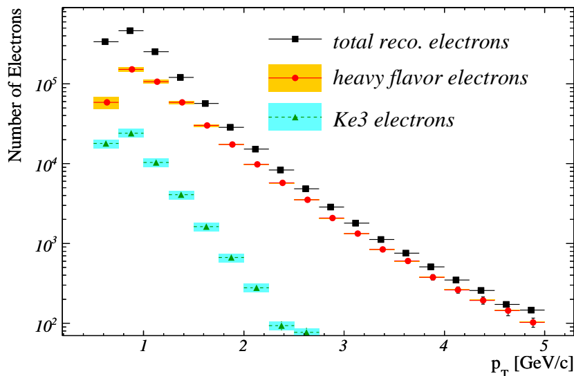
FIG. 9: (color online). Heavy flavor electron yield spectrum. The black square points represent the total number of the reconstructed electrons after applying the eID-Cut and the npe-Cut. The red circle points represent the estimated yield of the heavy flavor electrons. The yellow bands represent the systematic uncertainties for the heavy flavor electron yield. The green triangle points with dashed lines represent the estimated K_{e3} contribution with systematic uncertainties shown by light-blue bands.
