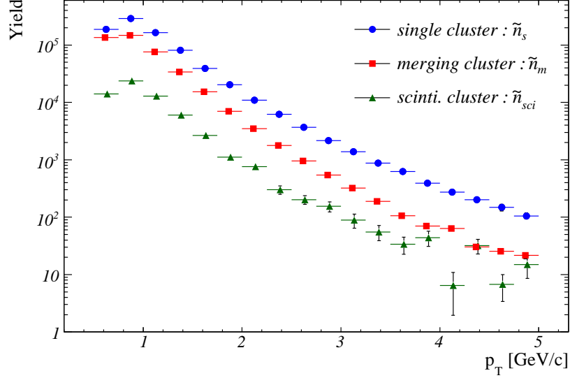
FIG. 6: (color online). Yield spectra of HBD clusters after applying the eID-Cut and the npe-Cut estimated from the HBD cluster charge fitting. The plot shows the spectrum for the single clusters ( \tilde{n}_s , blue circle), the spectrum for the merging clusters ( \tilde{n}_m , red square) and the spectrum for the scintillation clusters ( \tilde{n}_{sci} , green triangle). The error bars represent fitting uncertainties.
