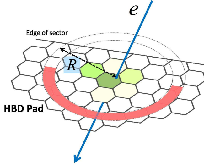
FIG. 7: (color online). A half of an annular region around the reconstructed electron track on the HBD for the definition of q_{\text{ring}} . The inner and outer radii of the annular region are 7.0 cm and 8.0 cm respectively. The direction of the half region is determined as the opposite side to the edge of the HBD sector to avoid inefficiency around the edge.
