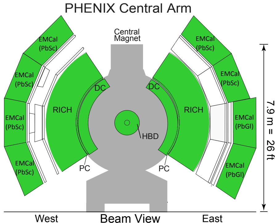
FIG. 1: (color online) Beam view (at z = 0 ) of the PHENIX central arm detectors in 2009. See text for details.
