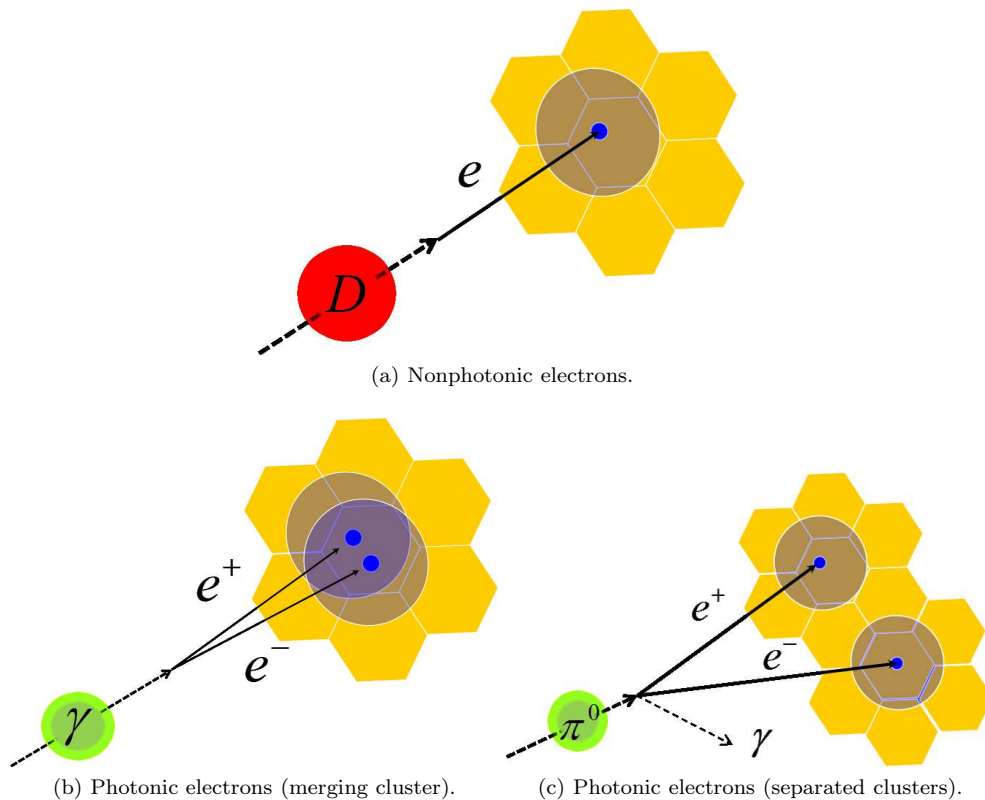
FIG. 4: (color online) Responses of the HBD for (a) nonphotonic electrons and (b,c) photonic electrons. (b) Most of the photonic electron pair create merging clusters. (c) However, the photonic electrons with large opening angles create separated clusters.
