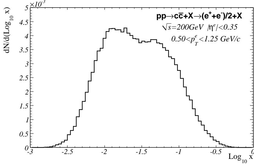
FIG. 14: (color online). Bjorken x distributions of gluons contributing the heavy flavor electron production with momentum ranging 0.50 < p_T < 1.25 GeV/ c obtained from PYTHIA simulation. The distribution is normalized with respect to the number of total generated charmed hadrons.
