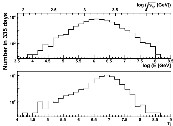
FIG. 4. Top: The true total primary energy of Sibyll simulated shower events that pass all selection criteria. The equivalent center of mass energy for proton-proton collisions is shown on the top axis. Bottom: The pseudorapidity of the muon with the maximum transverse separation in Sibyll simulated shower events that pass all selection criteria.
