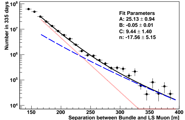
FIG. 11. (Color online). The LS muon data distribution at sea level, along with the best fit parameters for the function described in the text. The exponential part of the fit is plotted as a dotted red line and the power law is shown as a dashed blue line.
