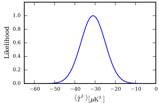
FIG. 3. Likelihood of the skewness measurement described in the text (with Gaussian statistics assumed).
