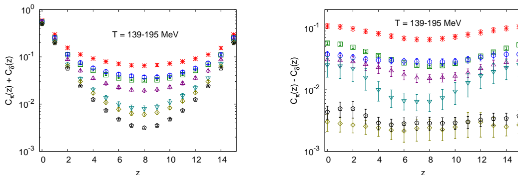
FIG. 10. (Left) The sum of the spatial \pi and the \delta correlators. The temperature increases from T = 139 MeV to 195 MeV as one moves downward along the y -axis. (Right) The difference C_\pi(z) - C_\delta(z) . The temperatures are identified by the same symbols as in the sum. The monotonic decreasing behavior seen with increasing temperature in the left panel is not seen for the highest temperatures in the right panel where the T = 195 MeV data lies slightly above that for T = 186 . However, this apparent diminished rate of decrease with increasing temperature may be an artifact of insufficient statistics since the statistical errors on this signal, which, as discussed in Sec. VIC, arises from infrequent spikes in the data, may be underestimated.
