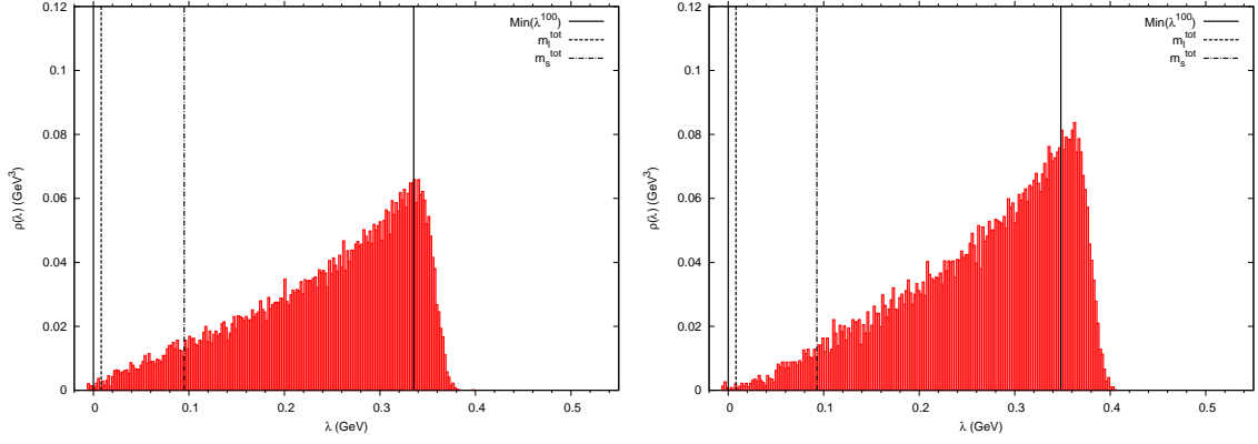
FIG. 13. Renormalized Dirac spectrum 168 MeV (left) and 177 MeV (right).
