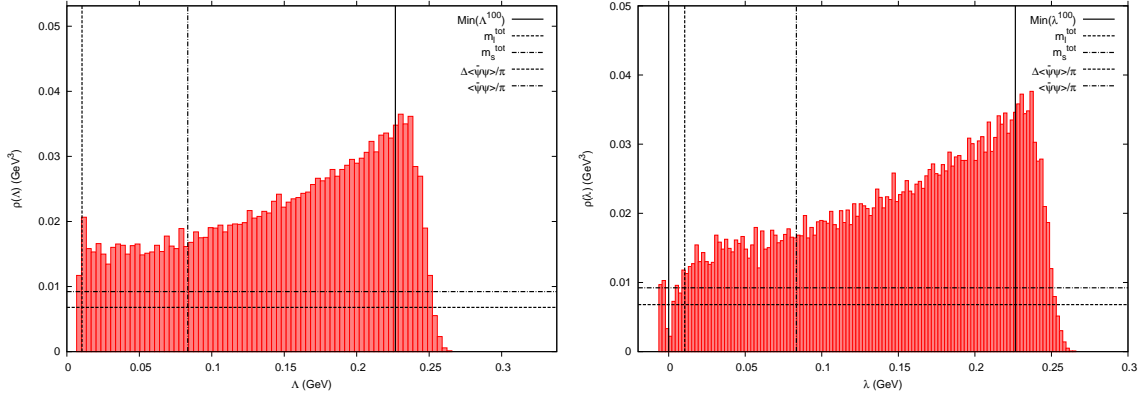
FIG. 4. Histogram of the spectrum of eigenvalues \Lambda of the hermitian DWF Dirac operator normalized in the \overline{\text{MS}} scheme at the scale \mu = 2 GeV (left). These eigenvalues are calculated on the zero-temperature ensemble labeled #11. The right hand panel shows a histogram of the eigenvalues \lambda = \sqrt{\Lambda^2 - (m_f + m_{\text{res}})^2} from which the quark mass has been removed. In the this panel, the region \lambda > 0 shows those values for which \Lambda^2 > (m_f + m_{\text{res}})^2 , i.e. , \lambda is purely real, a condition that should be obeyed in the continuum limit. The region \lambda < 0 shows those eigenvalues with \Lambda^2 < (m_f + m_{\text{res}})^2 , i.e. , \lambda pure imaginary, plotted on the negative part of the x-axis as \lambda = -|\sqrt{\Lambda^2 - (m_f + m_{\text{res}})^2}| . These unphysical values give a visible measure of the finite lattice spacing distortions to the region of small \lambda > 0 .
