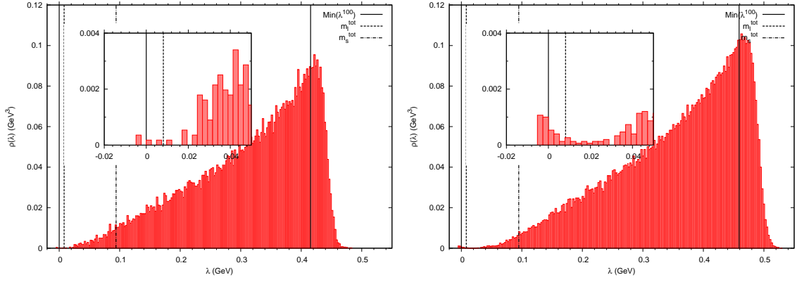
FIG. 14. Renormalized Dirac spectrum 186 MeV (left) and 195 MeV (right).
