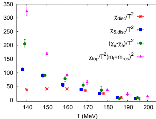
FIG. 9. The disconnected scalar (chiral) and pseudo-scalar susceptibilities plotted versus temperature as crosses and squares respectively. The circles show the U(1)_A -breaking difference \chi_\pi - \chi_\delta , which in the chiral limit will become equal to both disconnected susceptibilities above T_c . Finally the triangles represent the topological susceptibility divided by the square of the total bare quark mass, m_f + m_{\text{res}} , a combination which should equal the pseudo-scalar susceptibility at all temperatures, as in Eq. 43. The large discrepancy between \chi_{\text{top}}/(m_f + m_{\text{res}})^2 and \chi_{5,\text{disc}} is believed to arise from large lattice artifacts in the determination of \chi_{\text{top}} as discussed below and in Appendix D
