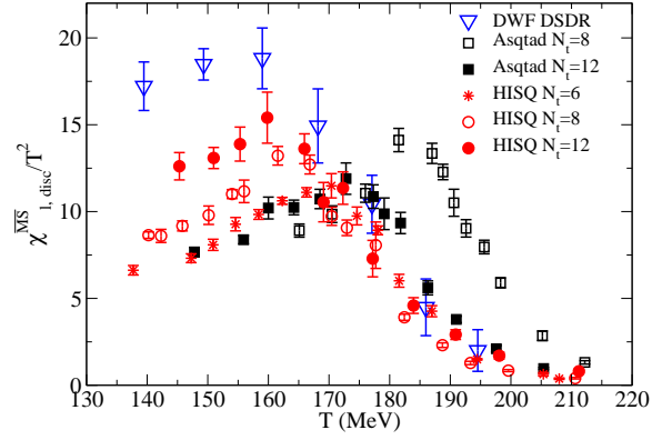
FIG. 7. In the upper panel, the unrenormalized, disconnected chiral susceptibility for DWF DSDR L_s = 32, 48 is compared with the DWF results with L_s = 96 . In the lower panel, the renormalized chiral susceptibilities, converted to the \overline{\text{MS}} scheme are compared between the DWF DSDR calculation and the HISQ and asqtad results from the HotQCD Collaboration, corresponding to a pseudo-Goldstone pion mass of 161 and 179 MeV, respectively.
