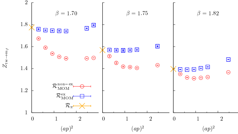
FIG. 3. Plots of the results for the quantity Z_{tw \rightarrow m_f} given in Tabs. IV and VI for each of the three values of \beta that were studied at zero temperature. The single value of \mathcal{R}_\pi is plotted as an “ \times ” in each panel and given the value (pa)^2 = 0 . (The scale on the left-most y -axis applies to all three plots.) As discussed in the text, the discrepancies between \mathcal{R}_{\text{MOM}}^{\text{non-ex}} and \mathcal{R}_{\text{MOM}}^{\text{ex}} are indicative of O((pa)^2) errors, so we use the value of \mathcal{R}_\pi for Z_{tw \rightarrow m_f} .
