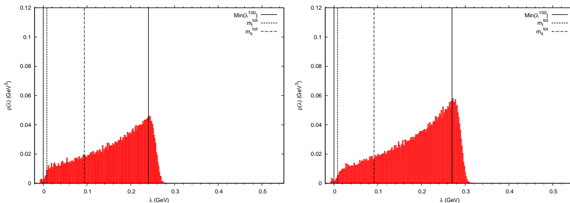
FIG. 12. Renormalized Dirac spectrum 149 MeV L_s = 32 (left) and 159 MeV (right).
