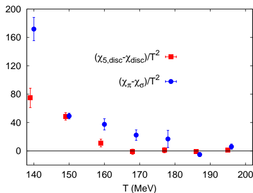
FIG. 8. The SU(2)_L \times SU(2)_R -breaking differences between the disconnected pseudo-scalar and disconnected scalar susceptibilities and between the flavor-triplet pseudo-scalar and flavor singlet scalar susceptibilities.
