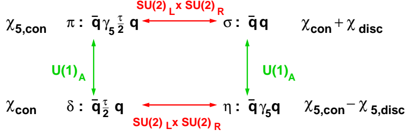
FIG. 5. Symmetry transformations relating scalar and pseudo-scalar mesons in flavor singlet and non-singlet channels.
