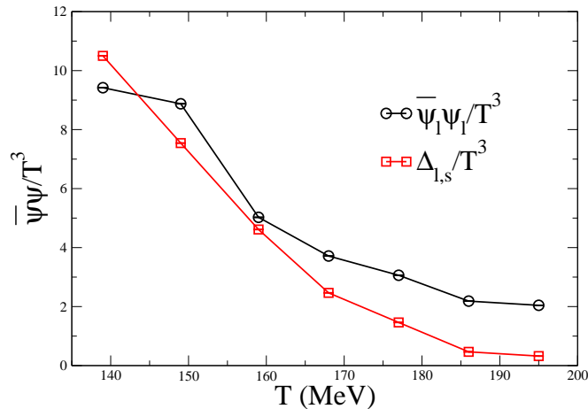
FIG. 6. The light quark chiral condensate, as well as the subtracted chiral condensate plotted as a function of temperature. As discussed in the text, the values plotted for T = 139 and 149 MeV were computed using L_s = 48 while those at higher temperatures used L_s = 32 .
