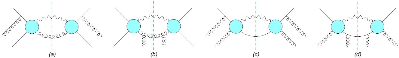
FIG. 2: Double scattering diagrams for q\bar{q} \rightarrow \gamma g (left two) and qg \rightarrow \gamma q (right two): (a) and (c) are for initial-state double scattering, while (b) and (d) are for final-state double scattering. The blobs represent the tree-level diagrams as shown in Fig. 1.
