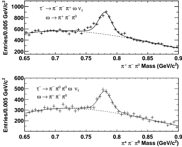
FIG. 4: The fits to the \omega peak in the \pi^+\pi^-\pi^0 invariant mass distributions for \tau^- \rightarrow 2\pi^-\pi^+\omega\nu_\tau and \tau^- \rightarrow \pi^-2\pi^0\omega\nu_\tau decay candidates after all selection criteria are applied. The solid lines represent the fit to the \omega peak and background. The dashed lines show the extrapolation of the background function under the \omega peak.
