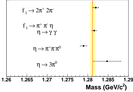
FIG. 3: Compilation of our measurements of the f_1 mass. The solid line is the weighted average and the shaded area is the one-standard-deviation region.
