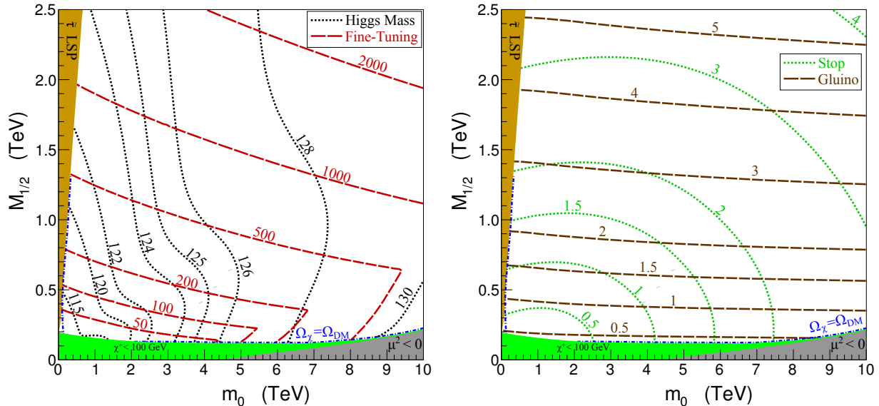
FIG. 4. As in Fig. 2, but for Model B with (x, y) = (\frac{5}{9}, \frac{7}{27}) and weak-scale-unified stops with m_{Q_3}^2(m_W) = m_{U_3}^2(m_W) = \frac{1}{9}m_0^2 .
