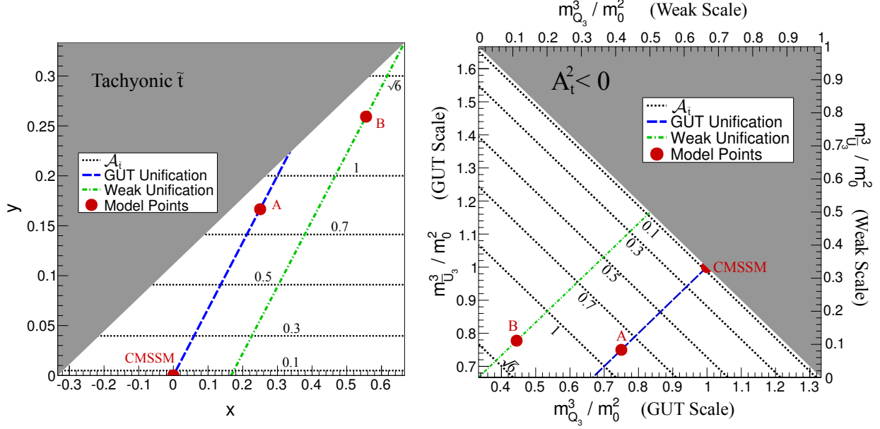
FIG. 1. The model parameter space in the (x, y) plane (left) and in the (m_{Q_3}^2(m_{GUT}), m_{U_3}^2(m_{GUT})) [or alternatively, (m_{Q_3}^2(m_W), m_{U_3}^2(m_W)) ] plane (right). The blue dashed and green dot-dashed lines correspond to the special cases where m_{Q_3}^2 = m_{U_3}^2 at the GUT scale and m_{Q_3}^2 \simeq m_{U_3}^2 at the weak scale, respectively, and red dots correspond to the three models (x, y) = (0, 0) (mSUGRA/CMSSM), (\frac{1}{4}, \frac{1}{6}) , and (\frac{5}{9}, \frac{7}{27}) examined in detail. Black dotted lines of constant stop mixing parameter A_{\tilde{t}} are also shown.
