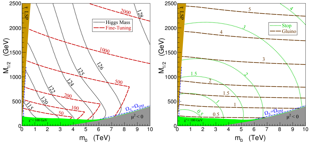
FIG. 3. As in Fig. 2, but for Model A with (x, y) = (\frac{1}{4}, \frac{1}{6}) and GUT-unified stops with m_{Q_3}^2(m_{\text{GUT}}) = m_{U_3}^2(m_{\text{GUT}}) = \frac{3}{4}m_0^2 .
