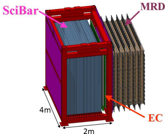
FIG. 4. Schematic view of the SciBooNE detector.
