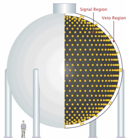
FIG. 3. Schematic view of the MiniBooNE detector.
