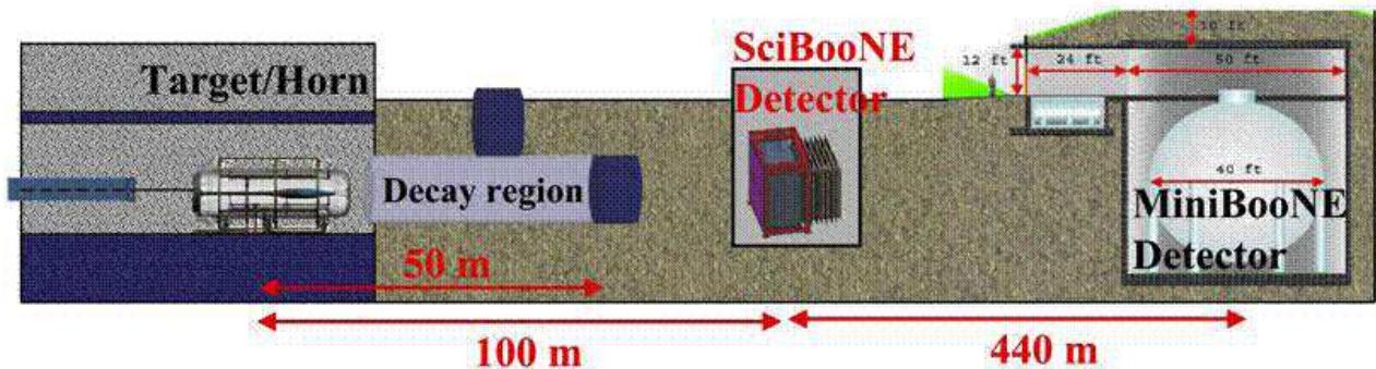
FIG. 1. Schematic view of the BNB from the beryllium target and magnetic horn to the SciBooNE and MiniBooNE detectors.
