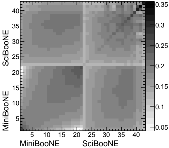
FIG. 10. Bin-wise square root of the total (statistical and systematic errors combined) fractional error matrix \sqrt{\hat{M}_{ij}} = \sqrt{M_{ij}}/\sqrt{N_i N_j} , where M_{ij} is the total error matrix and N_i ( N_j ) is the MC prediction for reconstructed antineutrino energy bin i ( j ). Bins 1 through 21 are MiniBooNE, bins 22 through 42 are SciBooNE.
