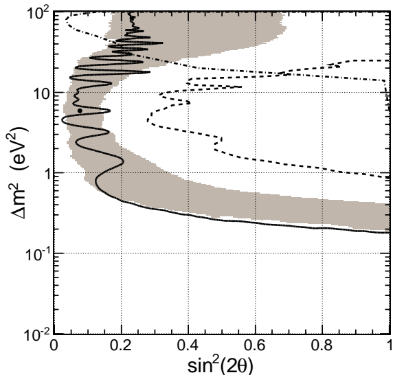
FIG. 14. 90% CL exclusion region (solid line) and best fit point for the MiniBooNE-only \bar{\nu}_\mu disappearance analysis. Also shown is the 90% CL result from the 2009 MiniBooNE disappearance analysis [8] (dashed line) and the CCFR experiment [41] (dot-dashed line). The expected 90% CL sensitivity band from fake data studies is also shown (shaded region); 1\sigma (68%) of fake data tests, where the fake data had statistical and systematic fluctuations but no oscillation signal, had 90% CL limit curves in this shaded region.
