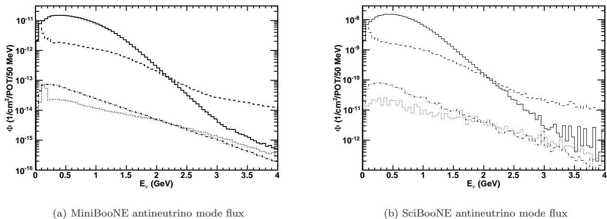
FIG. 2. The neutrino and antineutrino flux prediction as a function of true neutrino(antineutrino) energy, in antineutrino mode at the MiniBooNE and SciBooNE detectors. The \bar{\nu}_\mu flux is represented by the solid line, the \nu_\mu flux is represented by the dashed line, the \bar{\nu}_e flux is represented by the dot-dashed line, and the \nu_e flux is represented by the dotted line.
