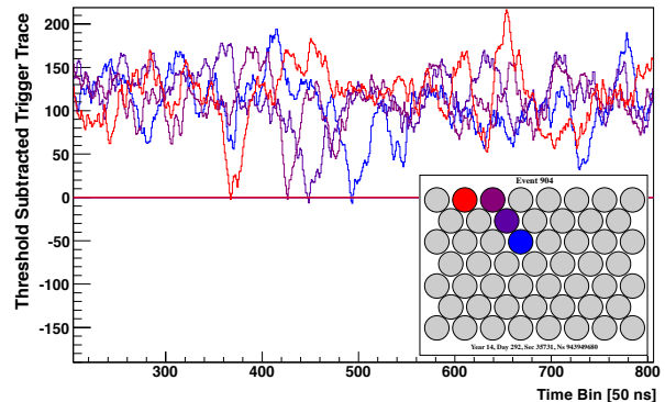
FIG. 2. (Color Online) One of the candidate 4-pixel events found in the data exhibiting topology which is consistent with expectations from an EAS.
