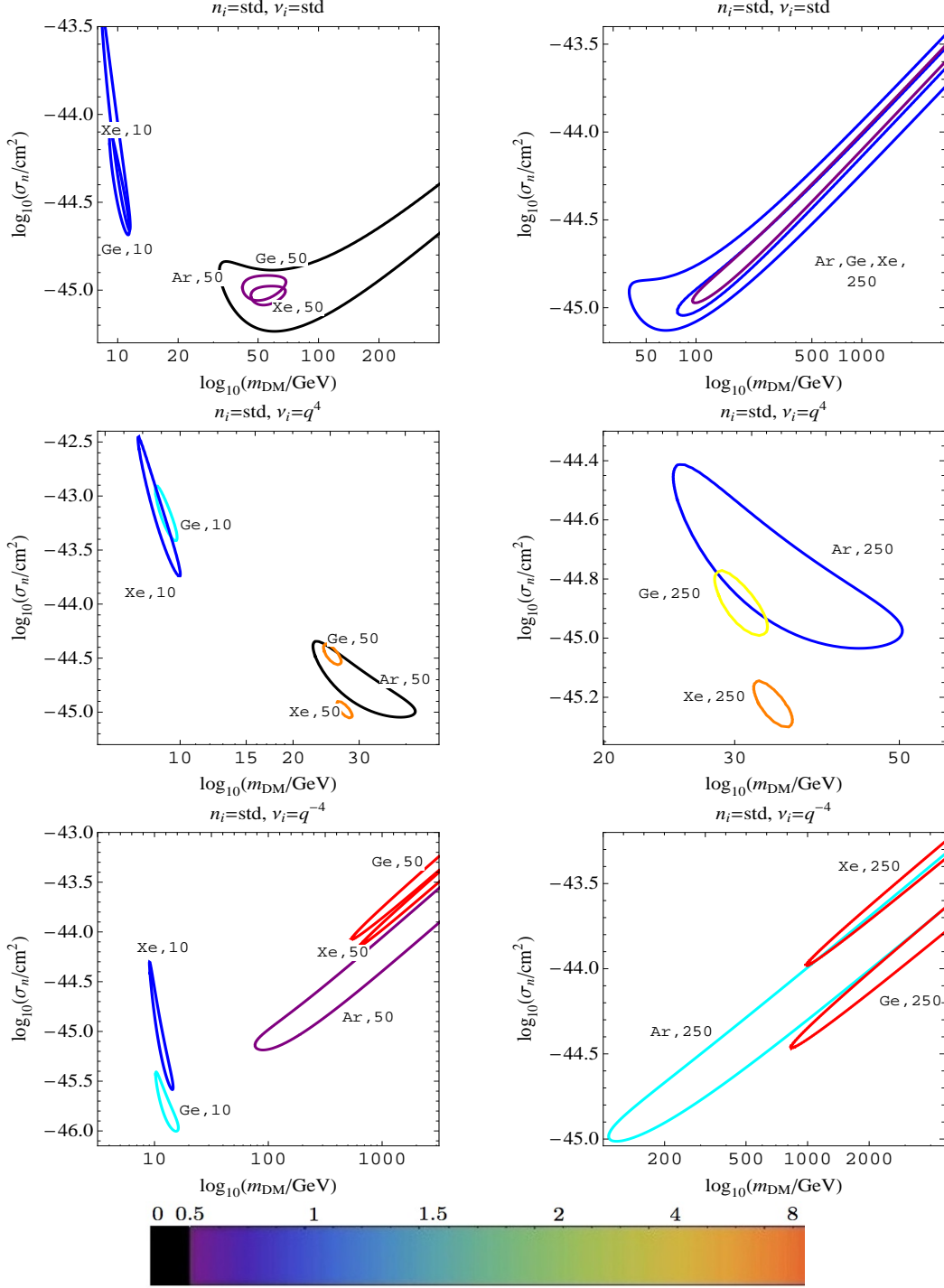
Figure 1. 95% CLCs for a 10, 50, and 250 GeV particle interacting through an n_i = standard operator with equal exposures, such that there are 300 events on a germanium target and more (fewer) on a xenon (argon) target. Comparisons are made to \nu_i = standard, q^4 , and q^{-4} operators. The colors represent the value of \tilde{L}_{\min}/\text{d.o.f.} The standard interaction can be distinguished from the q^{\pm 4} operators via both CLC overlap and the values of \tilde{L}_{\min}/\text{d.o.f.} As can be seen in Fig. (10) in the appendix, \tilde{L}_{\min}/\text{d.o.f.} is less powerful for distinguishing n_i = standard from \nu_i = q^{\pm 2} , though overlap remains robust.
