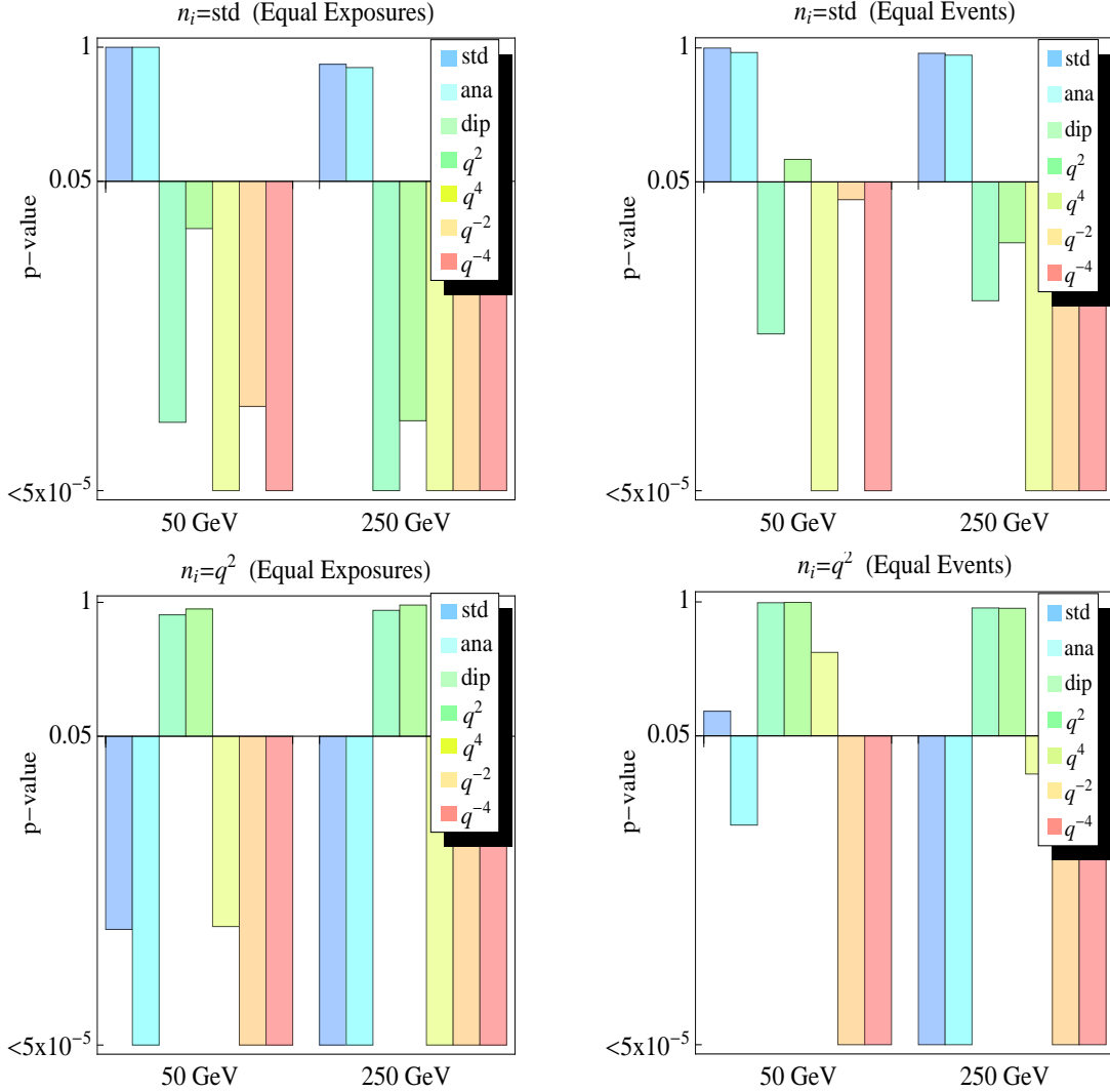
Figure 8. The p-values of trial operators for n_i = \text{standard} and q^2 operators for candidate masses of 50 and 250 GeV. We display the equal exposure and equal event bar charts side by side to underscore the robustness of the discrimination. For the visual purpose, the plot is normalized so that each bar starts at 5% significance level.
