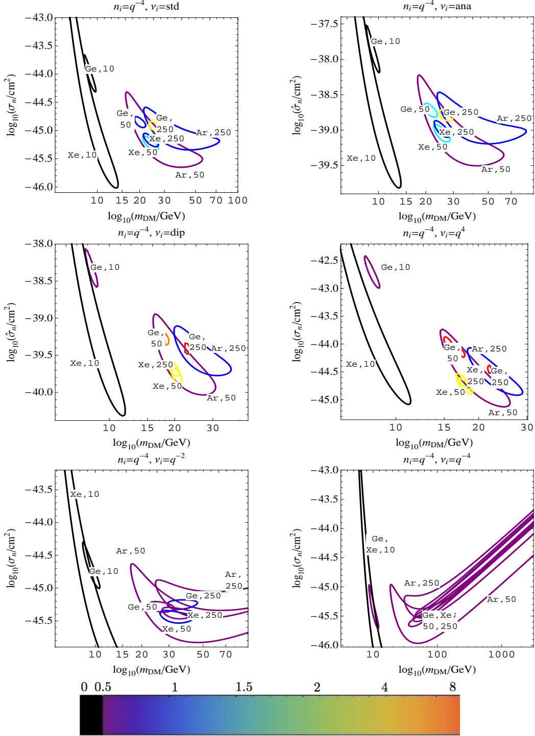
Figure 14. 95% CLCs for a 10, 50, and 250 GeV particle interacting through an n_i = q^{-4} operator. Comparisons are made to \nu_i = \text{standard, anapole, dipole, } q^4, q^{-2}, \text{ and } q^{-4} operators. The colors represent the value of \tilde{L}_{\text{min}} / \text{d.o.f.} As described above, cyan and lighter colors correspond to 95% or worse disagreement with the data.
