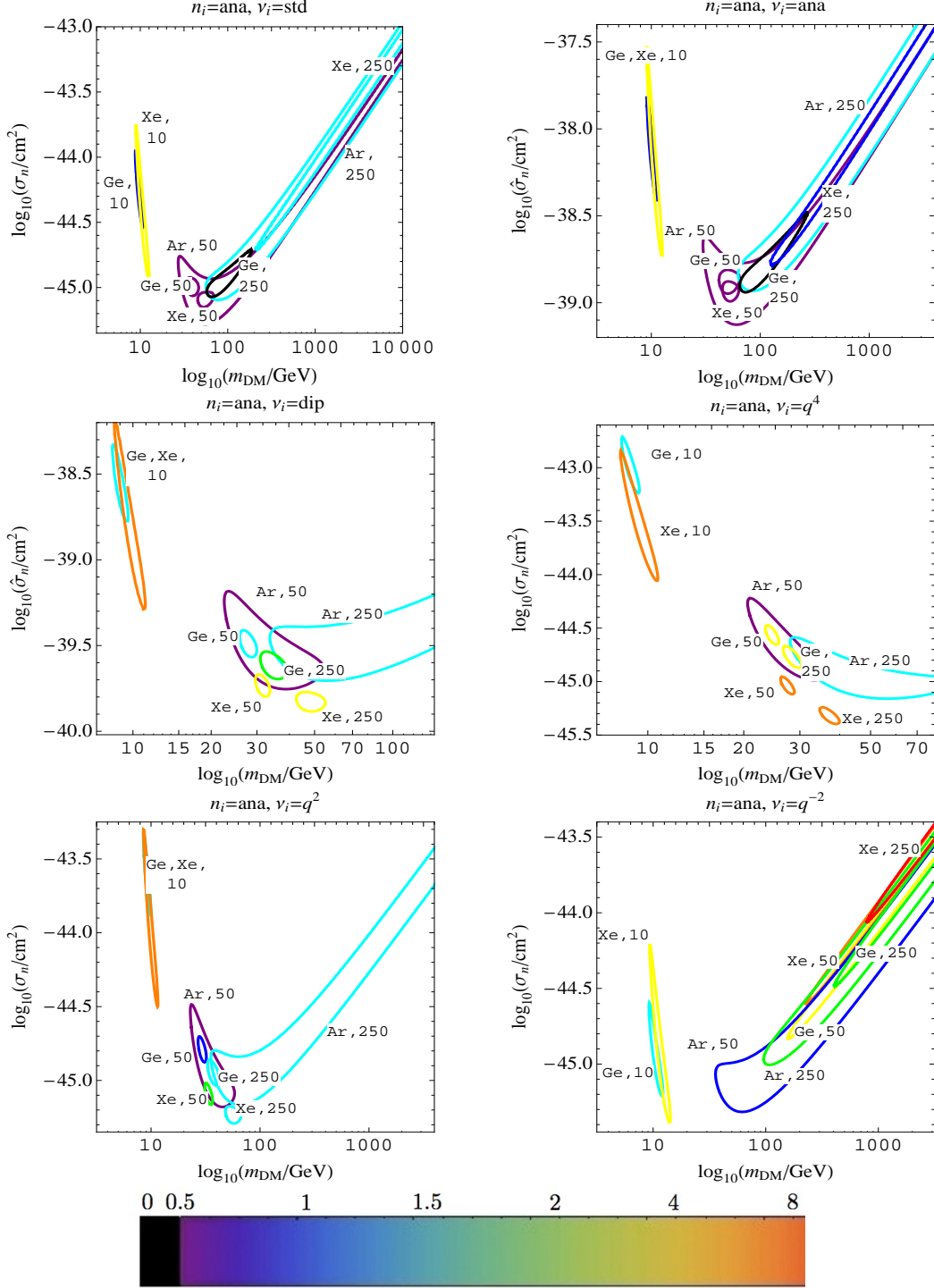
Figure 11. 95% CLCs for a 10, 50, and 250 GeV particle interacting through an n_i = \text{anapole} moment operator. Comparisons are made to \nu_i = \text{standard} , \text{anapole} , \text{dipole} , q^4 , q^2 , and q^{-2} operators. The colors represent the value of \tilde{L}_{\text{min}}/\text{d.o.f.} As described above, cyan and lighter colors correspond to 95% or worse disagreement with the data.
