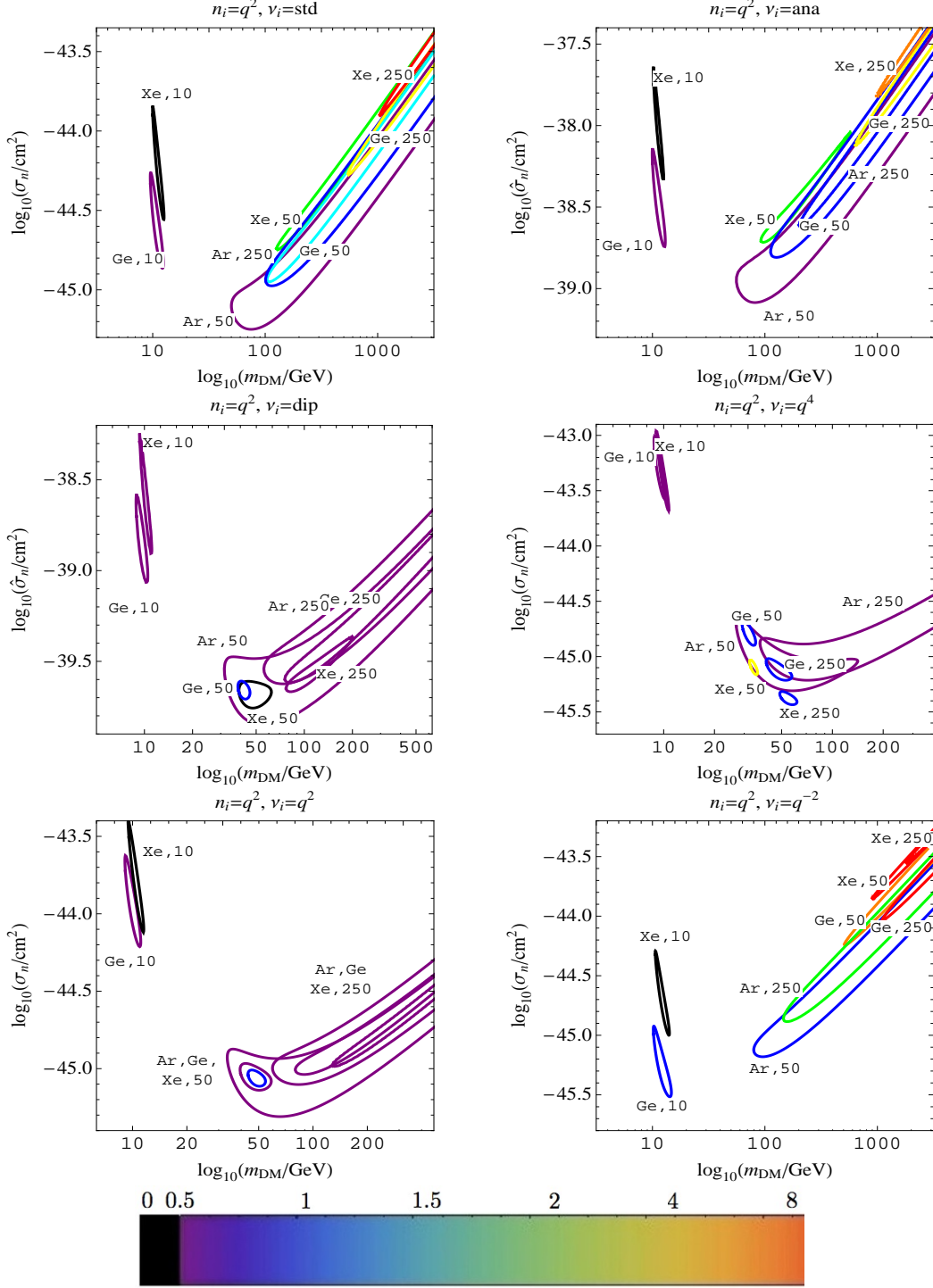
Figure 13. 95% CLCs for a 10, 50, and 250 GeV particle interacting through an n_i = q^2 operator. Comparisons are made to \nu_i = standard, anapole, dipole, q^4 , q^2 , and q^{-2} operators. The colors represent the value of \tilde{L}_{\text{min}}/\text{d.o.f.} As described above, cyan and lighter colors correspond to 95% or worse disagreement with the data.
