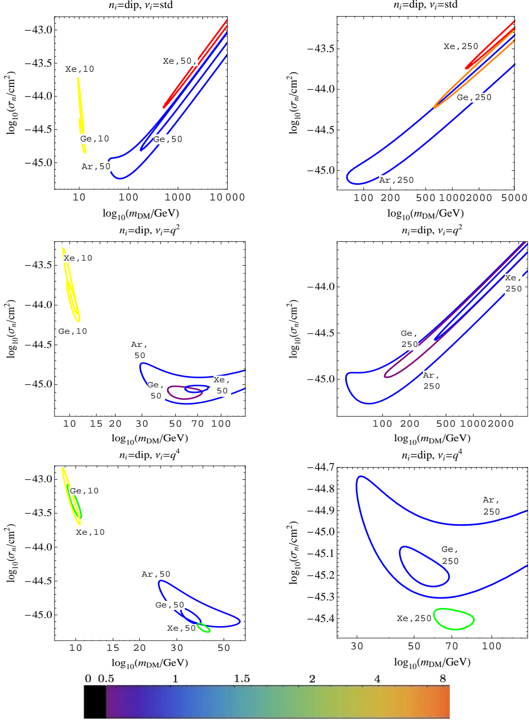
Figure 2. 95% CLCs for a 10, 50, and 250 GeV particle interacting through an n_i = \text{dipole} operator with equal exposures. Comparisons are made to \nu_i = \text{standard}, q^2, and q^4 operators. The colors represent the value of \tilde{L}_{\text{min}} / \text{d.o.f.} The dipole moment operator is dominated by a term proportional to q^2 , and is indistinguishable from this q^2 operator. The dipole interaction can be distinguished from the q^4 and standard operators via CLC overlap, which is largely powered by the statistics of the xenon target. As can be seen in Fig. (12) in the appendix, overlap remains powerful for distinguishing n_i = \text{dipole} from other operators.
