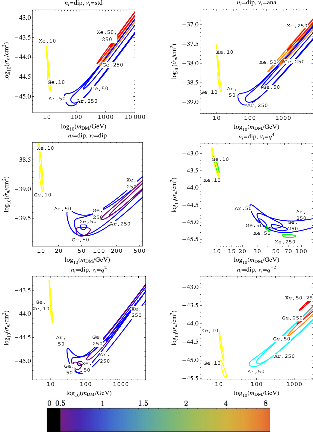
Figure 12. 95% CLCs for a 10, 50, and 250 GeV particle interacting through an n_i = \text{dipole} moment operator. Comparisons are made to \nu_i = \text{standard} , \nu_i = \text{anapole} , \nu_i = \text{dipole} , \nu_i = q^4 , \nu_i = q^2 , and \nu_i = q^{-2} operators. The colors represent the value of \tilde{L}_{\text{min}}/\text{d.o.f.} As described above, cyan and lighter colors correspond to 95% or worse disagreement with the data.
