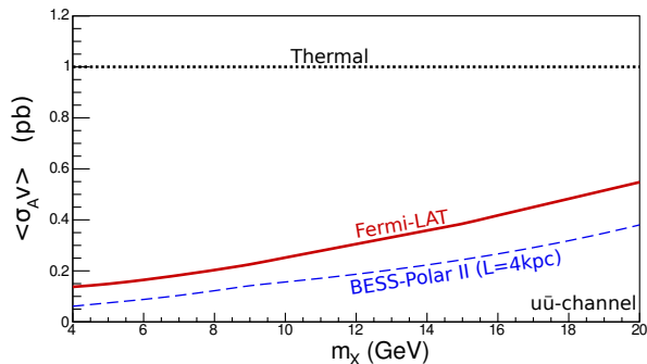
FIG. 1. 95% CL exclusion bound (see text) from Fermi in the (m_\chi, \langle\sigma_{AV}\rangle) plane, assuming dark matter annihilation to u\bar{u} . The results for annihilation to the d\bar{d} channel are visually identical. Also shown is the exclusion contour from BESS-Polar II for the same channel (assuming a diffusion halo size of 4 kpc). The dotted line indicates 1 pb, which is approximately the total annihilation cross-section at freeze-out for dark matter produced thermally in the early universe.
