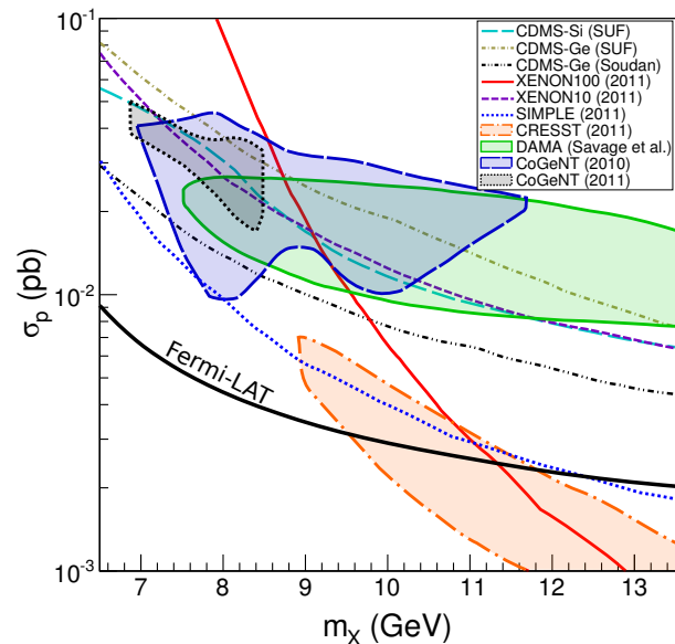
FIG. 2. Favored regions and exclusion contours in the (m_X, \sigma_p) plane for IVDM with f_n/f_p = -0.7 . The solid black line is the bound from this analysis at 95% CL, assuming central values for the satellite density profile.
