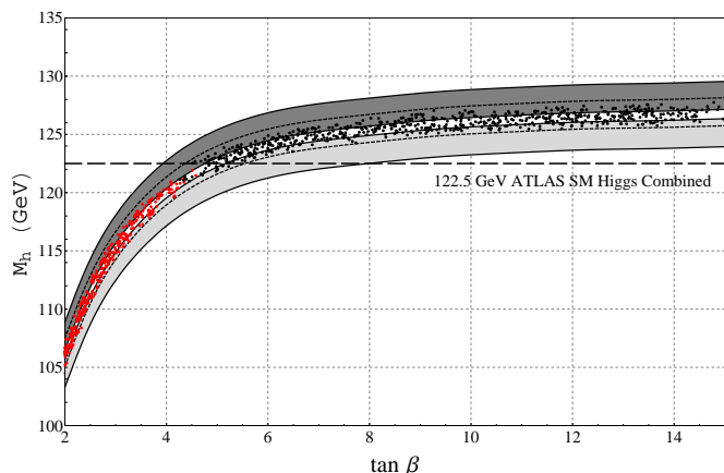
FIG. 1: The prediction for the Higgs mass at two-loops for realistic string/ M theory vacua defined in the text, as a function of \tan \beta for three different values of the gravitino mass m_{3/2} , and varying the theoretical and experimental inputs as described below. SPheno 2.2.3 was used to evolve GUT scale parameters to M_{SUSY} . For precise numbers and more details, see section IV. The central band within the dashed curves for which scatter points are plotted corresponds to m_{3/2} = 50 \text{ TeV} . This band includes the total uncertainty in the Higgs mass arising from the variation of three theoretical inputs at the unification scale, and from those in the top mass m_t and the SU(3) gauge coupling \alpha_s within the allowed uncertainties. The innermost (white) band bounded by solid curves includes the uncertainty in the Higgs mass for m_{3/2} = 50 \text{ TeV} only from theoretical inputs. The upper (dark gray) band bounded by solid curves corresponds to the total uncertainty in the Higgs mass for m_{3/2} = 100 \text{ TeV} while the lower (light gray) band bounded by solid curves corresponds to that for m_{3/2} = 25 \text{ TeV} . For m_{3/2} = 50 \text{ TeV} , the red scatter points (with \tan \beta less than about 4.5) and blue scatter points (with \tan \beta greater than about 4.5) correspond to “Large” \mu and “Small” \mu respectively, as described in section II and section IV. The lower bound of the higgs mass is from [44]. We assume the currently almost excluded regime 117.5-118.5 GeV will soon be fully excluded.
