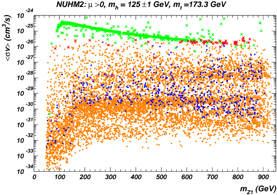
Figure 17: Thermally averaged neutralino annihilation cross section times relative velocity \langle \sigma v \rangle vs. m_{\tilde{z}_1} from scan over NUHM2 points restricted by m_h = 125 \pm 1 GeV. The color coding is the same as in Fig. 16.
