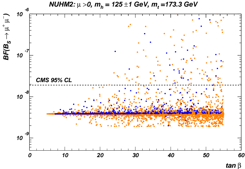
Figure 13: Value of BF(B_s \rightarrow \mu^+ \mu^-) vs. \tan \beta from scan over NUHM2 parameters restricted by m_h = 125 \pm 1 GeV. Blue points denote m_0 < 5 TeV, while orange points allow m_0 values up to 20 TeV. The dashed line represent the 95% CL upper limit from the CMS [39].
