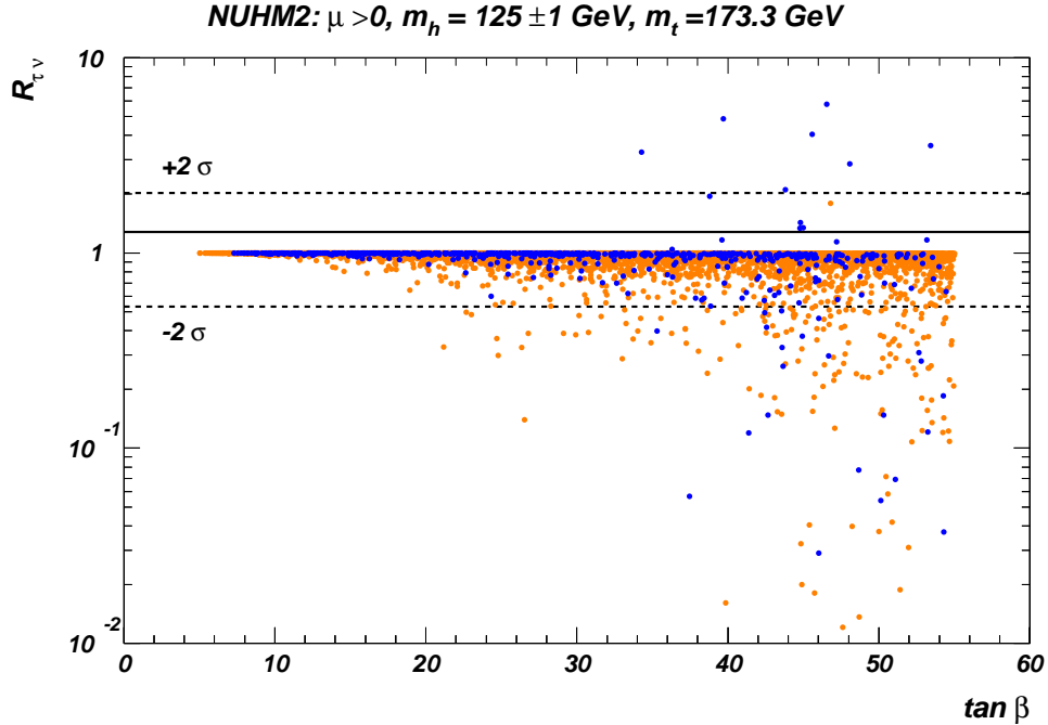
Figure 14: Value of R_{\tau\nu} \equiv BF(B_u \rightarrow \tau^+\nu_\tau)_{MSSM}/BF(B_u \rightarrow \tau^+\nu_\tau)_{SM} vs. \tan\beta from scan over NUHM2 parameters restricted by m_h = 125 \pm 1 GeV. Blue points denote m_0 < 5 TeV, while orange points allow m_0 values up to 20 TeV. The solid line denotes the central experimental value, while dashed lines represent the \pm 2\sigma error bars [43].
