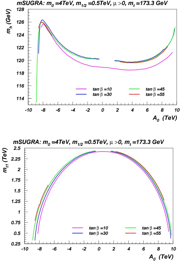
Figure 2: Plot of a) m_h vs. A_0 in the mSUGRA model for m_0 = 4 \text{ TeV} , m_{1/2} = 0.5 \text{ TeV} , \mu > 0 and various values of \tan \beta . In frame b), we show m_{\tilde{t}_1} vs. A_0 versus A_0 for the same parameter choices. Curves terminate due to the lack of EWSB or because top squark becomes tachyonic.
