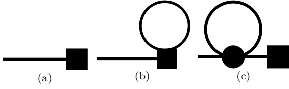
FIG. 2. SChPT diagrams contributing to the single kaon matrix elements in the denominator of B_K : (a) tree-level; (b-c) one-loop. Notation is as in Fig. 1.
