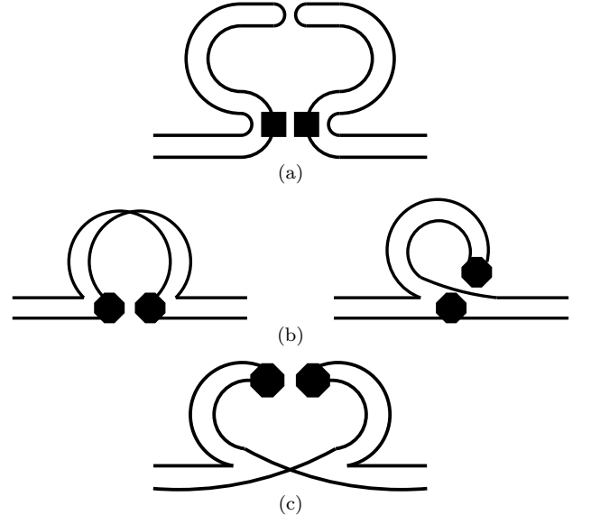
FIG. 3. Quark-line diagrams contributing to (a) Fig. 1(d), (b) Fig. 1(e), and (c) Fig. 1(f). In each case, each of the filled boxes correspond to one of the factors of \Sigma (or \Sigma^\dagger ) in the chiral operators. The square boxes arise from the double trace operators and thus have flavor \bar{S}_1 D_1 or \bar{S}_2 D_2 . The octagonal boxes arise from the single trace operators and thus have flavor \bar{S}_1 D_2 or \bar{S}_2 D_1 .
