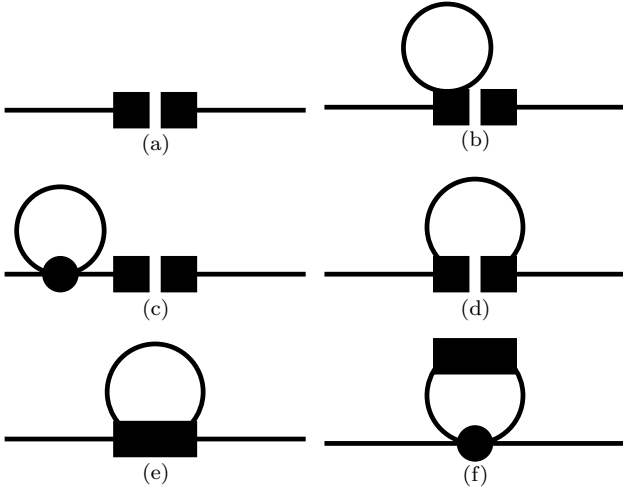
FIG. 1. SChPT diagrams contributing to the numerator of B_K : (a) tree-level; (b-f) one-loop. The double trace components of the chiral operators are represented by two square boxes, one per trace, while the single trace components are shown with one rectangular box. (It turns out that there is no contribution from a diagram of the form of (f) but with a two trace operator.) The filled circle is the full LO vertex from the SChPT Lagrangian, including \mathcal{O}(a^2) terms. For (b) and (c) we have not shown separately the diagrams in which the loop is attached to the other external kaon.
