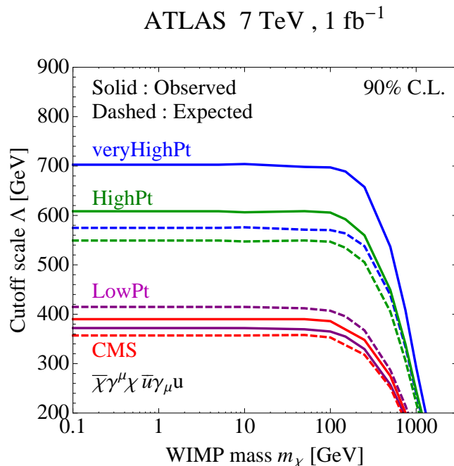
Figure 3: Limits on the suppression scale \Lambda for the vector operator, \mathcal{O}_V , where only the coupling to up quarks is considered, for the three ATLAS analyses and the analysis of CMS. In all cases the observed (expected) bound is represented by a solid (dashed) line.
