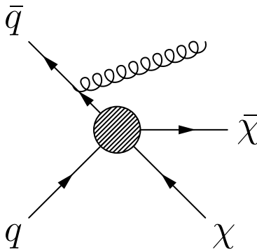
Figure 1: Dark matter production in association with a single jet in a hadron collider.
