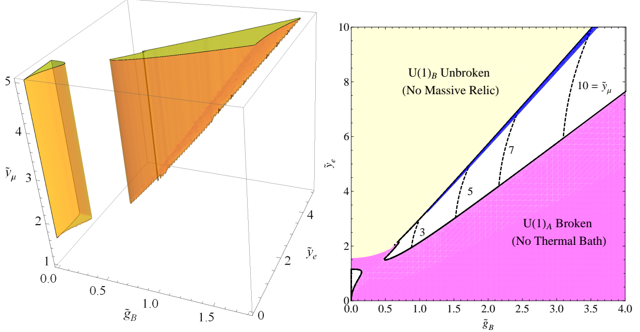
FIG. 1: Left : Allowed regions in the (\tilde{g}_B, \tilde{y}_e, \tilde{y}_\mu) parameter space of the U(1)_A \times U(1)_B model. Right : A projection of the allowed parameter space onto the (\tilde{g}_B, \tilde{y}_e) plane. The light yellow and medium magenta shaded regions are excluded for the reasons indicated. Dark matter is composed of selectrons everywhere in the viable region, except inside the dark blue band, where it is electrons. At tree-level, the mass of the dark matter particle is independent of \tilde{y}_\mu , as long as \tilde{y}_\mu is in a viable region of parameter space. Contours of minimum \tilde{y}_\mu for given values of (\tilde{g}_B, \tilde{y}_e) are shown. Regions to the right of the \tilde{y}_\mu = \text{const.} curves are not viable for \tilde{y}_\mu > \text{const.} , since the constraint m_{H_e}^2 + m_{H_\mu}^2 > 0 cannot hold, and the potential is unstable.
