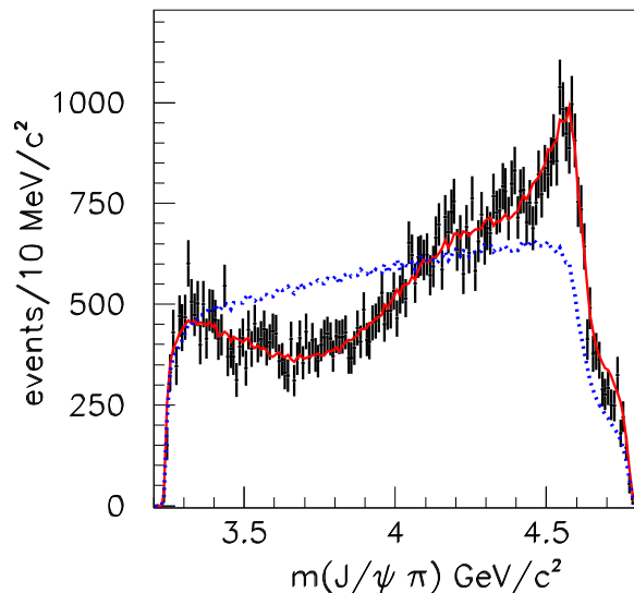
FIG. 9: Background-subtracted and efficiency-corrected J/\psi \pi mass distribution for the B \rightarrow J/\psi K\pi control sample with the superimposed curves resulting from the MC simulation described in the text. The solid curve is obtained using the total weight w obtained with L_{\max} = 5 , the dotted curve by omitting the angular-dependence factor w_L .
