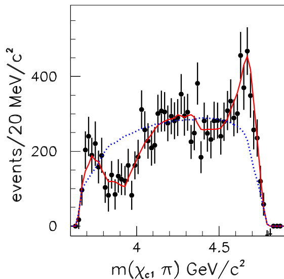
FIG. 10: Background-subtracted and efficiency-corrected \chi_{c1}\pi mass distribution from B \rightarrow \chi_{c1}K\pi . The solid curve results from the MC simulation described in the text, which uses of the moments from the same channels. The dotted curve shows the result of the simulation when the w_L weight is removed.
