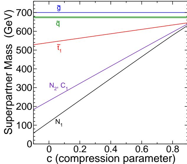
FIG. 1: The masses of the most relevant superpartners for the models of class I defined in section III, as a function of the compression parameter c , for fixed M_{\tilde{g}} = 700 GeV. The case c = 0 corresponds to an mSUGRA-like model.
