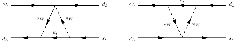
FIG. 8: Diagrams that yield the chiral logarithmically-enhanced three-site model corrections to \Delta S = 2 processes in the effective theory, Eq. (36), including the flavor non-universal corrections to \epsilon_L shown in Eq. (71), . Here \pi_W are the 't-Hooft-Feynman gauge unphysical Goldstone Bosons eaten by the W boson. As discussed in the text, though enhanced by \log(M^2/M_W^2) , all new three-site contributions are even more deeply suppressed by m_q^2/M^2 .
