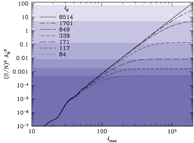
FIG. 11. The square of the SNR per unit bispectrum amplitude ( A_B ) for various damping scales \ell_d . The shaded regions indicate the prediction of our scaling formula in Eq. (96) and match the asymptotic high \ell \gg \ell_d saturation point for each case.
