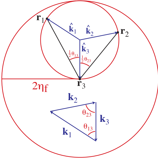
FIG. 13. Relationship between bispectrum triangle shapes and resonances in the three-point real space correlation function. As d \rightarrow 0 each set of self-similar bispectrum triangles determined by (\mathbf{k}_1, \mathbf{k}_2, \mathbf{k}_3)s , where s is some scale factor, causes a resonance at (\mathbf{r}_1, \mathbf{r}_2, \mathbf{r}_3) and its mirror image. As the overall size of the triangle s \rightarrow \infty this resonance becomes sharper and sharper in real space but remain associated with separations \mathcal{O}(\eta_f) . Flat triangles are responsible for the largest scale resonance for \mathbf{r}_1 - \mathbf{r}_3 = \mathbf{r}_2 - \mathbf{r}_3 = 2\eta_f .
