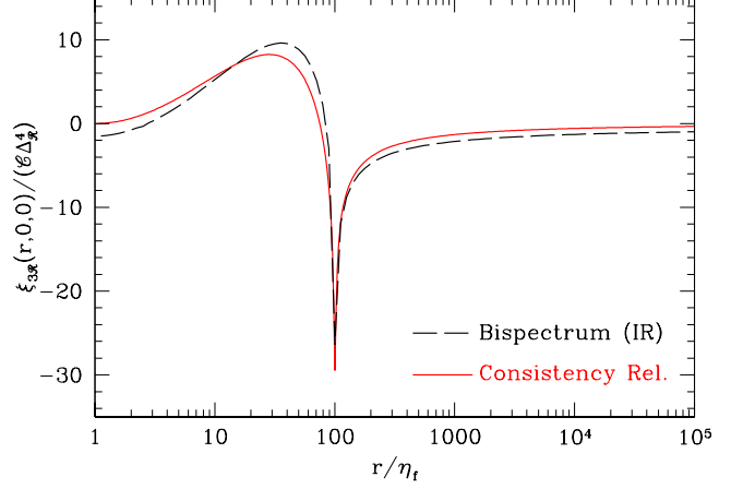
FIG. 16. The contribution to the real space three-point correlation function from the infra-red terms (the second two terms) in Eq. (A25) (dashed black curve) and the consistency relation of Eq. (A35) (red, solid). We take x_d = 100 with an infrared cutoff at k_{\min} = 0.001/\eta_f .
