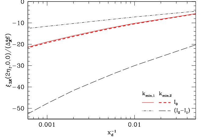
FIG. 15. Behavior of the various contributions to the real space three-point correlation function \xi_{3\mathcal{R}}(r, 0, 0) in Eq. (A25) at the point r = 2\eta_f as a function ultraviolet cutoff x_d . The dependence on the infrared cutoff is also demonstrated. Here k_{\min,1} = 0.1/\eta_f , while k_{\min,2} = 0.001/\eta_f .
