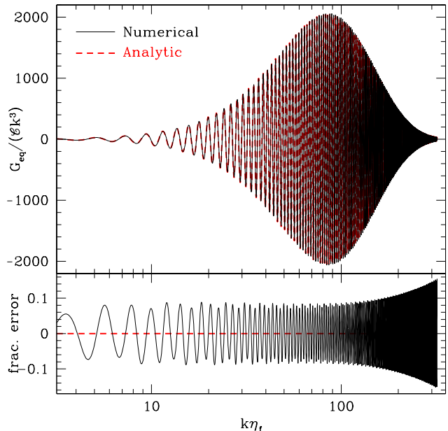
FIG. 4. Equilateral bispectrum computed using the analytic approximation in Eq. (48) (red dashed) compared with a full numerical evaluation of the integral in Eq. (45) for a small amplitude c = 10^{-5} (or \mathcal{C} \ll 1 ). The lower panel shows the difference between the curves, expressed as a fraction of the envelope of the analytic approximation in Eq. (63).
