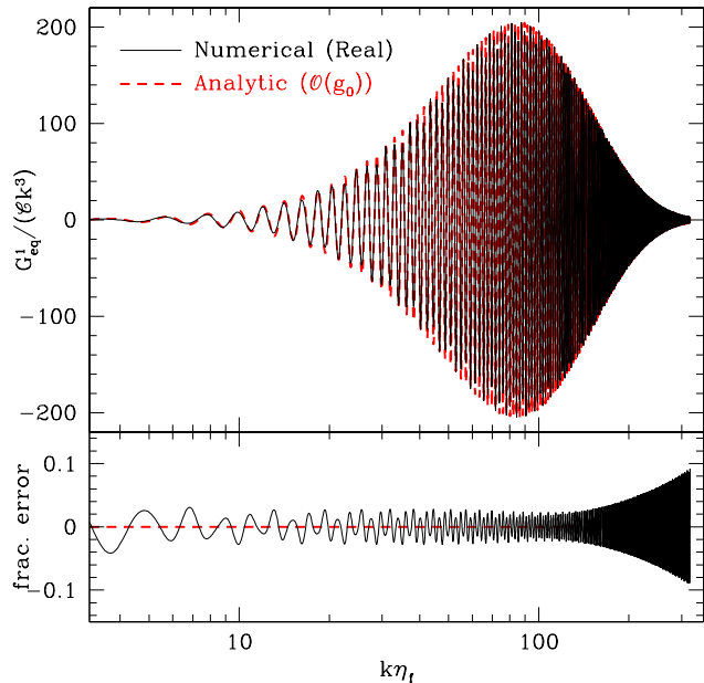
FIG. 17. First order corrections to the equilateral bispectrum computed using the analytic approximation Eq. (B11) and (B14) compared with the numerical evaluation of the second term in Eq. (B5) for a step with height c = 10^{-5} and width d = 0.001 . The lower panel here shows the fractional error of the full bispectrum, once this first order correction is taken into account. We take \pi g_0/2 = 0.1 for this plot.
