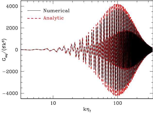
FIG. 5. Equilateral bispectrum computed using the analytic approximation in Eq. (48) (red dashed) compared with a full numerical evaluation of the integral in Eq. (45) for a large amplitude c \approx \epsilon_0/6 (or \mathcal{C}_0 = 1, \mathcal{C} = 2/3 ). Here the location, amplitude and damping scale of the feature have been nonlinearly scaled according to Eq. (33) and Eq. (35).
