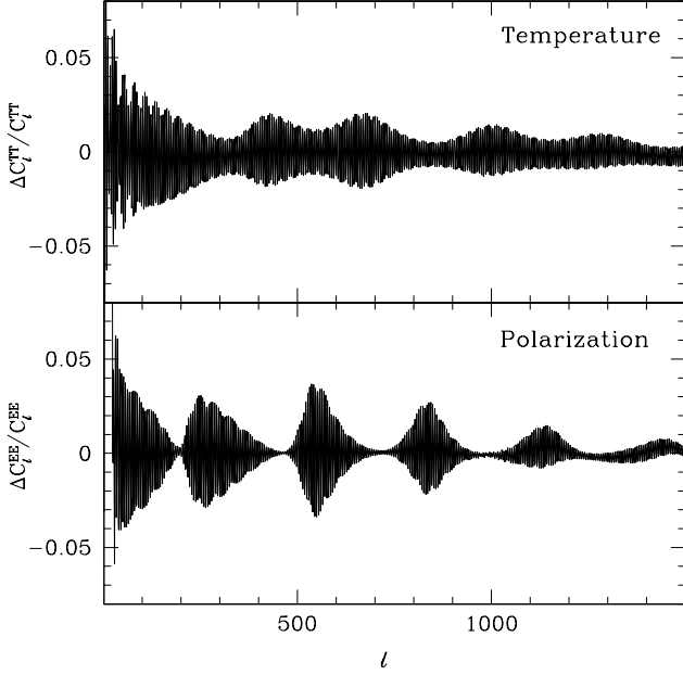
FIG. 9. Fractional angular power spectrum differences between the maximum likelihood sharp-step model ( A_C = 0.11, \eta_f = 8.163 Gpc) and pure power law model ( A_C = 0 ). The WMAP data prefer a few percent oscillation in the temperature power spectrum (top panel) around the first acoustic peak by 2\Delta \ln L = 11.6 . This model predicts matching E -polarization power spectrum oscillations (bottom panel) modulated by an orthogonal acoustic phase.
