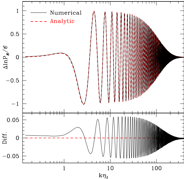
FIG. 2. Same as Fig. 1 but using a smaller value of the step width. Here we take d = 10^{-3} , or x_d \approx 43 .
