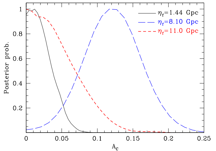
FIG. 8. Posterior probability distribution of the oscillation amplitude A_C in the angular power spectrum for representative value of \eta_f = 1.44, 8.1 and 11 Gpc. The constraint weakens as \eta_f approaches the horizon for typical cases. For \eta_f \sim 8.1 Gpc and other specific values, the peak of the posterior is shifted to A_C \sim 0.1 with comparable distribution width.
