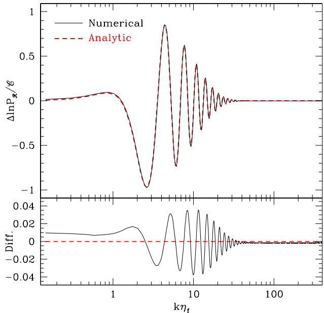
FIG. 1. Initial curvature power spectrum evaluated numerically (in black solid curves) compared with using the approximation in Eq. (32) (in dashed red curves) for a small amplitude step c = 10^{-5} \ll \epsilon_0/6 (or C \ll 1 ), where the approximation is expected to work, and a step width, d = 10^{-2} , or x_d \approx 4.3 . The lower panel shows the difference between the two curves, numerical - analytic. The remaining parameters used in both models are shown in Table I.
