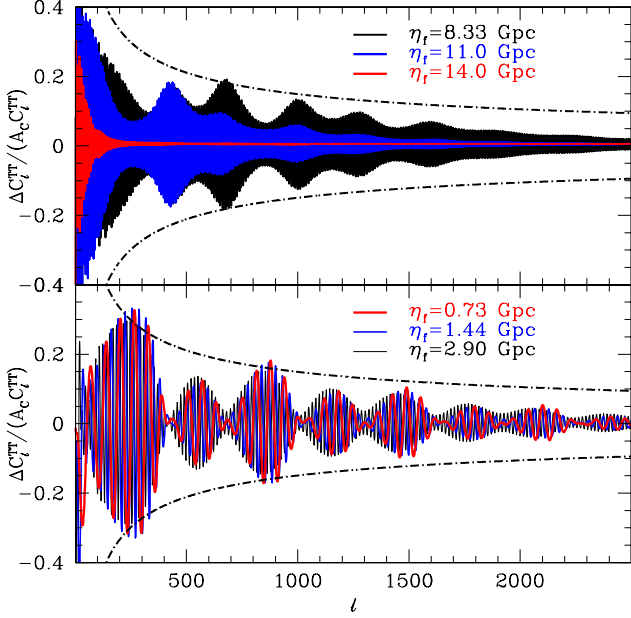
FIG. 7. Fractional difference of the temperature power spectrum (relative to a model with c = 0 ) of a model with c = 10^{-5} and d = 10^{-5} and different step positions. Gravitational lensing is taken into account in these examples. Note that as D/\eta_f \rightarrow 1 (in the upper panel), the nodes shift, and the shape changes significantly. In black dot-dashed lines we show the expected \ell^{-1/2} envelope from Eq. (70).
