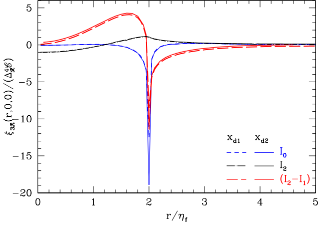
FIG. 14. Contribution to the real space three-point correlation function from the three terms in Eq. (A25). The thick dashed curves were computed for damping scale x_d = x_{d1} = 200 with an infrared cutoff at k_{\min} = 0.1/\eta_f , while the corresponding thin solid curves were calculated with x_{d2} = 1000 .
