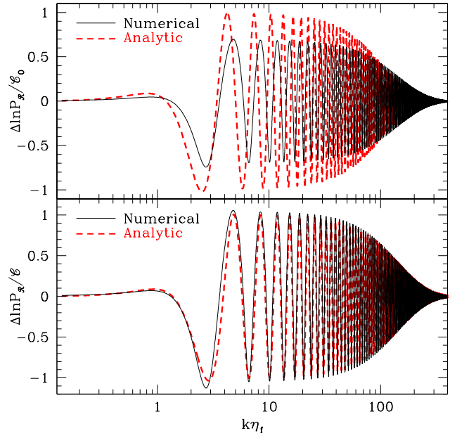
FIG. 3. Initial curvature power spectrum evaluated numerically (in solid black curves) compared with the approximation in Eq. (32) (in dashed red curves) for a large amplitude c = \epsilon_0/6 (or \mathcal{C}_0 = 1 , \mathcal{C} = 2/3 ), where the linear expansion is violated by order unity terms. Using the leading order expressions for the step location, oscillation amplitude and damping \eta_f , \mathcal{C} = \mathcal{C}_0 and x_d (upper panel) leads to phase and amplitude errors that are largely corrected by non-linearly rescaling these parameters using Eqs. (33) and (35) (lower panel).
