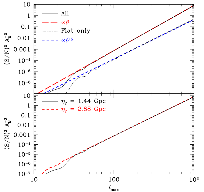
FIG. 10. The square of the SNR per unit bispectrum amplitude ( A_B ) for \ell_d = 8514 for all triangles, and for flat configurations only. We also plot the scaling relations from §VIC. In the lower panel, we demonstrate that changing \eta_f while fixing A_B and \ell_d leaves the SNR fixed at high \ell .
