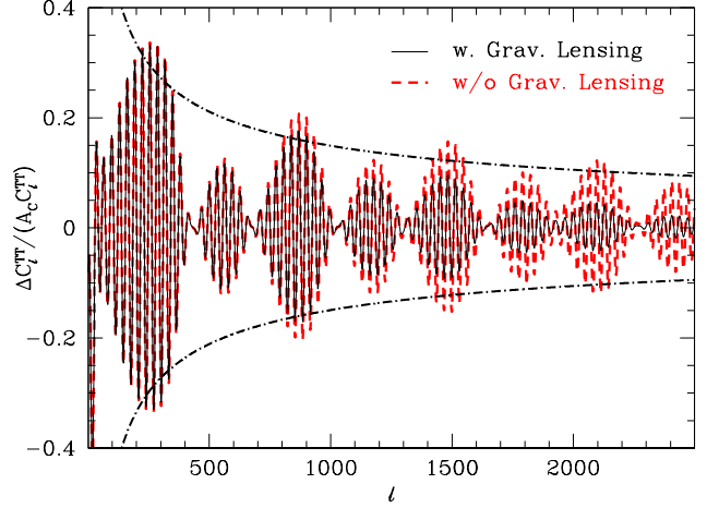
FIG. 6. Fractional difference of the temperature power spectrum of a model with \eta_f = 1.44 Gpc, c = 10^{-5} and d = 10^{-5} , relative to a model with c = 0 per unit power spectrum feature amplitude A_C (see Eq. 69). The case without gravitational lensing is shown in red dashed lines, and when gravitational lensing is taken into account is shown in black solid lines. In black dot-dashed lines we show the expected \ell^{-1/2} envelope from Eq. (70).
