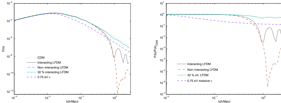
FIG. 1: Power spectra (left), and power compared to CDM (right) for CDM, LFDM (with different fractions, interacting and free-streaming) and a 0.75 eV freestreaming neutrino for z_{tach} = 50,000
