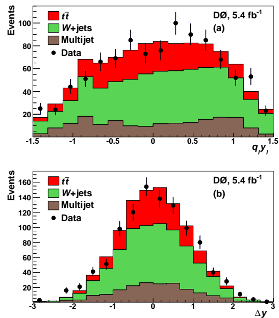
FIG. 5. The reconstructed (a) q_l y_l and (b) \Delta y in events with no b -tagged jets. In (b), the bin widths correspond to about half of the detector resolution in \Delta y .
