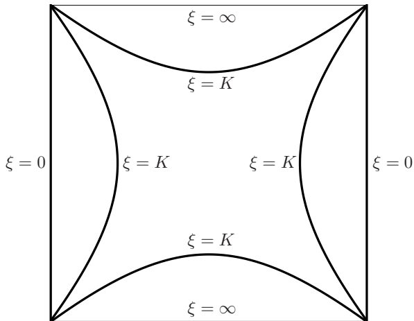
FIG. 5: Penrose diagram of the solution with p = -1 in the case of \Lambda > 0 .
