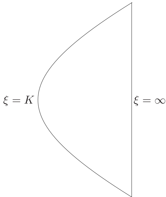
FIG. 1: Penrose diagram of the bubble solution
