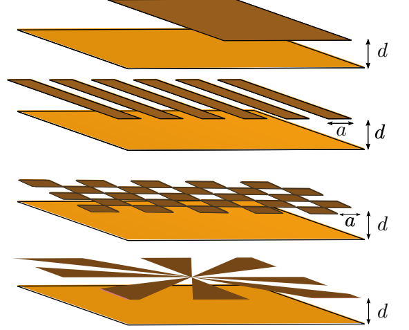
Figure 1: Self-complementary geometries, each facing an infinite plate.
