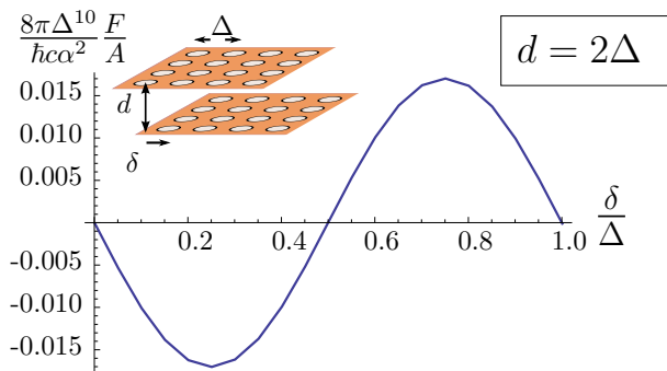
Figure 2: The lateral force per area as a function of the displacement \delta . For this graph, we chose d = 2\Delta . The point \delta = 0 is an stable equilibrium of this configuration.
